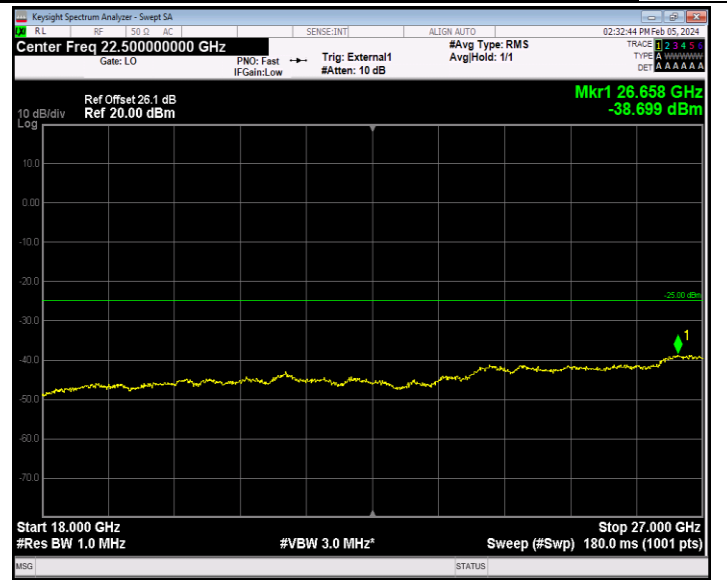
Band41_20MHz_QPSK_41140_1RB#0_18000~27000_18000~27
