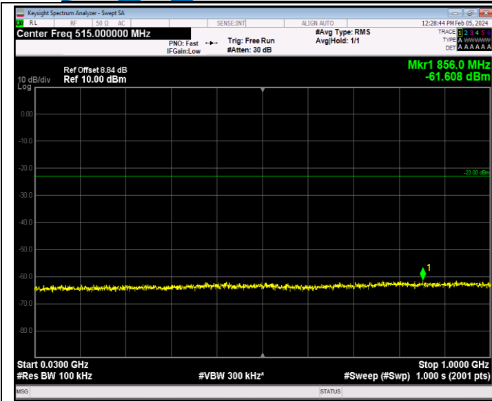
Band66_20MHz_QPSK_132322_1RB#0_30~1000_30~1000
