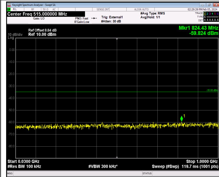
Band41_20MHz_16QAM_40140_1RB#0_30~1000_30~1000
