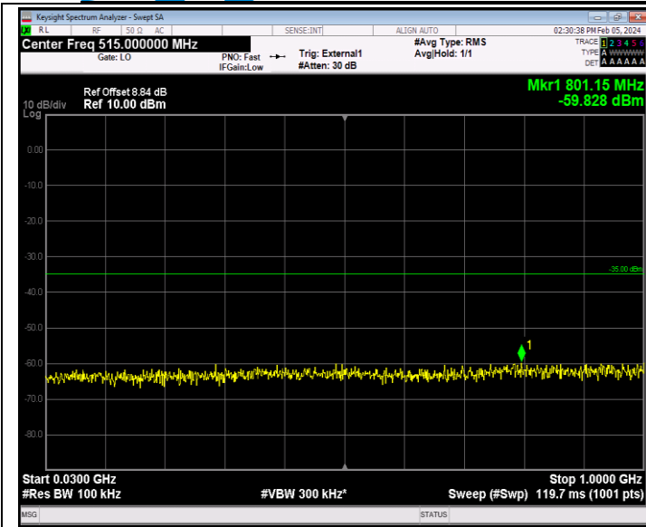
Band41_20MHz_QPSK_40640_1RB#0_30~1000_30~1000
