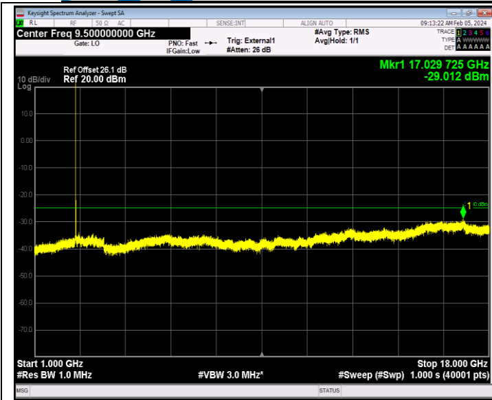
Band41_5MHz_16QAM_40065_1RB#0_1000~18000_1000~1800 0
