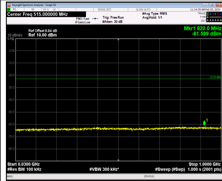
Band66_1.4MHz_16QAM_132665_1RB#0_30~1000_30~1000
