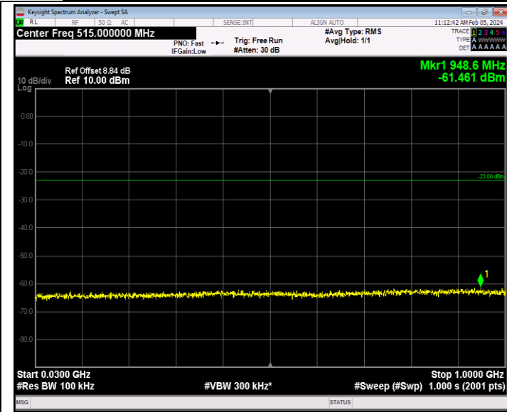
Band66_1.4MHz_64QAM_131979_1RB#0_30~1000_30~1000
