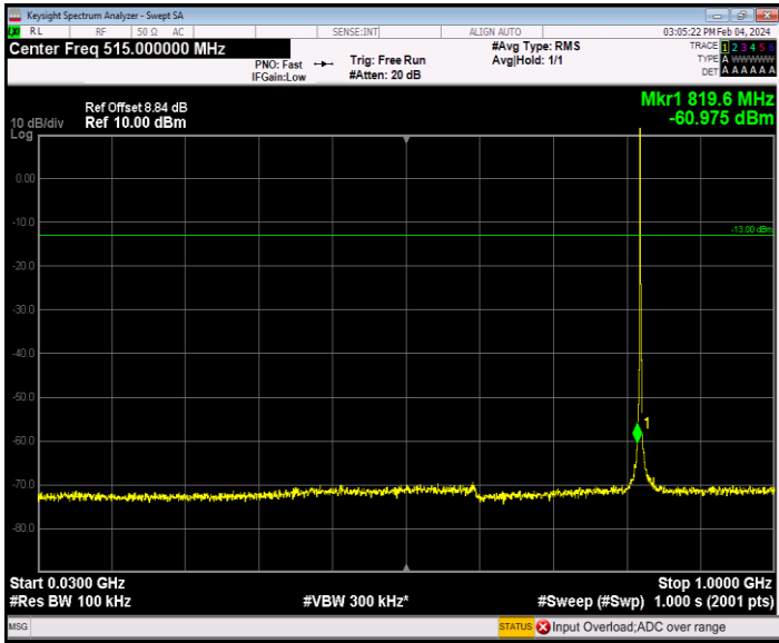
Band26_1.4MHz_64QAM_26783_1RB#0_30~1000_30~1000
