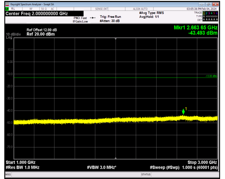
Band26_1.4MHz_64QAM_26783_1RB#0_1000~3000_1000~300 0
