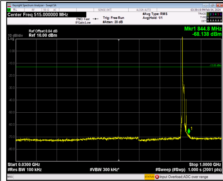
Band26_10MHz_16QAM_26740_1RB#0_30~1000_30~1000
