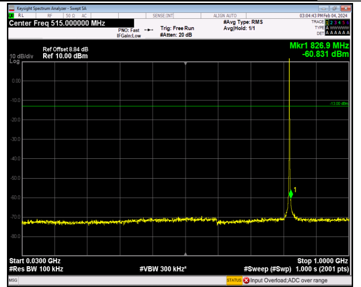
Band26_1.4MHz_16QAM_26783_1RB#0_30~1000_30~1000
