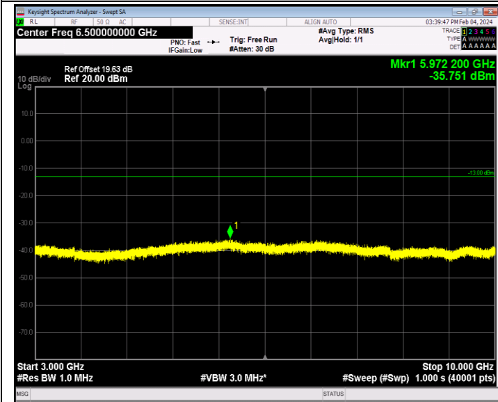
Band26_10MHz_16QAM_26740_1RB#0_3000~10000_3000~100
