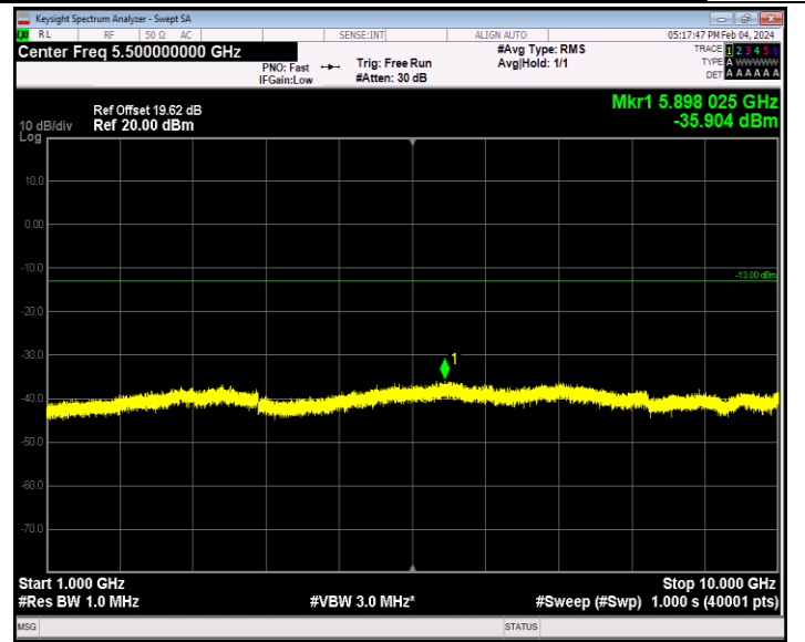
Band26_15MHz_16QAM_26915_1RB#0_1000~10000_1000~1000 00
