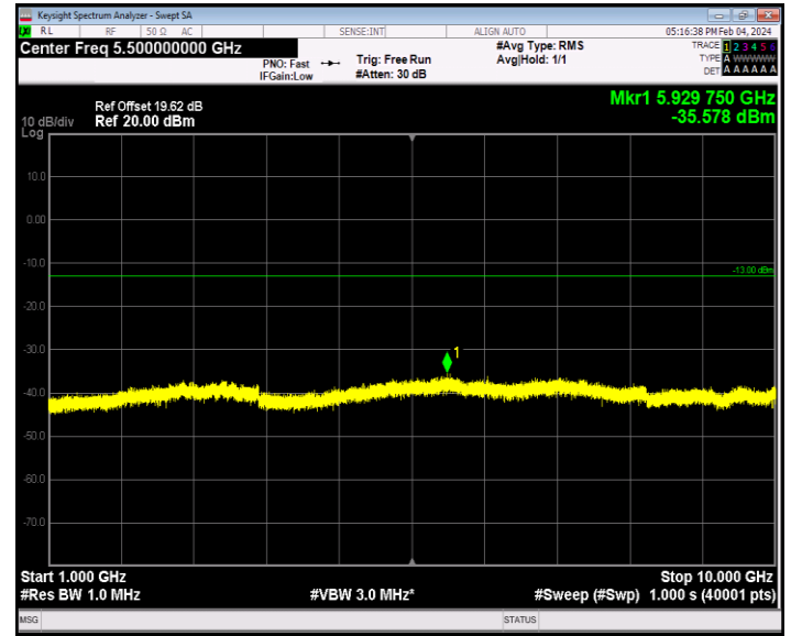
Band26_15MHz_16QAM_26865_1RB#0_1000~10000_1000~1000 00
