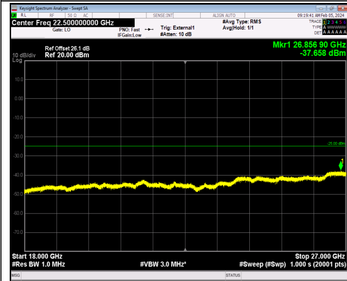
Band41_5MHz_QPSK_41215_1RB#0_18000~27000_18000~270
