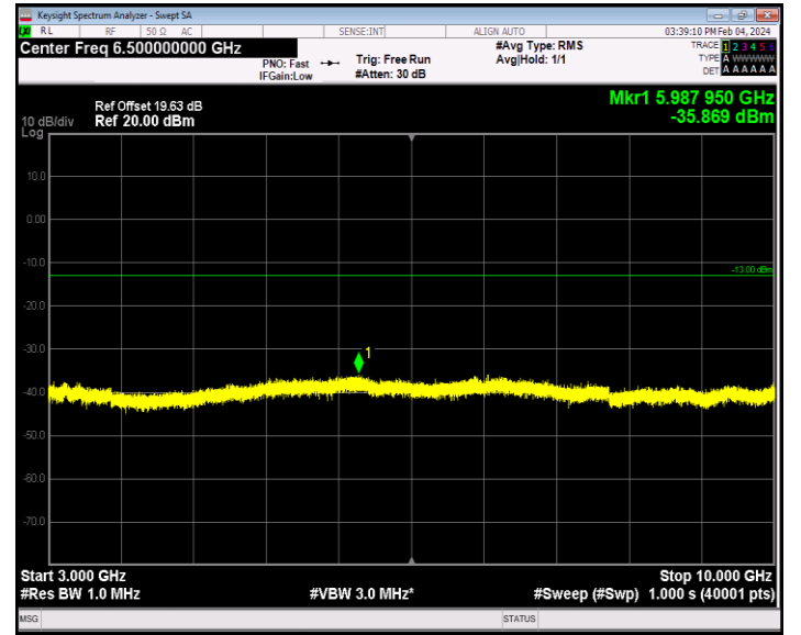
Band26_10MHz_QPSK_26740_1RB#0_3000~10000_3000~10000
