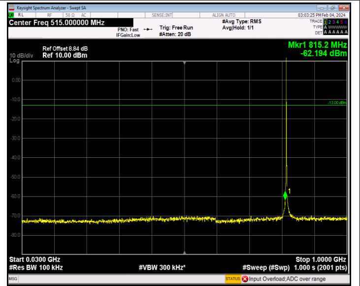
Band26_1.4MHz_64QAM_26740_1RB#0_30~1000_30~1000
