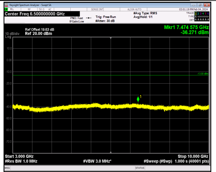
Band26_1.4MHz_16QAM_26697_1RB#0_3000~10000_3000~10 000
