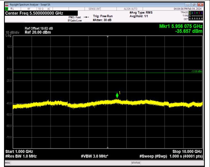
Band26_1.4MHz_16QAM_26915_1RB#0_1000~10000_1000~10000
