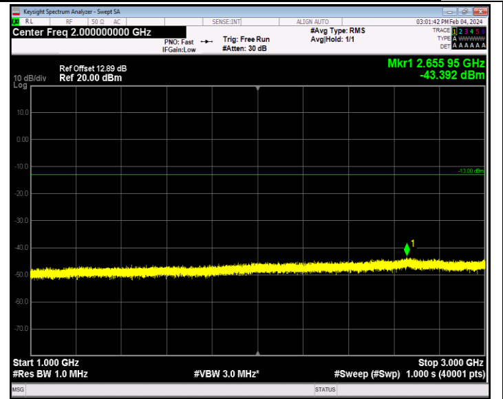
Band26_1.4MHz_64QAM_26697_1RB#0_1000~3000_1000~3000 0
