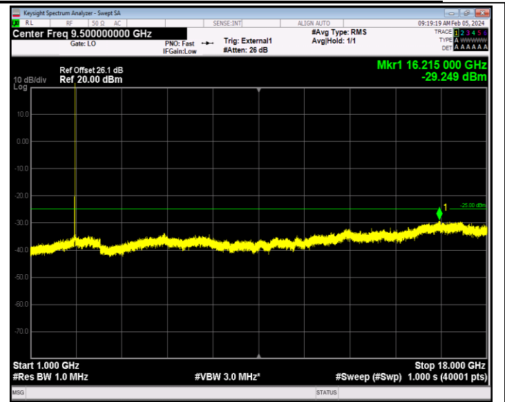
Band41_5MHz_QPSK_41215_1RB#0_1000~18000_1000~18000
