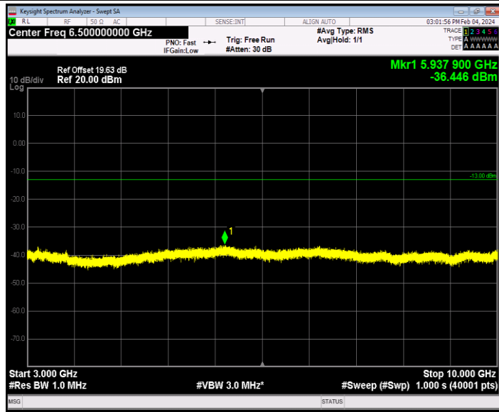
Band26_1.4MHz_64QAM_26697_1RB#0_3000~10000_3000~10000 000
