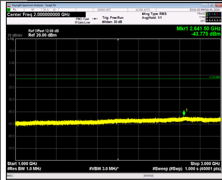
Band26_1.4MHz_16QAM_26697_1RB#0_1000~3000_1000~300 0
