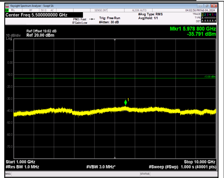
Band26_1.4MHz_16QAM_26797_1RB#0_1000~10000_1000~10000
