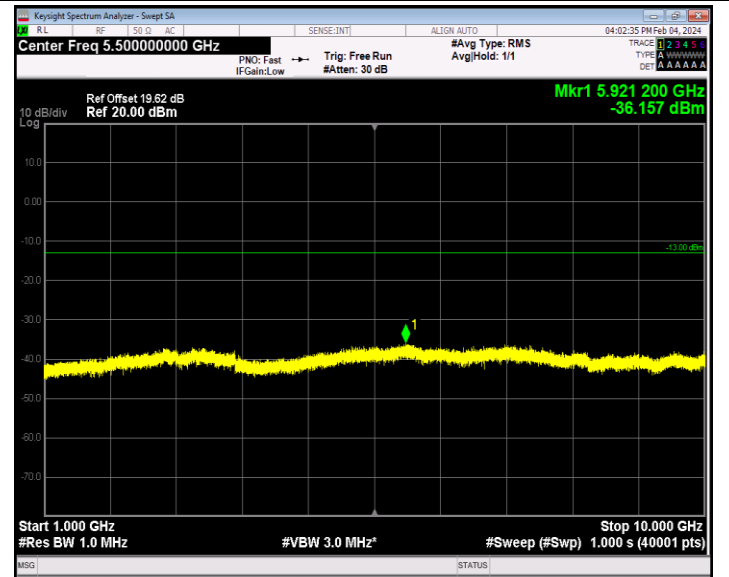
Band26_1.4MHz_QPSK_26797_1RB#0_1000~10000_1000~10000 00
