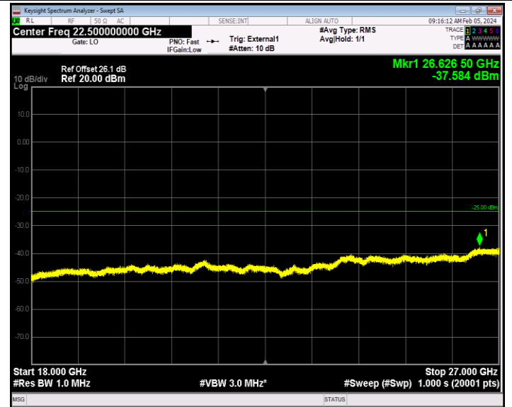
Band41_5MHz_QPSK_40640_1RB#0_18000~27000_18000~27000 00
