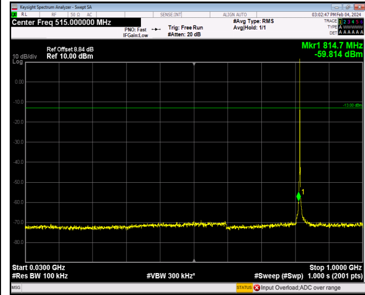
Band26_1.4MHz_16QAM_26740_1RB#0_30~1000_30~1000
