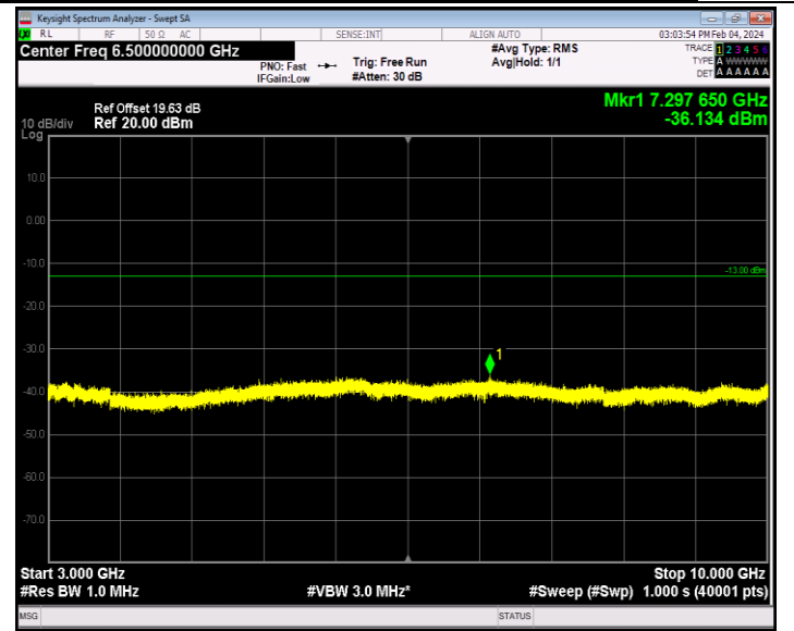
Band26_1.4MHz_64QAM_26740_1RB#0_3000~10000_3000~10 000
