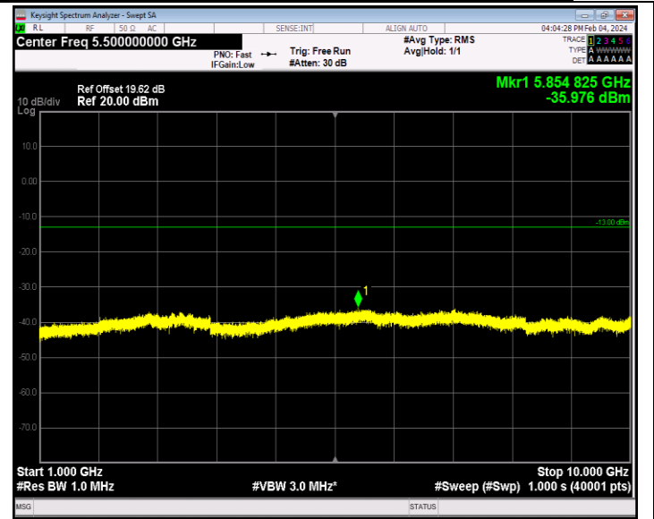
Band26_1.4MHz_64QAM_26915_1RB#0_1000~10000_1000~10000
