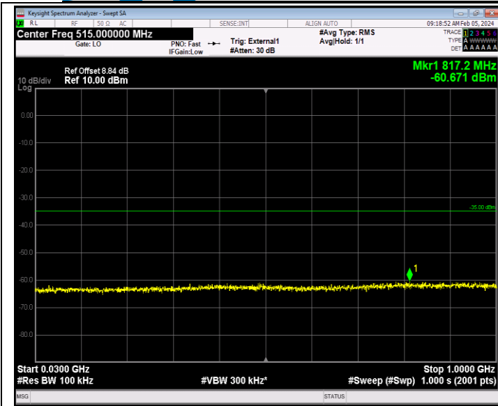
Band41_5MHz_QPSK_41215_1RB#0_30~1000_30~1000
