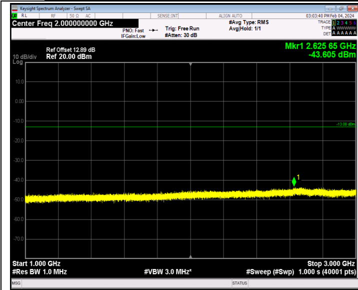
Band26_1.4MHz_64QAM_26740_1RB#0_1000~3000_1000~300 0
