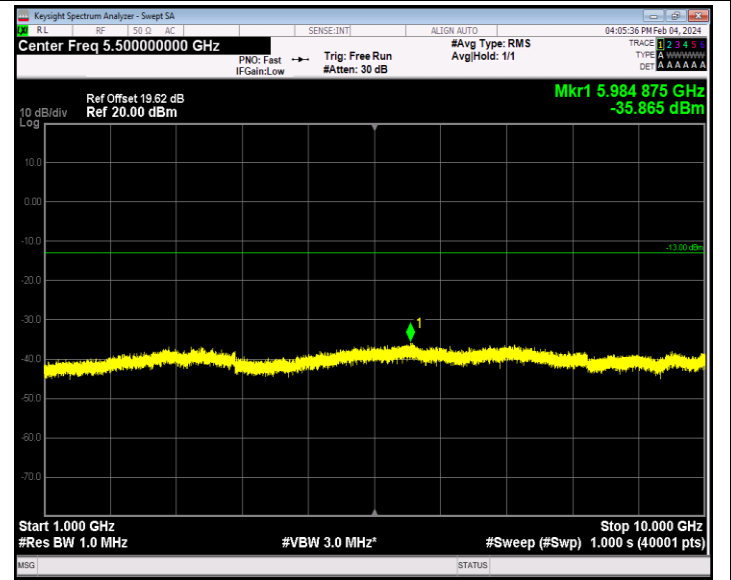
Band26_1.4MHz_64QAM_27033_1RB#0_1000~10000_1000~10000
