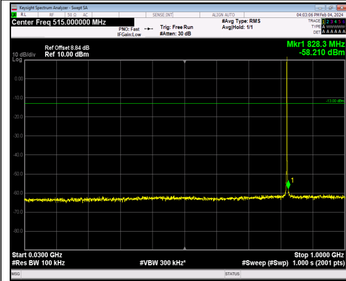
Band26_1.4MHz_64QAM_26797_1RB#0_30~1000_30~1000
