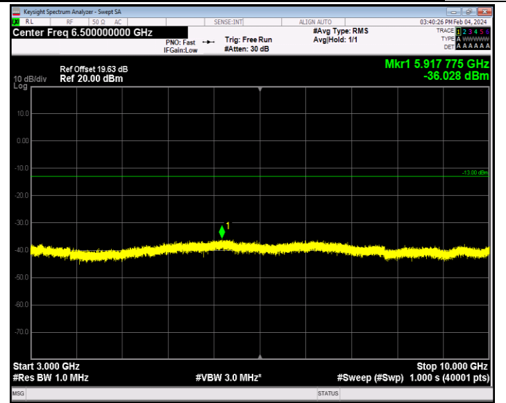
Band26_10MHz_64QAM_26740_1RB#0_3000~10000_3000~10000 00
