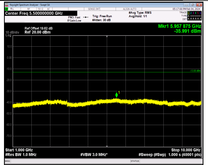
Band26_15MHz_64QAM_26865_1RB#0_1000~10000_1000~1000 00
