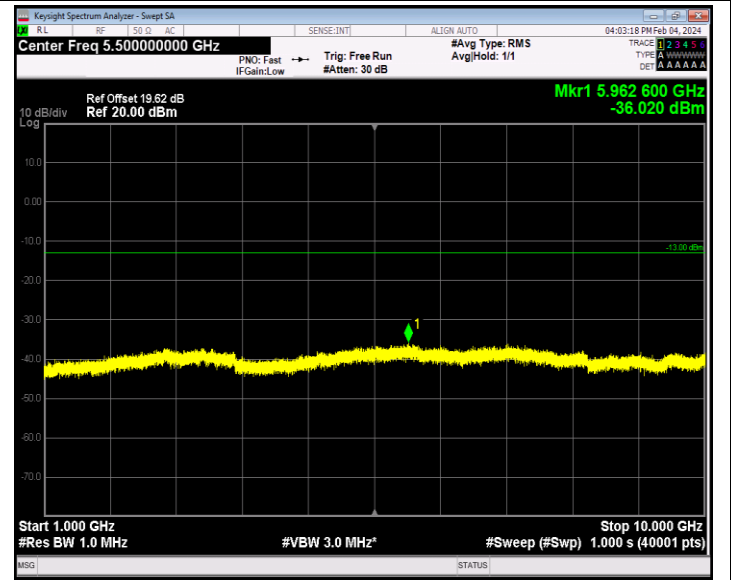
Band26_1.4MHz_64QAM_26797_1RB#0_1000~10000_1000~10000
