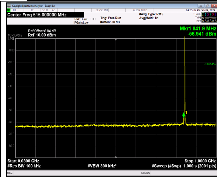
Band26_1.4MHz_16QAM_27033_1RB#0_30~1000_30~1000
