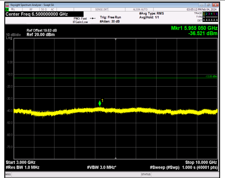
Band26_1.4MHz_16QAM_26783_1RB#0_3000~10000_3000~10000
