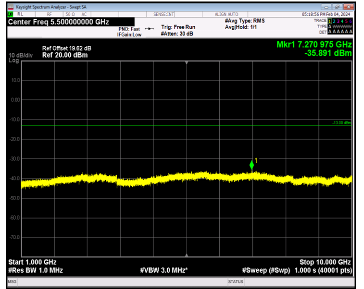
Band26_15MHz_16QAM_26965_1RB#0_1000~10000_1000~1000 00
