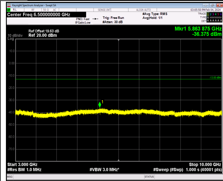
Band26_1.4MHz_64QAM_26783_1RB#0_3000~10000_3000~10000
