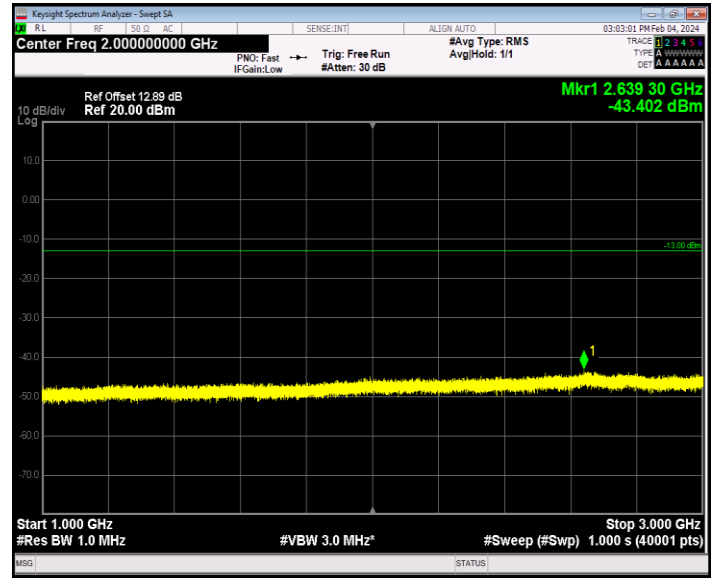
Band26_1.4MHz_16QAM_26740_1RB#0_1000~3000_1000~300 0
