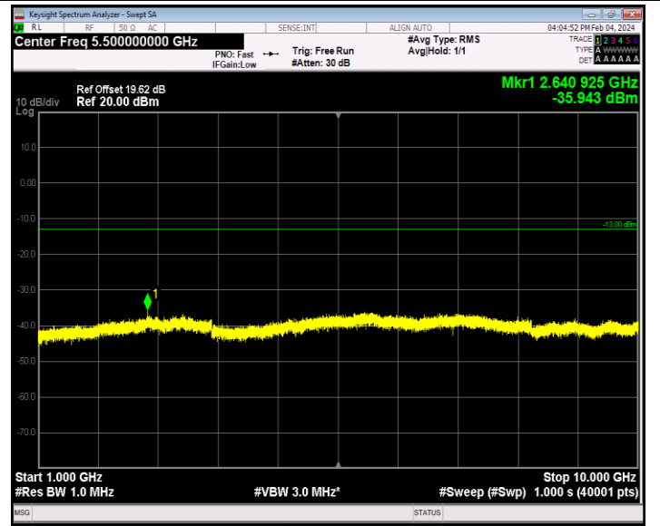
Band26_1.4MHz_QPSK_27033_1RB#0_1000~10000_1000~10000
