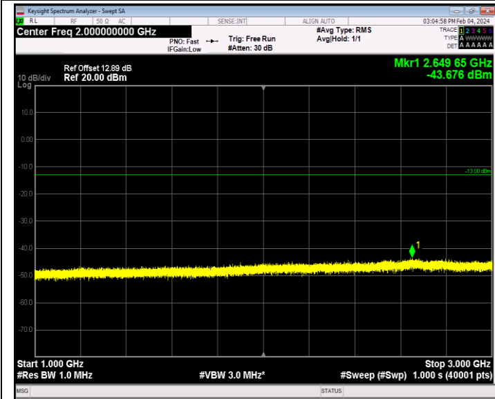
Band26_1.4MHz_16QAM_26783_1RB#0_1000~3000_1000~3000
