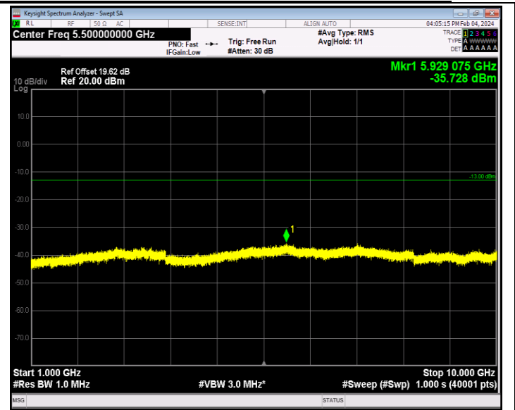
Band26_1.4MHz_16QAM_27033_1RB#0_1000~10000_1000~10000
