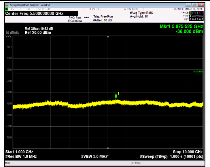
Band26_15MHz_QPSK_26965_1RB#0_1000~10000_1000~1000 0
