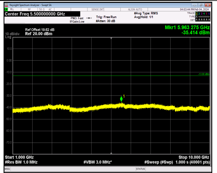
Band26_1.4MHz_QPSK_26915_1RB#0_1000~10000_1000~10000
