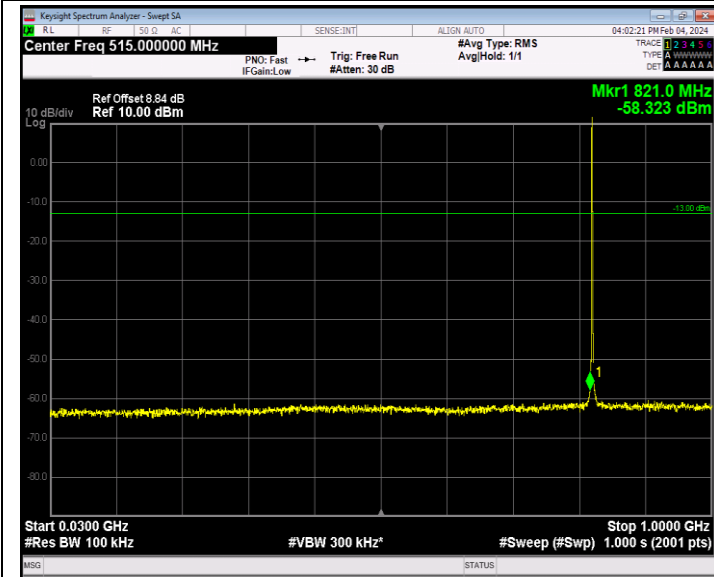
Band26_1.4MHz_QPSK_26797_1RB#0_30~1000_30~1000
