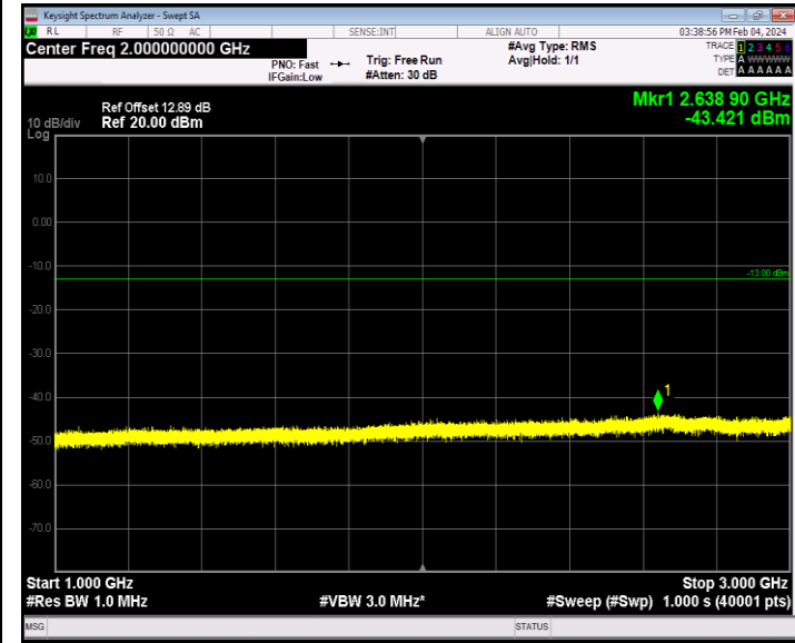
Band26_10MHz_QPSK_26740_1RB#0_1000~3000_1000~3000
