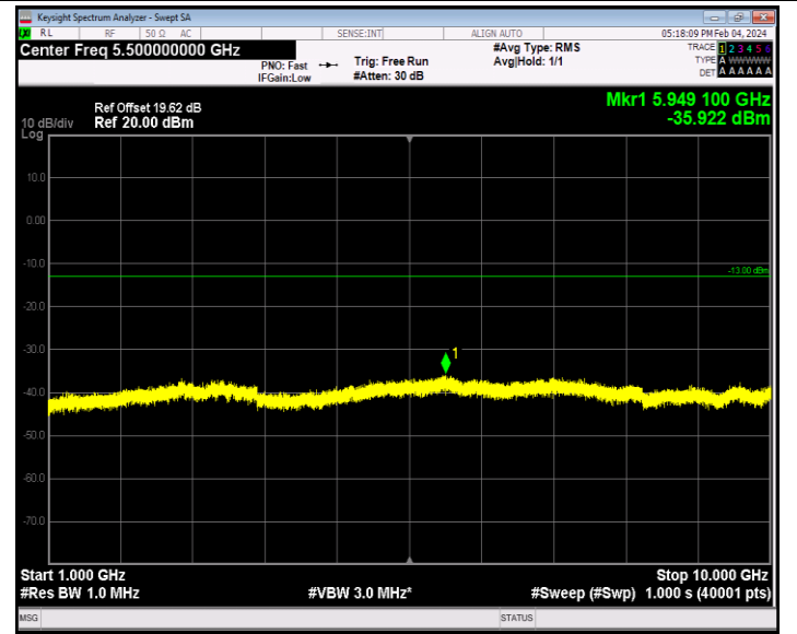
Band26_15MHz_64QAM_26915_1RB#0_1000~10000_1000~1000 00
