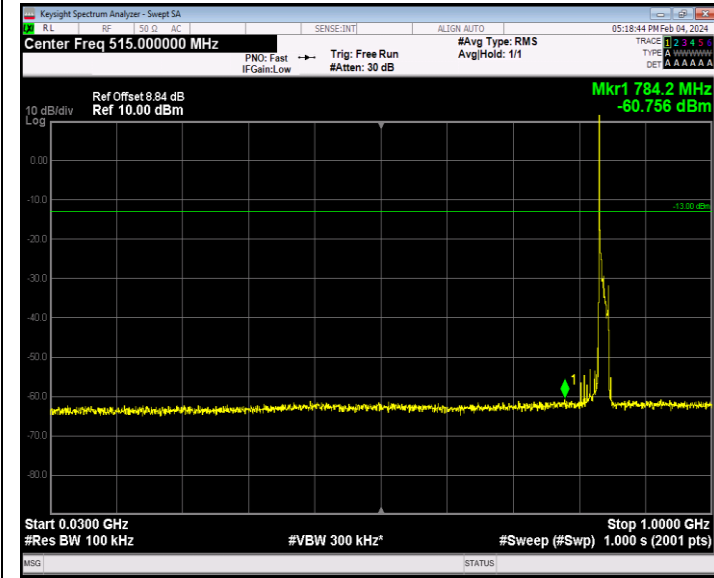
Band26_15MHz_16QAM_26965_1RB#0_30~1000_30~1000
