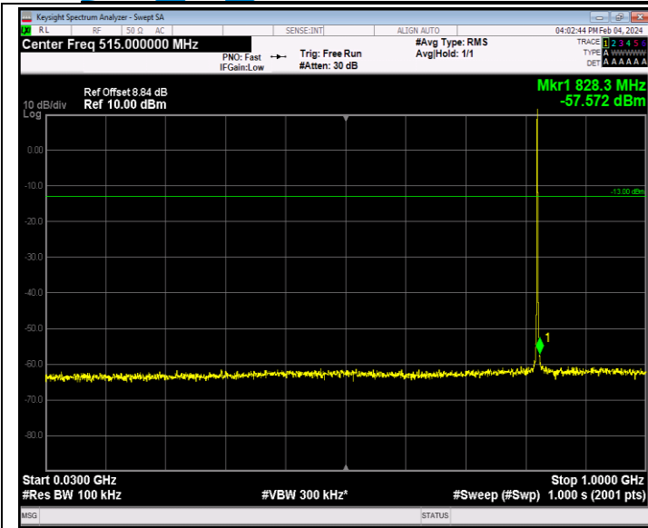
Band26_1.4MHz_16QAM_26797_1RB#0_30~1000_30~1000
