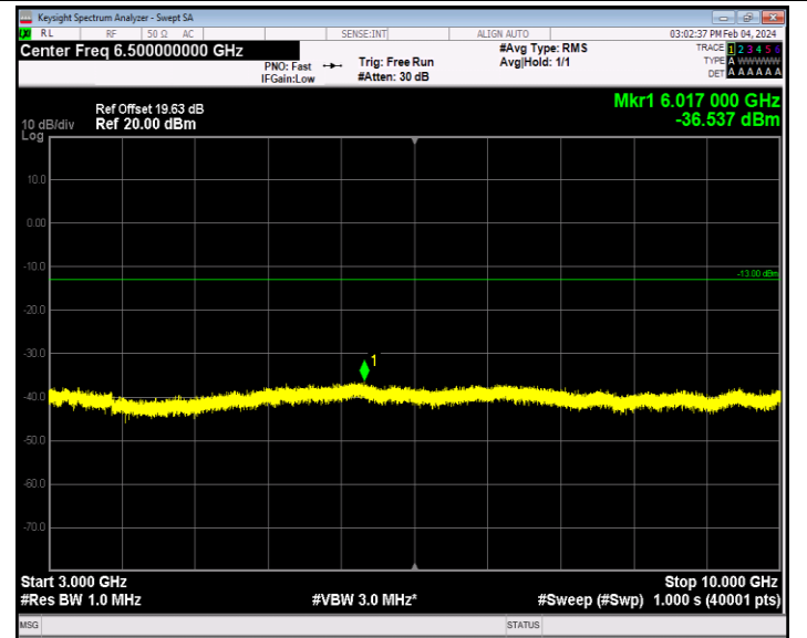
Band26_1.4MHz_QPSK_26740_1RB#0_3000~10000_3000~10000
