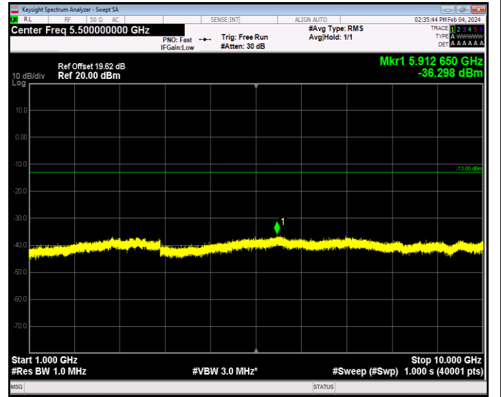
Band12_10MHz_64QAM_23095_1RB#0_1000~10000_1000~1000 00
