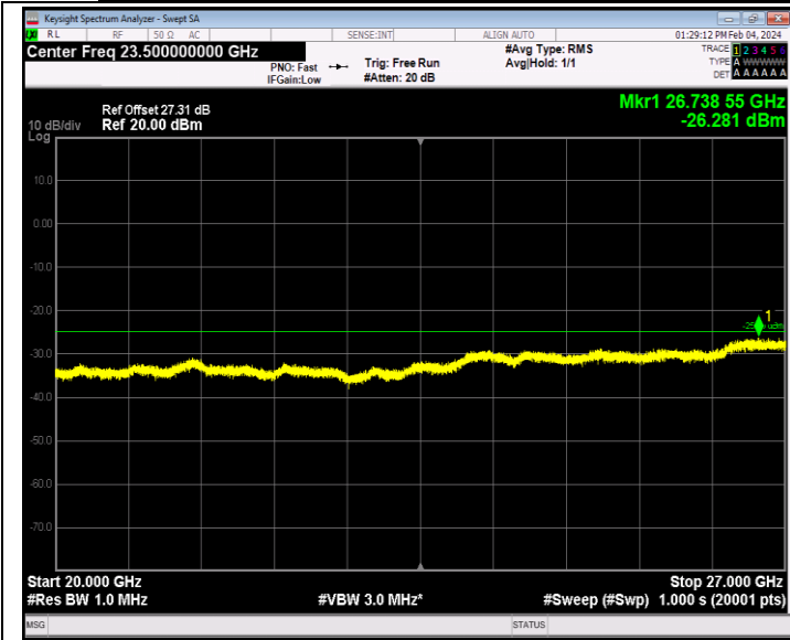
Band7_20MHz_16QAM_21350_1RB#0_20000~27000_20000~27000
