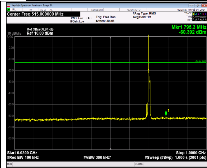
Band12_10MHz_QPSK_23130_1RB#0_30~1000_30~1000
