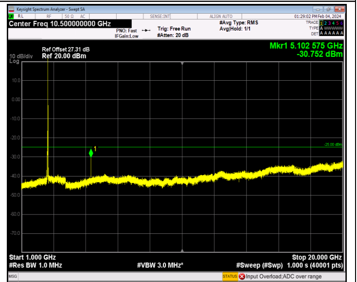
Band7_20MHz_16QAM_21350_1RB#0_1000~20000_1000~2000 0
