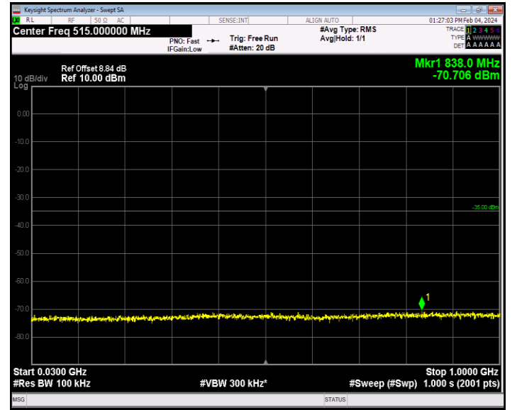
Band7_20MHz_16QAM_21100_1RB#0_30~1000_30~1000
