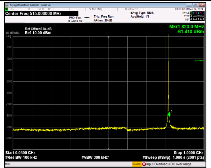
Band26_1.4MHz_QPSK_26740_1RB#0_30~1000_30~1000
