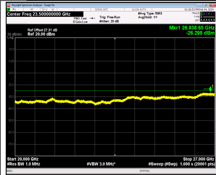
Band7_20MHz_QPSK_21100_1RB#0_20000~27000_20000~27000 00
