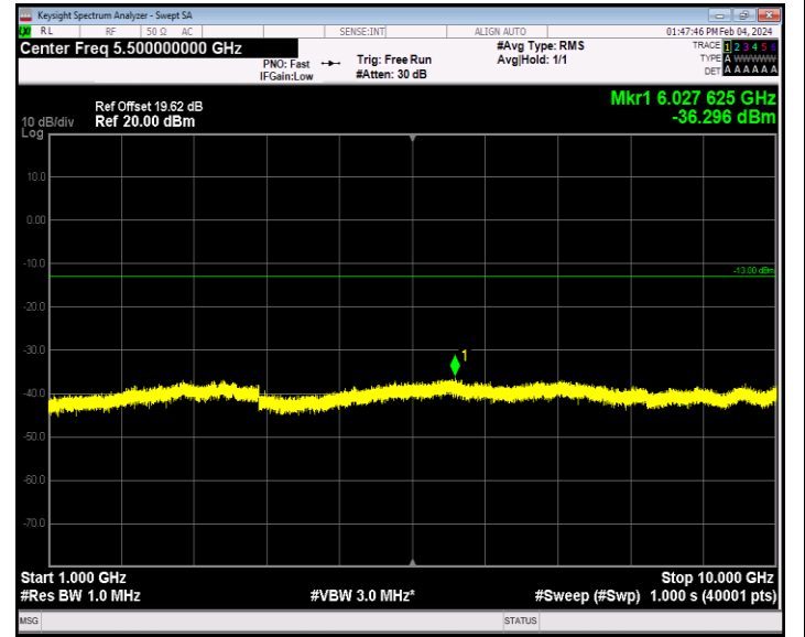
Band12_1.4MHz_QPSK_23017_1RB#0_1000~10000_1000~100 00
