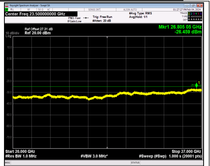
Band7_20MHz_16QAM_21100_1RB#0_20000~27000_20000~27 000
