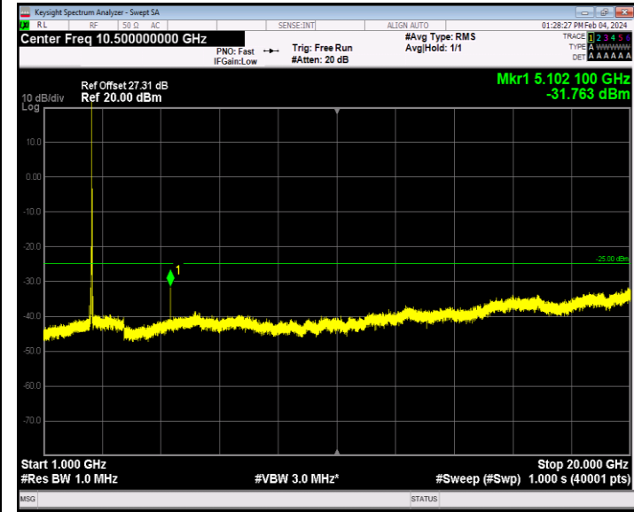
Band7_20MHz_QPSK_21350_1RB#0_1000~20000_1000~20000
