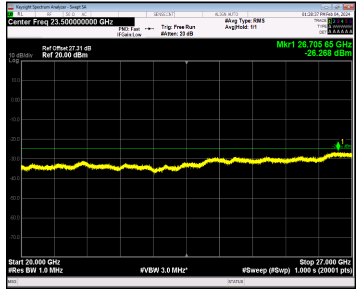
Band7_20MHz_QPSK_21350_1RB#0_20000~27000_20000~27000 00
