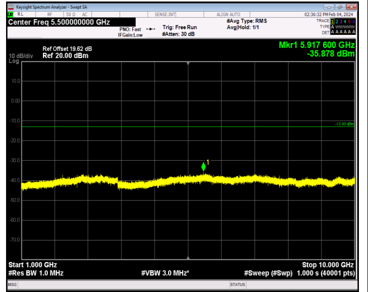
Band12_10MHz_16QAM_23130_1RB#0_1000~10000_1000~1000 00
