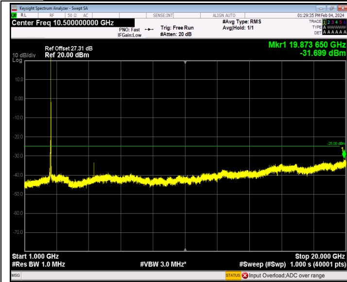
Band7_20MHz_64QAM_21350_1RB#0_1000~20000_1000~2000 0
