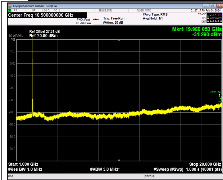
Band7_20MHz_16QAM_21100_1RB#0_1000~20000_1000~2000 0
