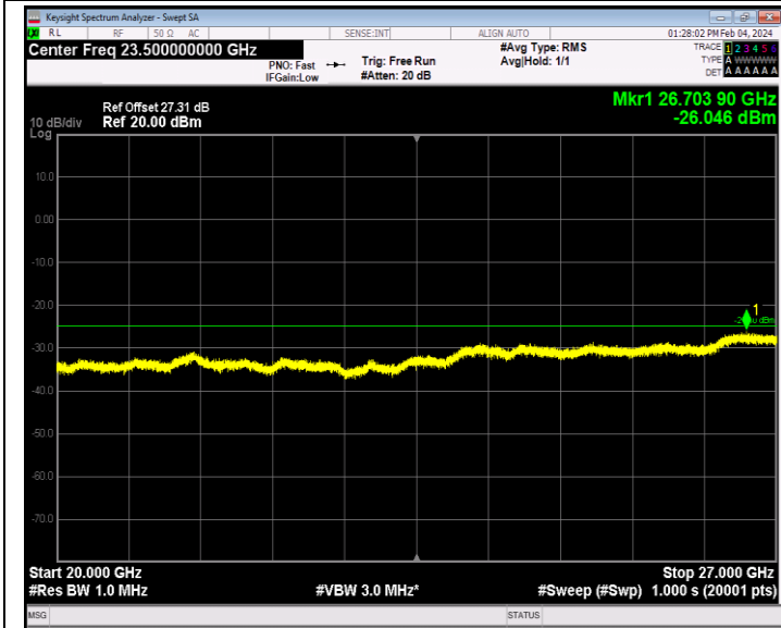
Band7_20MHz_64QAM_21100_1RB#0_20000~27000_20000~27 000
