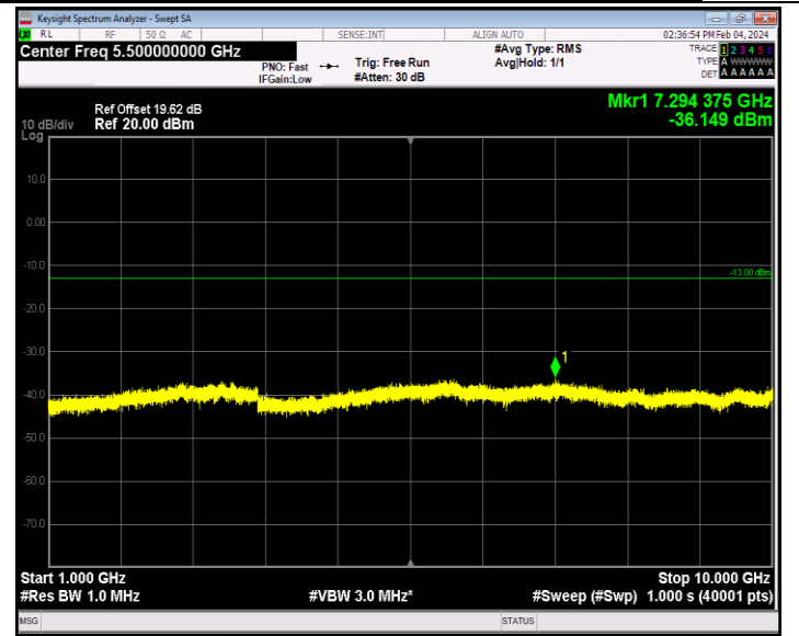
Band12_10MHz_64QAM_23130_1RB#0_1000~10000_1000~10000 00
