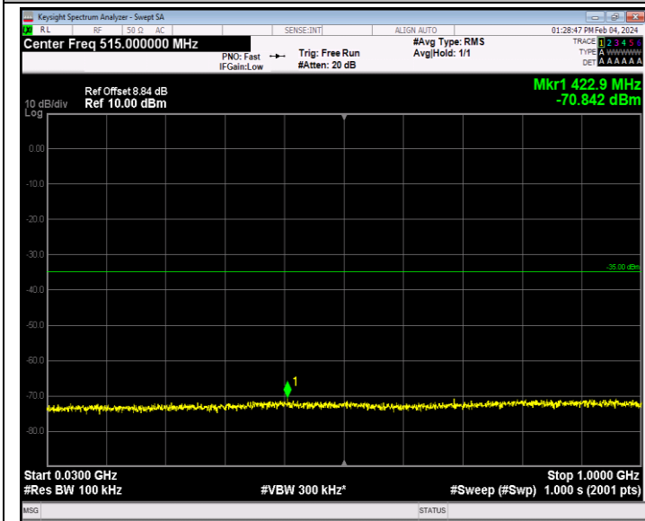
Band7_20MHz_16QAM_21350_1RB#0_30~1000_30~1000
