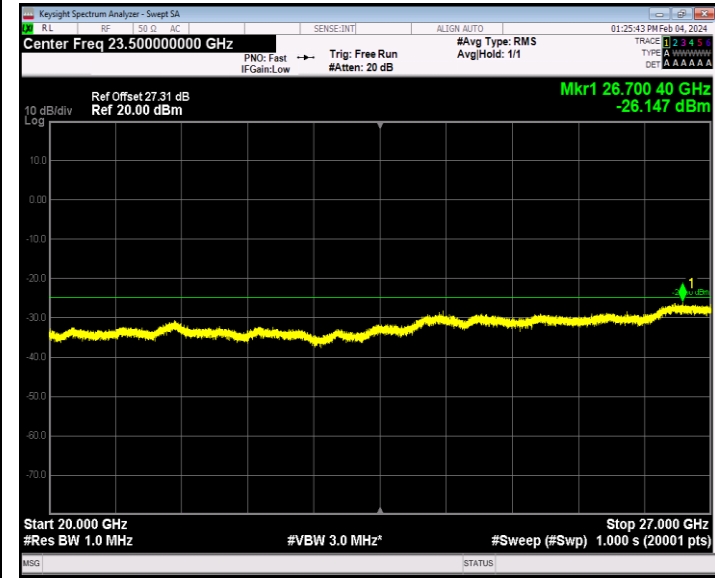
Band7_20MHz_16QAM_20850_1RB#0_20000~27000_20000~27000
