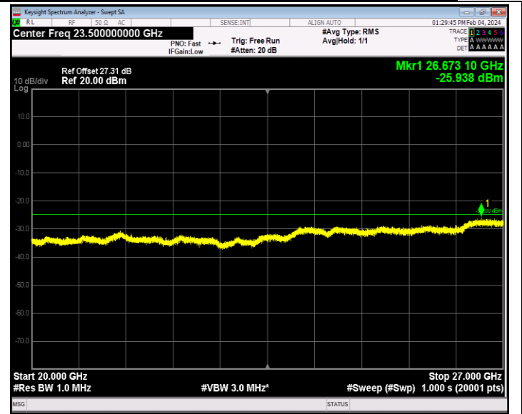
Band7_20MHz_64QAM_21350_1RB#0_20000~27000_20000~27 000
