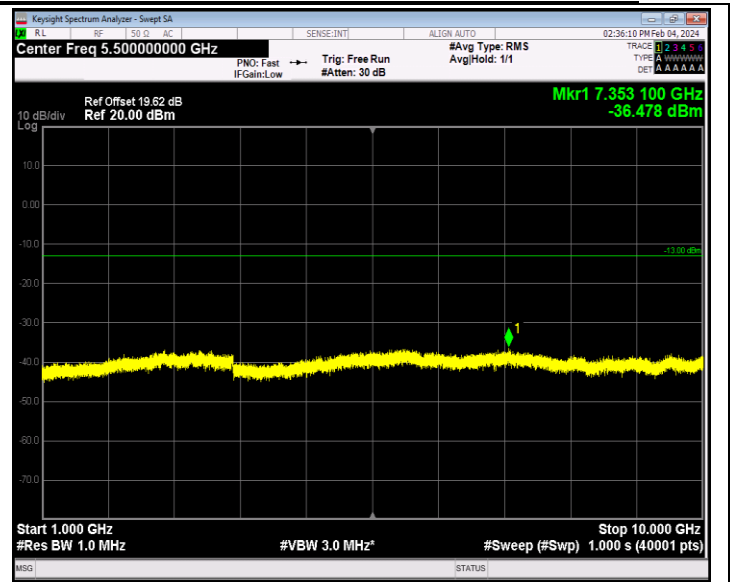
Band12_10MHz_QPSK_23130_1RB#0_1000~10000_1000~1000 0
