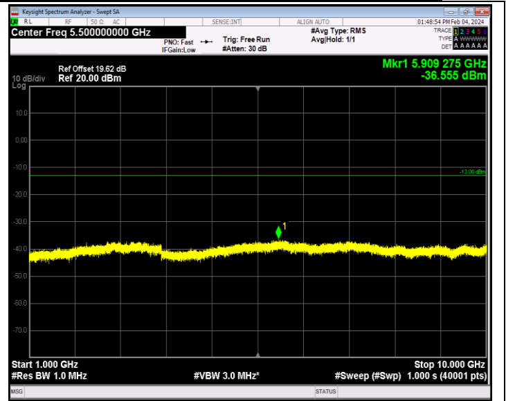
Band12_1.4MHz_QPSK_23095_1RB#0_1000~10000_1000~10000
