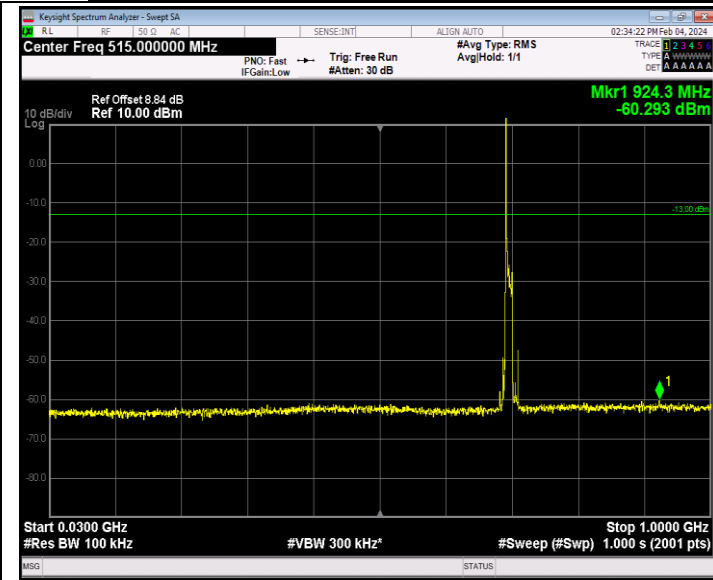
Band12_10MHz_64QAM_23060_1RB#0_30~1000_30~1000
