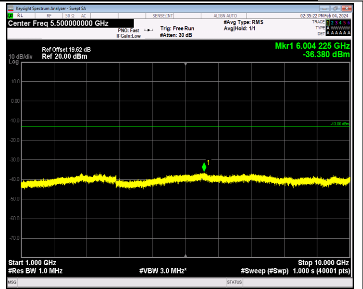
Band12_10MHz_16QAM_23095_1RB#0_1000~10000_1000~1000 00
