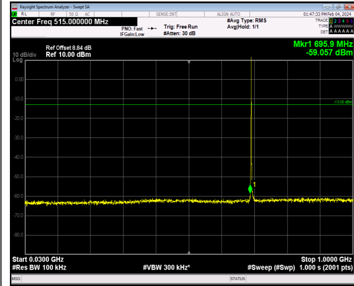
Band12_1.4MHz_QPSK_23017_1RB#0_30~1000_30~1000
