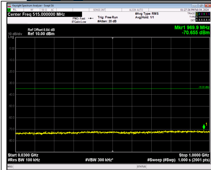
Band7_20MHz_64QAM_21100_1RB#0_30~1000_30~1000
