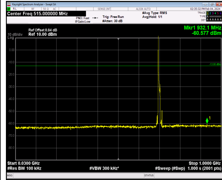
Band12_10MHz_64QAM_23095_1RB#0_30~1000_30~1000
