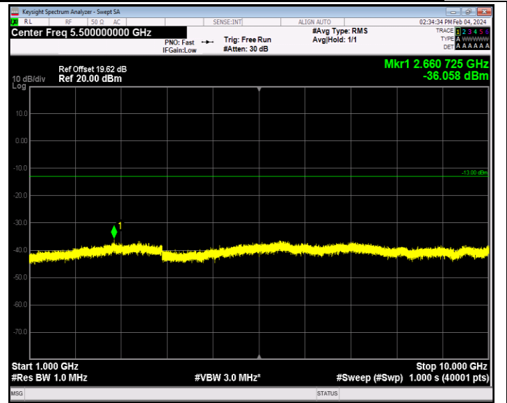
Band12_10MHz_64QAM_23060_1RB#0_1000~10000_1000~1000 00
