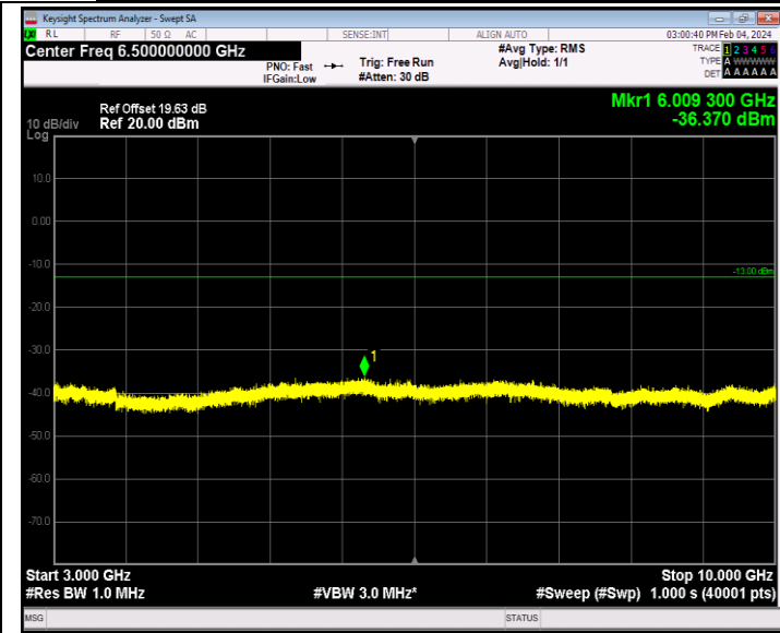
Band26_1.4MHz_QPSK_26697_1RB#0_3000~10000_3000~10000
