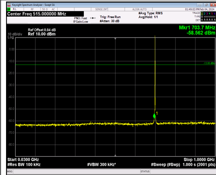
Band12_1.4MHz_16QAM_23095_1RB#0_30~1000_30~1000
