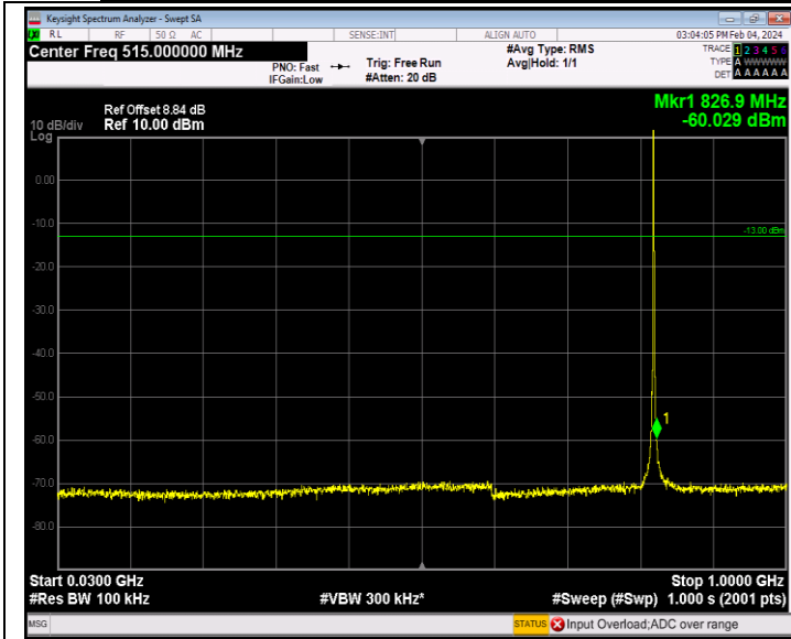
Band26_1.4MHz_QPSK_26783_1RB#0_30~1000_30~1000
