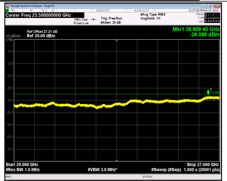
Band7_5MHz_16QAM_21425_1RB#0_20000~27000_20000~27000 00
