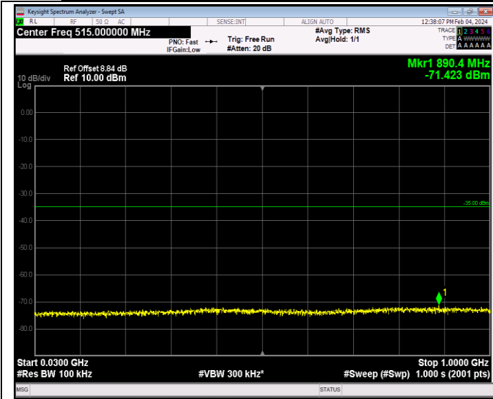
Band7_5MHz_64QAM_21425_1RB#0_30~1000_30~1000
