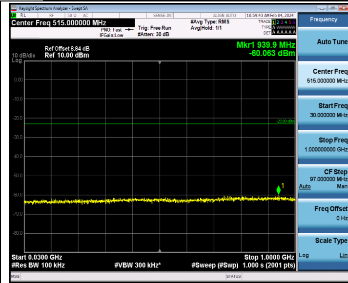
Band2_1.4MHz_QPSK_19193_1RB#0_30~1000_30~1000
