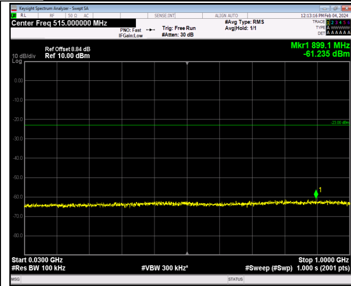
Band2_20MHz_16QAM_19100_1RB#0_30~1000_30~1000
