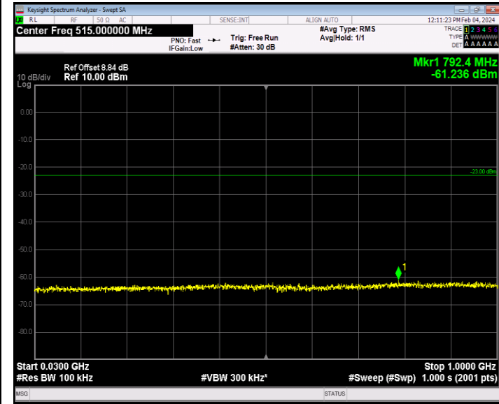
Band2_20MHz_64QAM_18700_1RB#0_30~1000_30~1000
