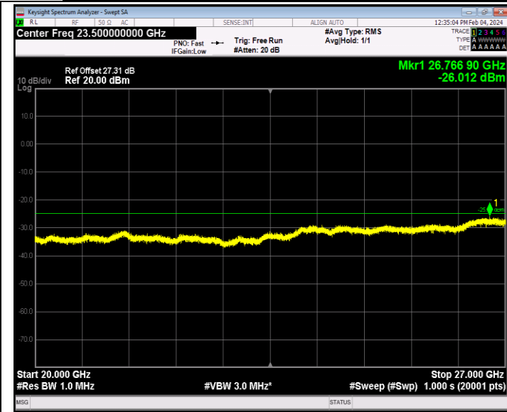
Band7_5MHz_64QAM_20775_1RB#0_20000~27000_20000~27000
