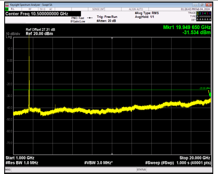
Band7_20MHz_QPSK_21100_1RB#0_1000~20000_1000~20000
