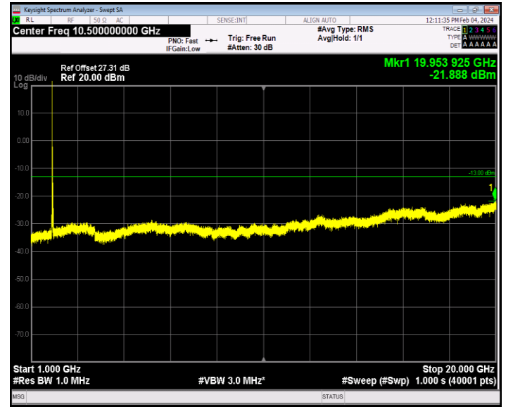
Band2_20MHz_64QAM_18700_1RB#0_1000~20000_1000~2000 0
