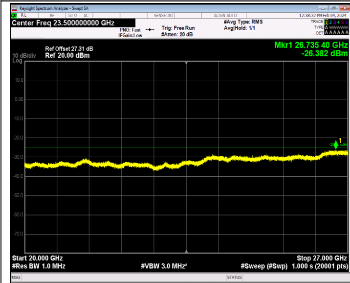
Band7_5MHz_64QAM_21425_1RB#0_20000~27000_20000~270
