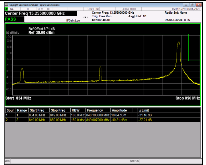
Band26_15MHz_QPSK_26965_1RB#74
