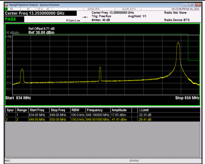
Band26_15MHz_64QAM_26965_1RB#74
