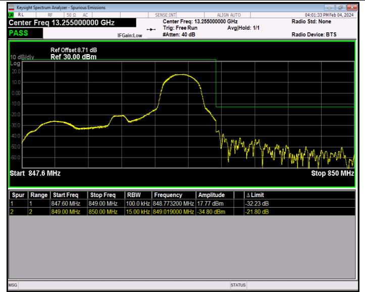
Band26_1.4MHz_64QAM_27033_1RB#5
