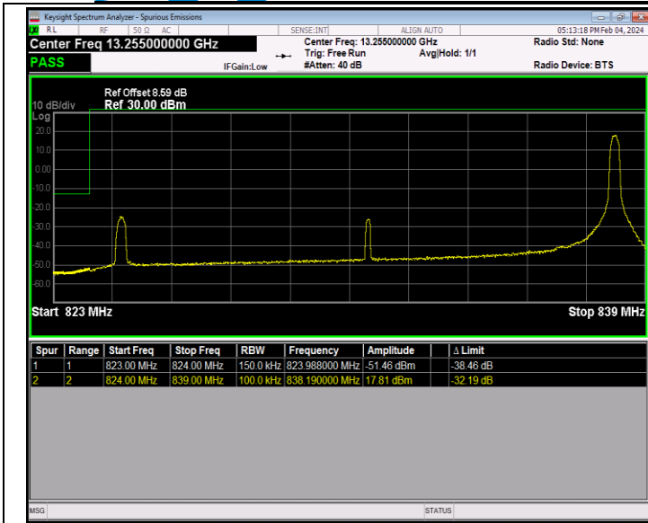
Band26_15MHz_64QAM_26865_1RB#74
