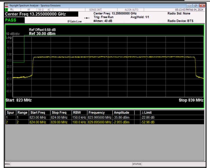
Band26_15MHz_16QAM_26865_75RB#0
