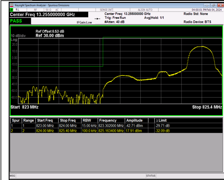
Band26_1.4MHz_64QAM_26797_1RB#5
