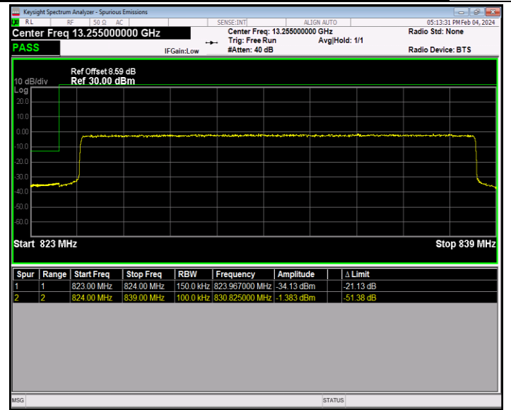
Band26_15MHz_QPSK_26865_75RB#0
