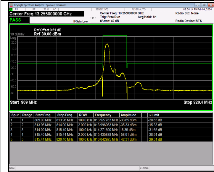
Band26_1.4MHz_64QAM_26697_1RB#0
