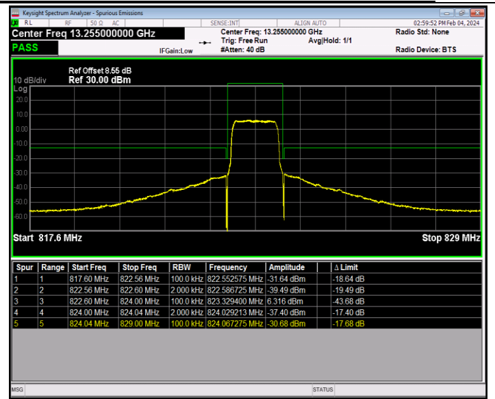
Band26_1.4MHz_64QAM_26783_6RB#0
