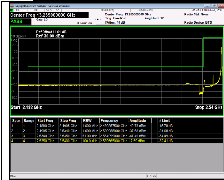
Band41_5MHz_64QAM_40065_1RB#24
