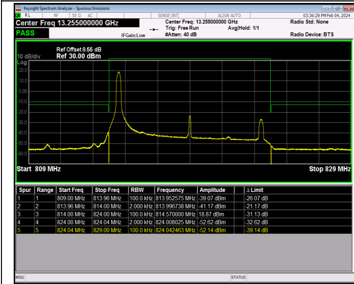
Band26_10MHz_QPSK_26740_1RB#0
