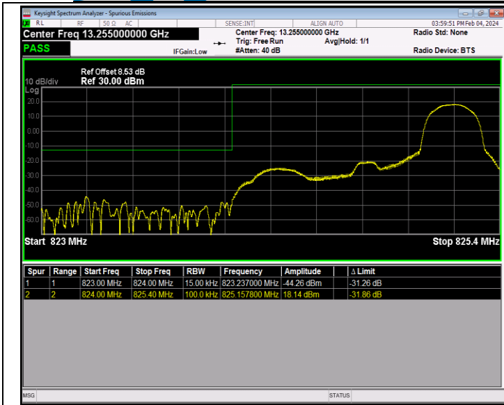
Band26_1.4MHz_16QAM_26797_1RB#5
