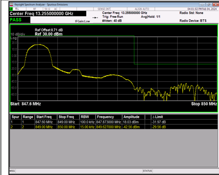
Band26_1.4MHz_64QAM_27033_1RB#0
