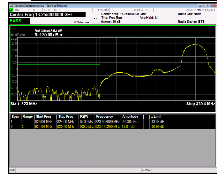
Band26_1.4MHz_QPSK_26797_1RB#5
