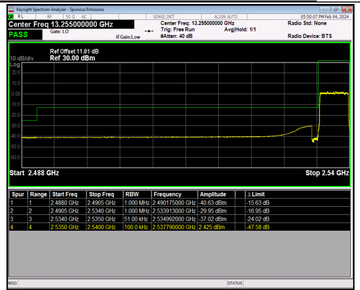
Band41_5MHz_16QAM_40065_25RB#0
