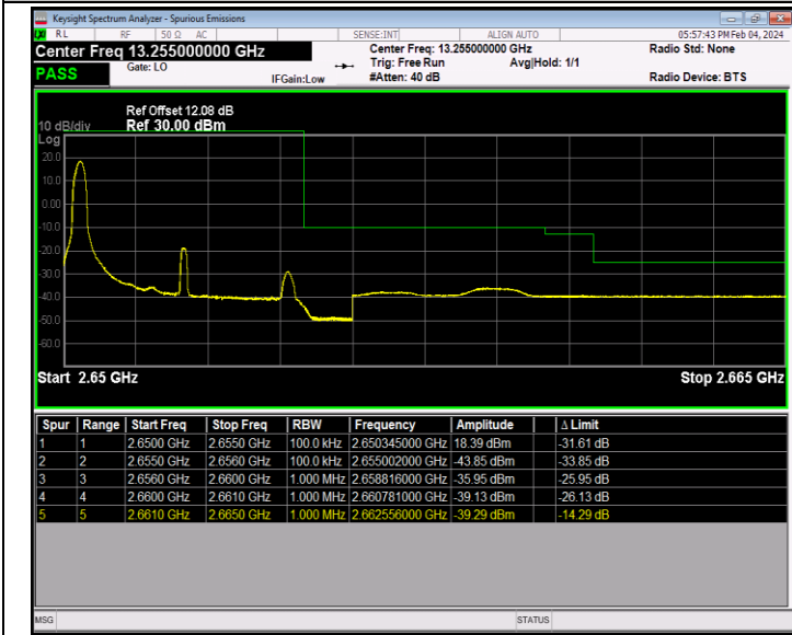
Band41_5MHz_16QAM_41215_1RB#0
