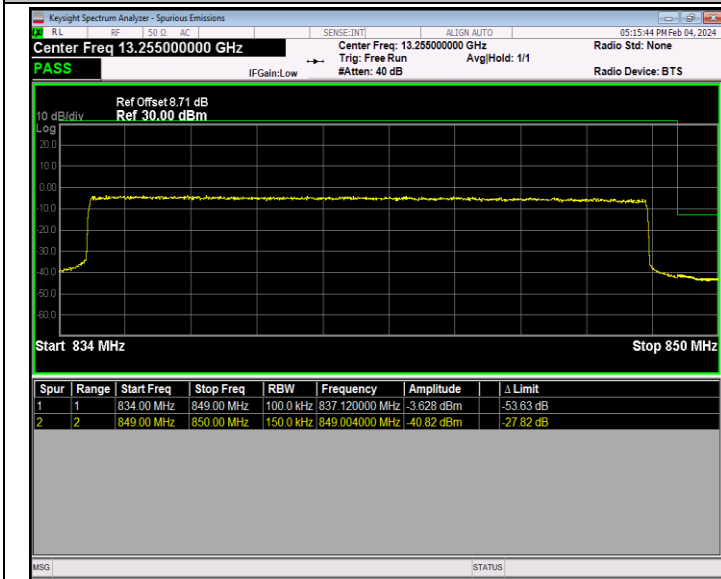
Band26_15MHz_64QAM_26965_75RB#0
