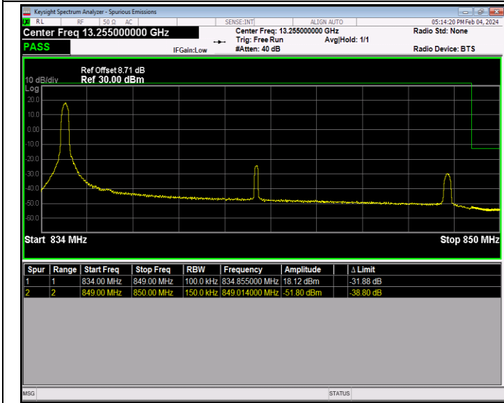
Band26_15MHz_16QAM_26965_1RB#0
