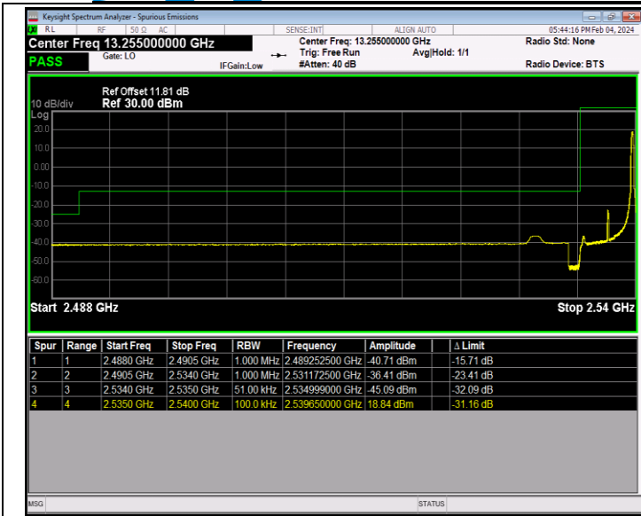
Band41_5MHz_QPSK_40065_1RB#24
