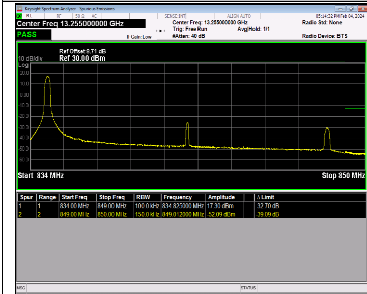
Band26_15MHz_64QAM_26965_1RB#0
