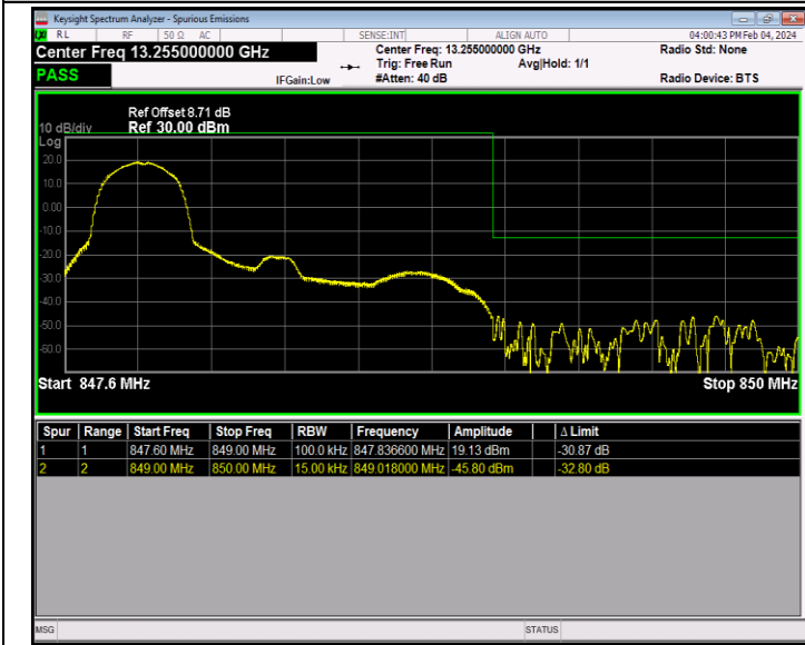
Band26_1.4MHz_QPSK_27033_1RB#0
