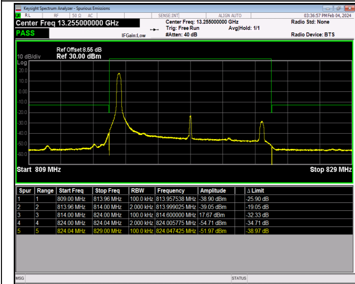
Band26_10MHz_64QAM_26740_1RB#0
