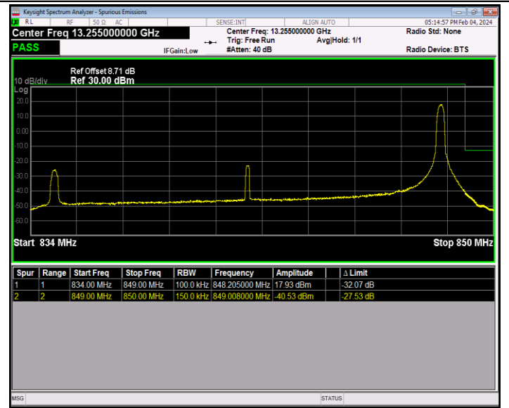
Band26_15MHz_16QAM_26965_1RB#74
