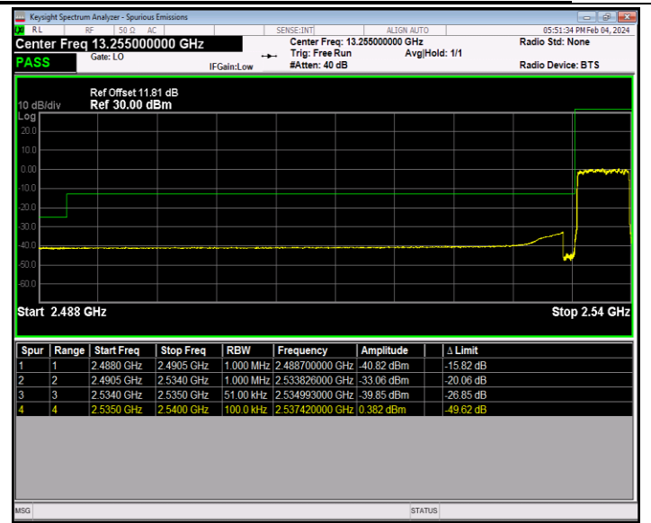
Band41_5MHz_64QAM_40065_25RB#0
