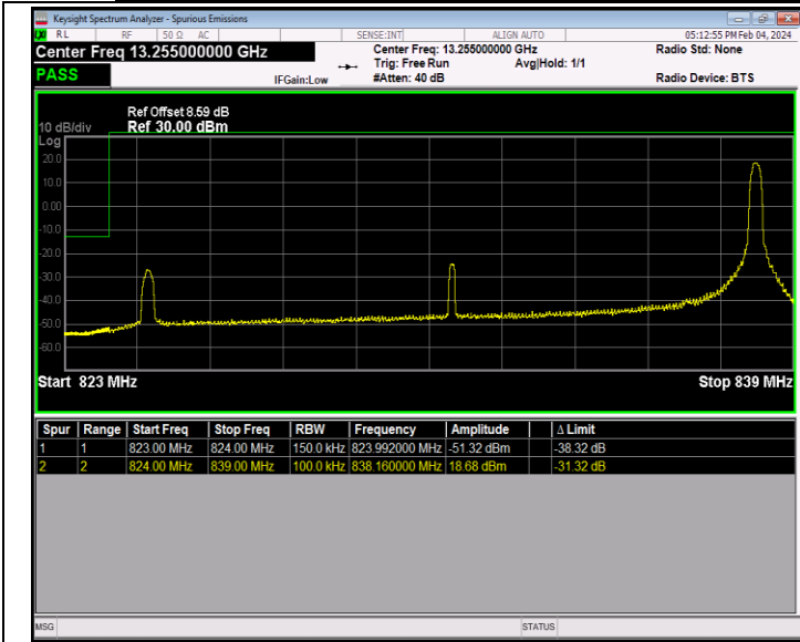
Band26_15MHz_QPSK_26865_1RB#74
