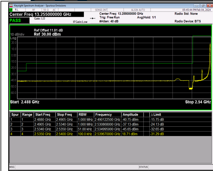
Band41_5MHz_16QAM_40065_1RB#24
