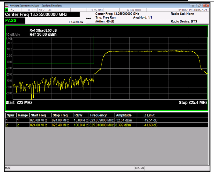
Band26_1.4MHz_16QAM_26797_6RB#0
