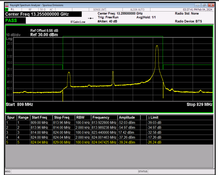
Band26_10MHz_64QAM_26740_1RB#49
