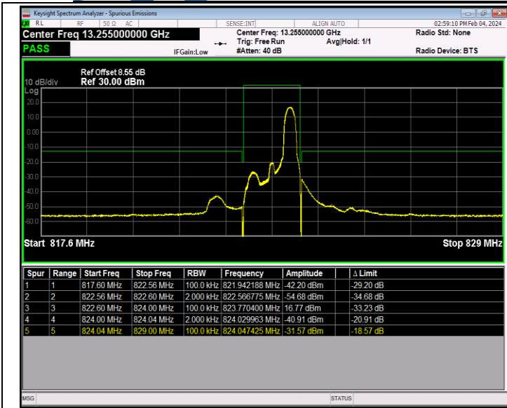
Band26_1.4MHz_64QAM_26783_1RB#5
