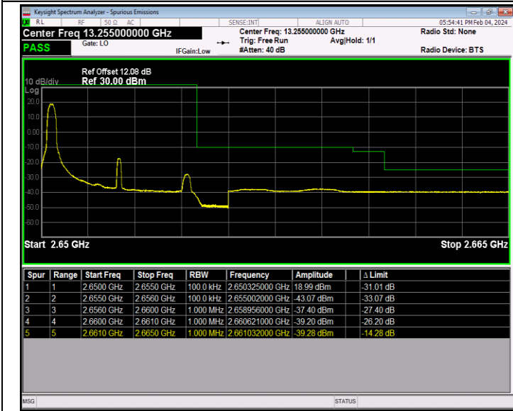
Band41_5MHz_QPSK_41215_1RB#0
