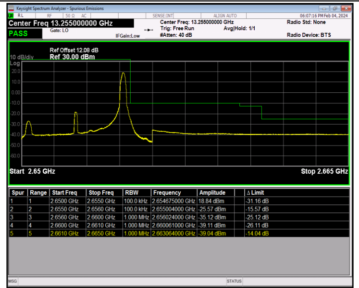
Band41_5MHz_16QAM_41215_1RB#24
