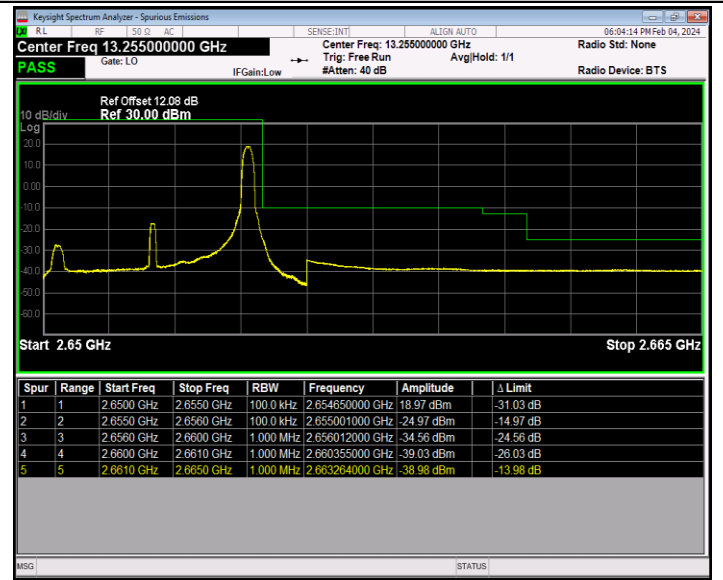
Band41_5MHz_QPSK_41215_1RB#24
