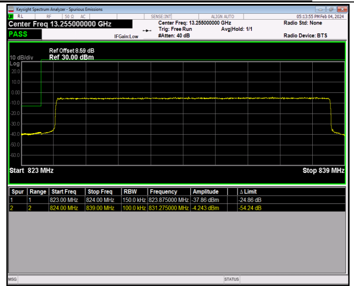
Band26_15MHz_64QAM_26865_75RB#0
