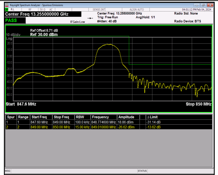
Band26_1.4MHz_QPSK_27033_1RB#5
