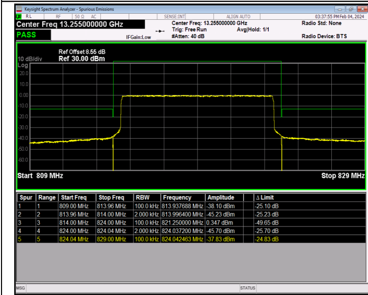
Band26_10MHz_QPSK_26740_50RB#0
