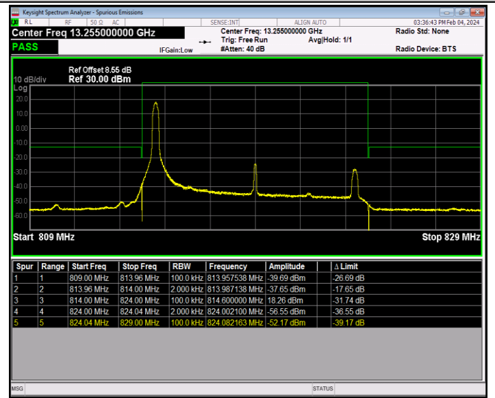
Band26_10MHz_16QAM_26740_1RB#0
