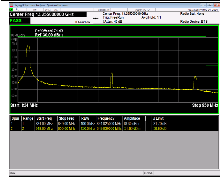
Band26_15MHz_QPSK_26965_1RB#0
