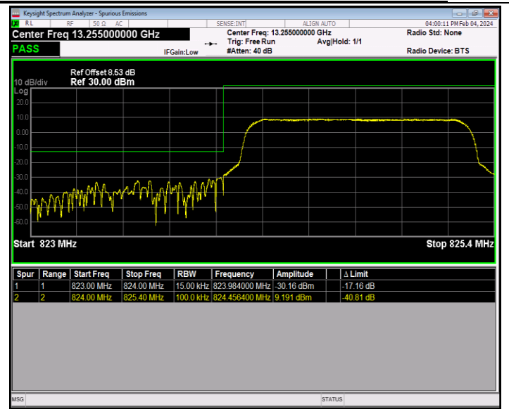
Band26_1.4MHz_QPSK_26797_6RB#0
