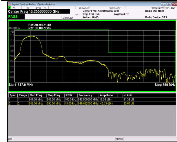
Band26_1.4MHz_16QAM_27033_1RB#0
