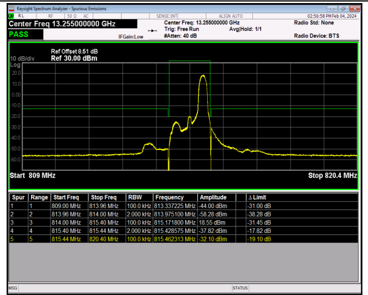
Band26_1.4MHz_64QAM_26697_1RB#5
