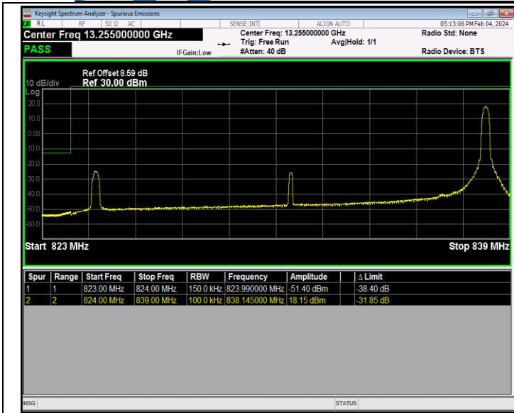
Band26_15MHz_16QAM_26865_1RB#74
