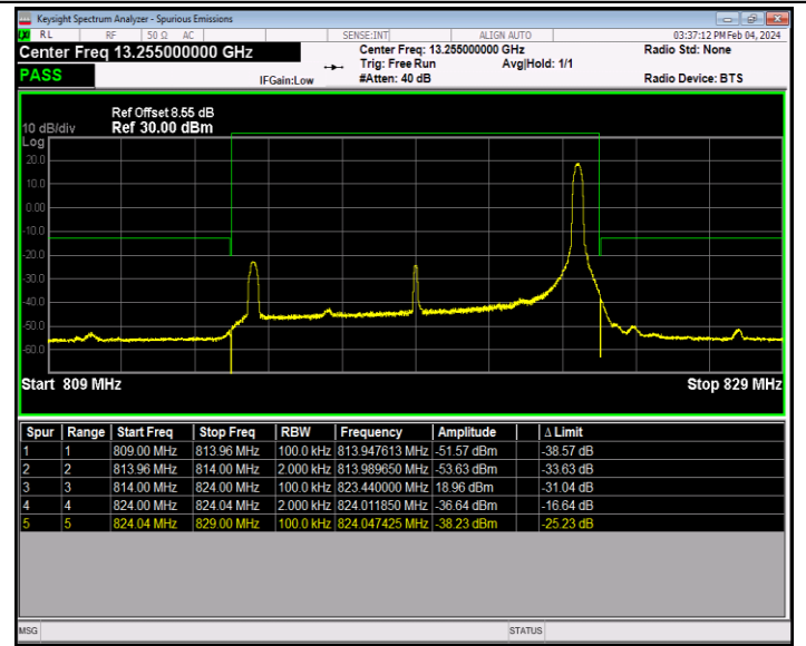
Band26_10MHz_QPSK_26740_1RB#49
