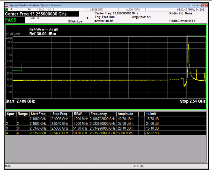
Band41_5MHz_64QAM_40065_1RB#0
