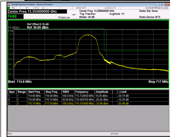
Band12_1.4MHz_QPSK_23173_1RB#5
