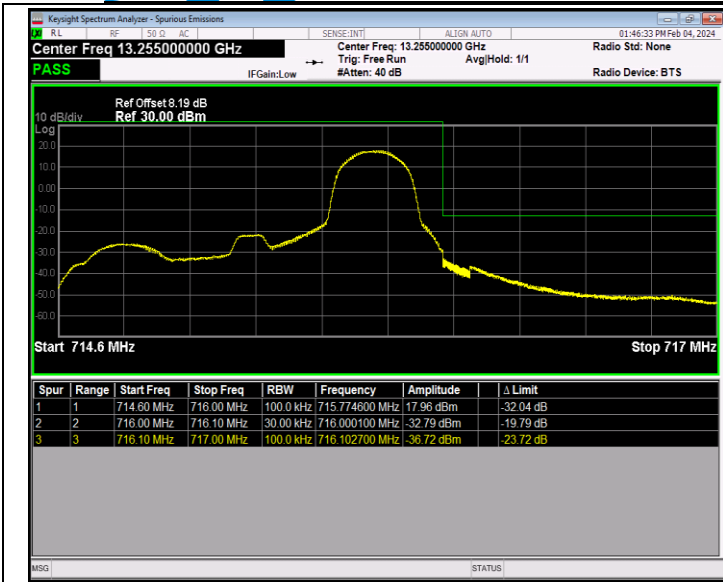
Band12_1.4MHz_64QAM_23173_1RB#5
