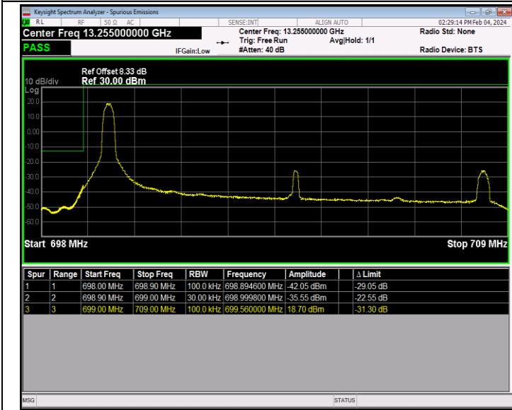
Band12_10MHz_QPSK_23060_1RB#0
