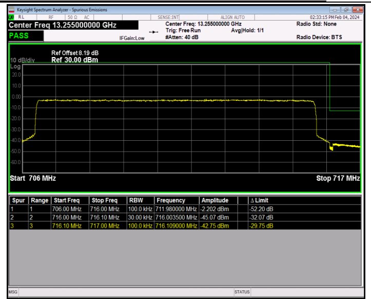
Band12_10MHz_64QAM_23130_50RB#0
