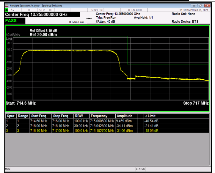
Band12_1.4MHz_QPSK_23173_6RB#0
