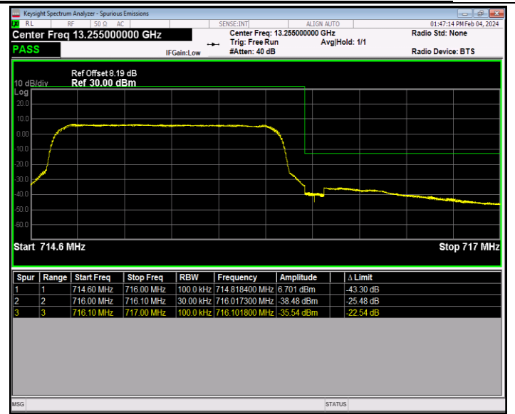
Band12_1.4MHz_64QAM_23173_6RB#0
