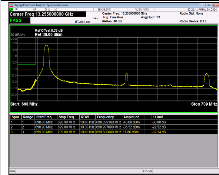
Band12_10MHz_64QAM_23060_1RB#0
