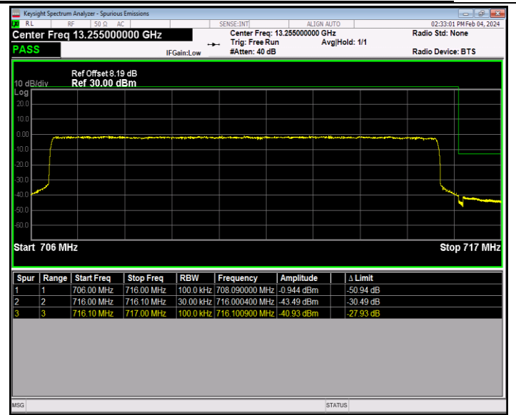
Band12_10MHz_16QAM_23130_50RB#0
