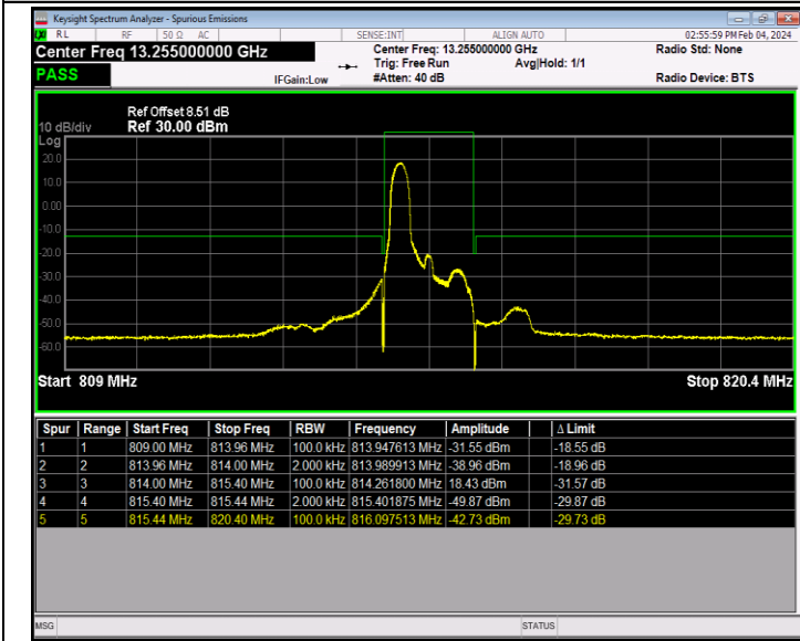
Band26_1.4MHz_16QAM_26697_1RB#0
