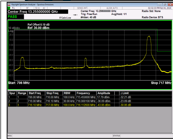
Band12_10MHz_64QAM_23130_1RB#49
