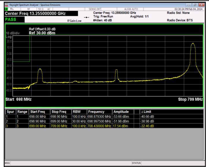
Band12_10MHz_64QAM_23060_1RB#49
