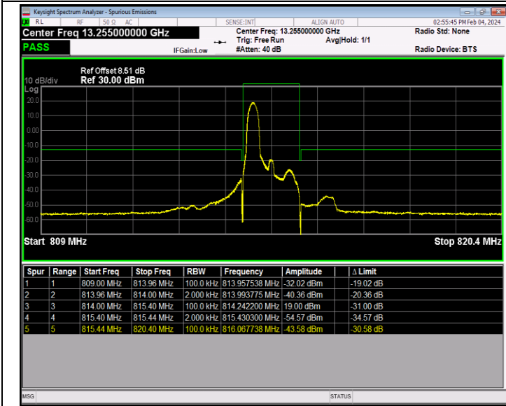
Band26_1.4MHz_QPSK_26697_1RB#0
