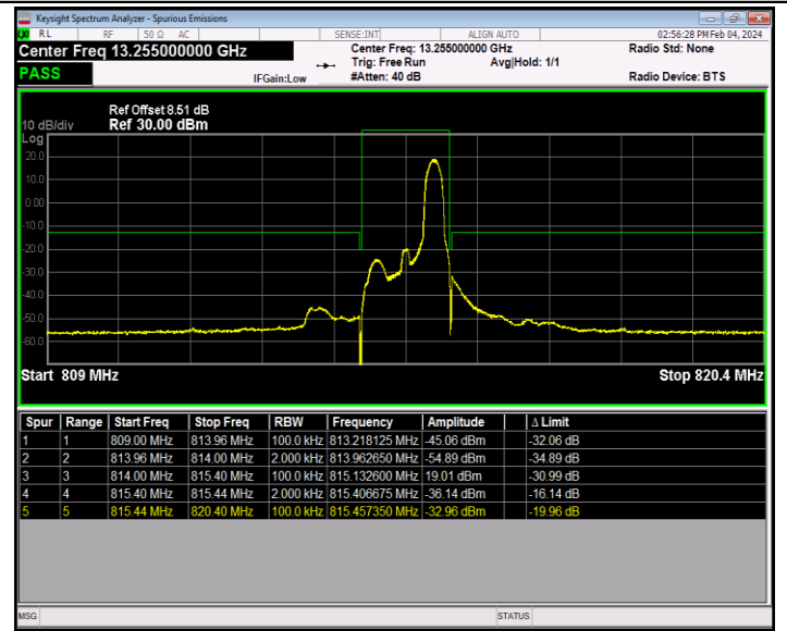
Band26_1.4MHz_QPSK_26697_1RB#5
