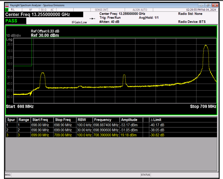
Band12_10MHz_QPSK_23060_1RB#49
