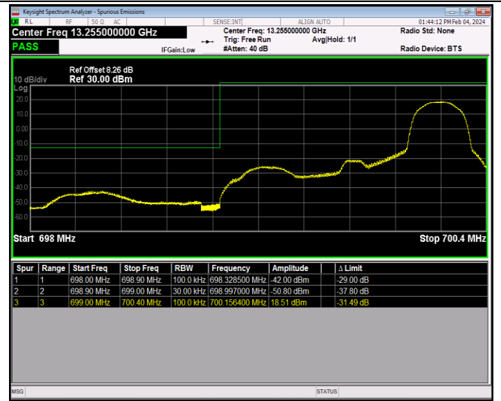
Band12_1.4MHz_16QAM_23017_1RB#5
