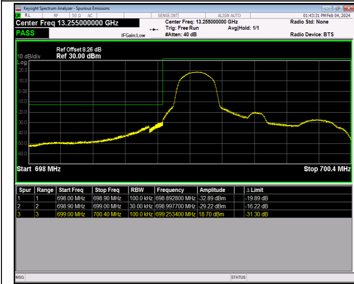
Band12_1.4MHz_16QAM_23017_1RB#0
