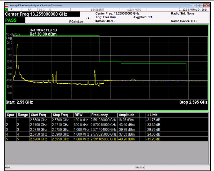
Band7_20MHz_64QAM_21350_1RB#0
