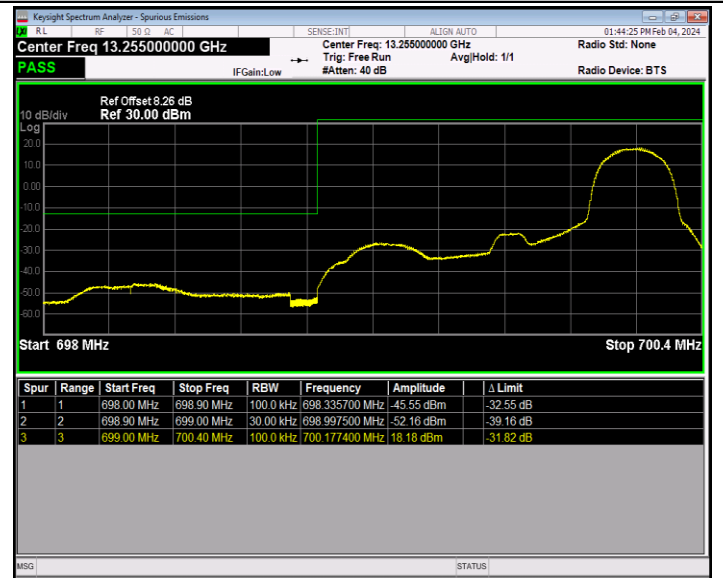
Band12_1.4MHz_64QAM_23017_1RB#5
