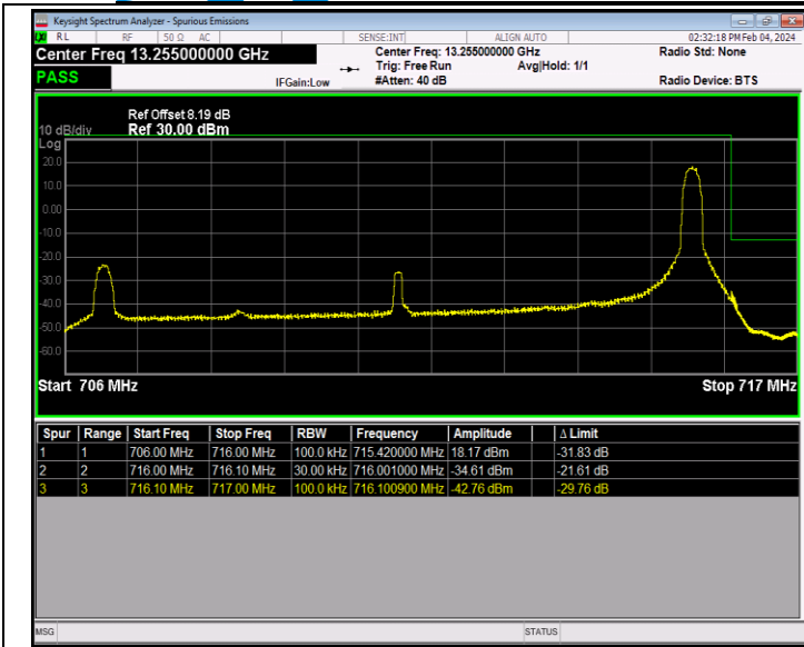
Band12_10MHz_16QAM_23130_1RB#49
