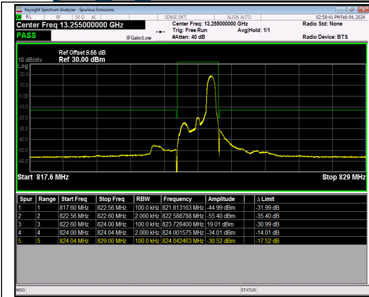
Band26_1.4MHz_QPSK_26783_1RB#5
