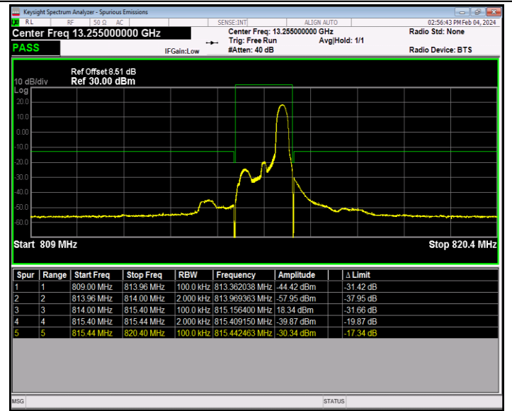
Band26_1.4MHz_16QAM_26697_1RB#5
