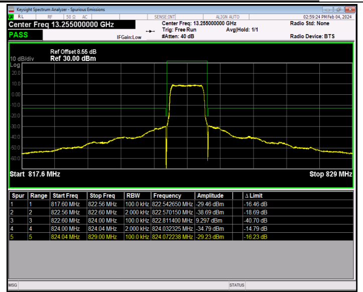
Band26_1.4MHz_QPSK_26783_6RB#0
