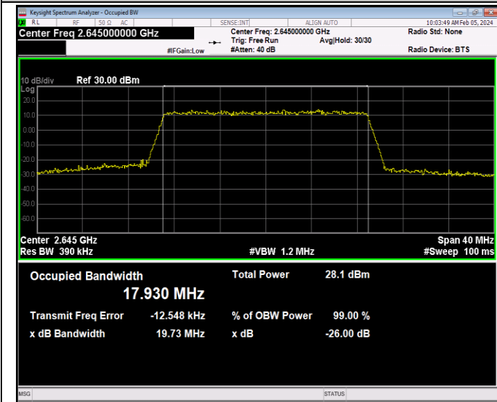
41(2535-2655)-20MHz-64QAM-41140-100RB#0-PASS
