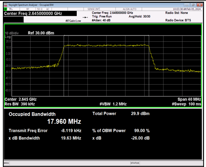
41(2535-2655)-20MHz-16QAM-41140-100RB#0-PASS
