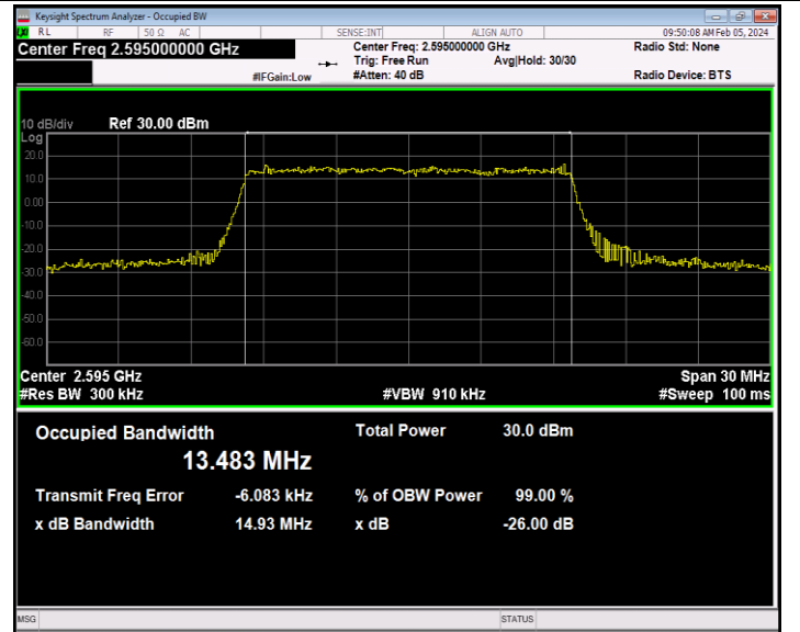
41(2535-2655)-15MHz-16QAM-40640-75RB#0-PASS
