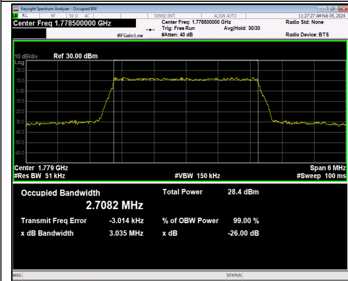
Band66-3MHz-64QAM-132657-15RB#0-PASS
