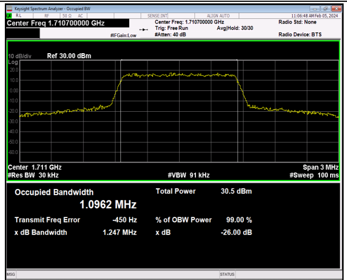
Band66-1.4MHz-QPSK-131979-6RB#0-PASS
