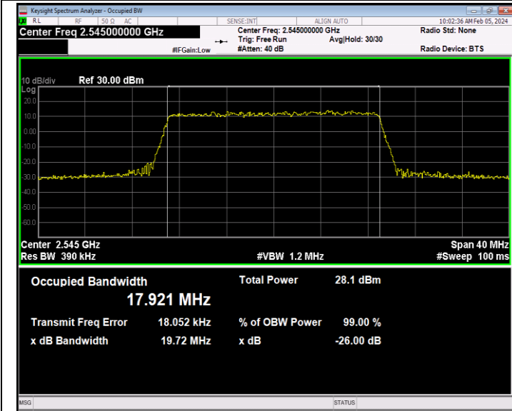
41(2535-2655)-20MHz-64QAM-40140-100RB#0-PASS
