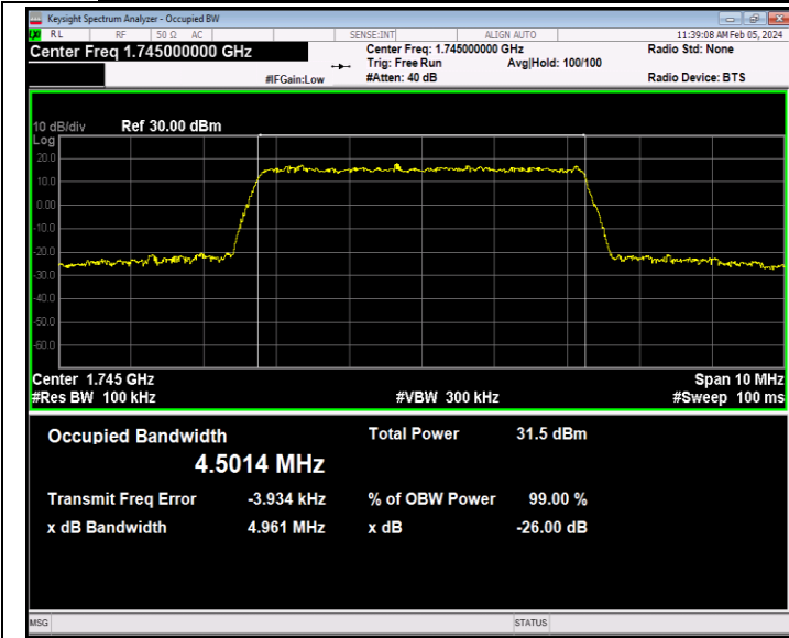
Band66-5MHz-QPSK-132322-25RB#0-PASS
