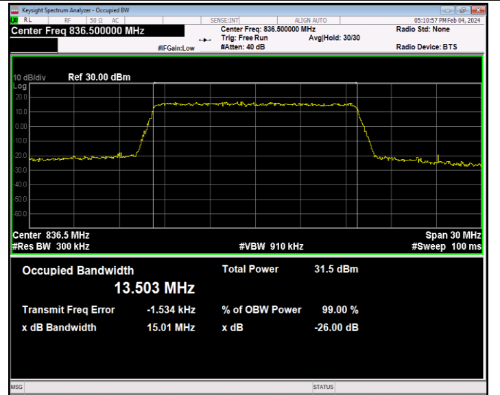
26(824-849)-15MHz-QPSK-26915-75RB#0-PASS
