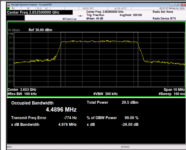
41(2535-2655)-5MHz-16QAM-41215-25RB#0-PASS
