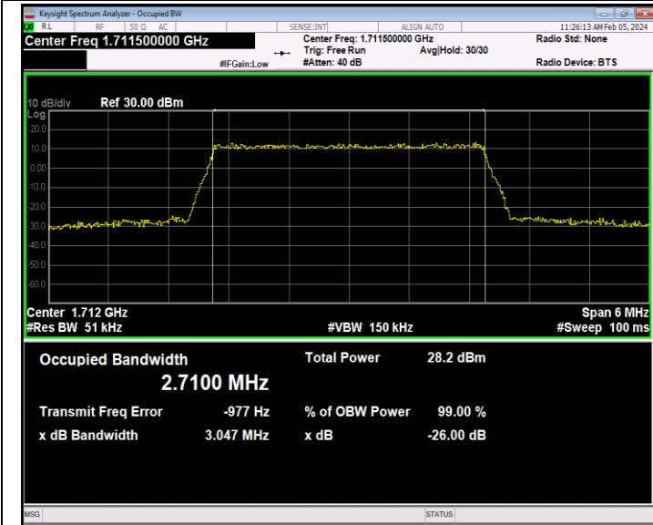
Band66-3MHz-64QAM-131987-15RB#0-PASS
