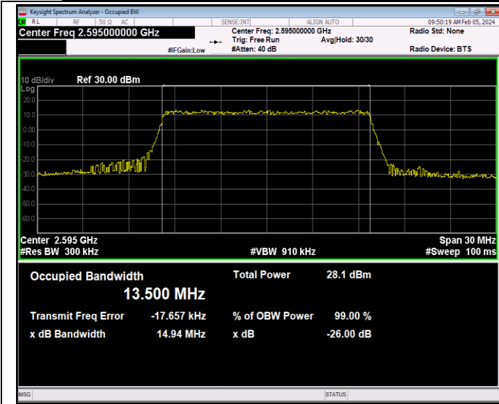
41(2535-2655)-15MHz-64QAM-40640-75RB#0-PASS
