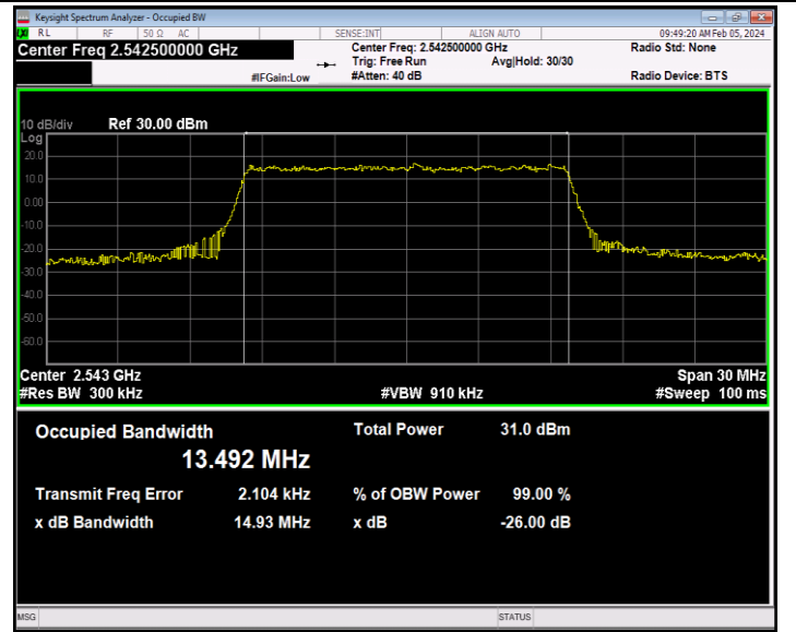
41(2535-2655)-15MHz-QPSK-40115-75RB#0-PASS
