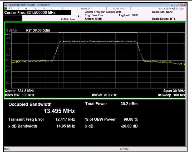
26(824-849)-15MHz-16QAM-26865-75RB#0-PASS
