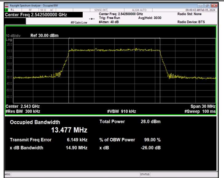
41(2535-2655)-15MHz-64QAM-40115-75RB#0-PASS
