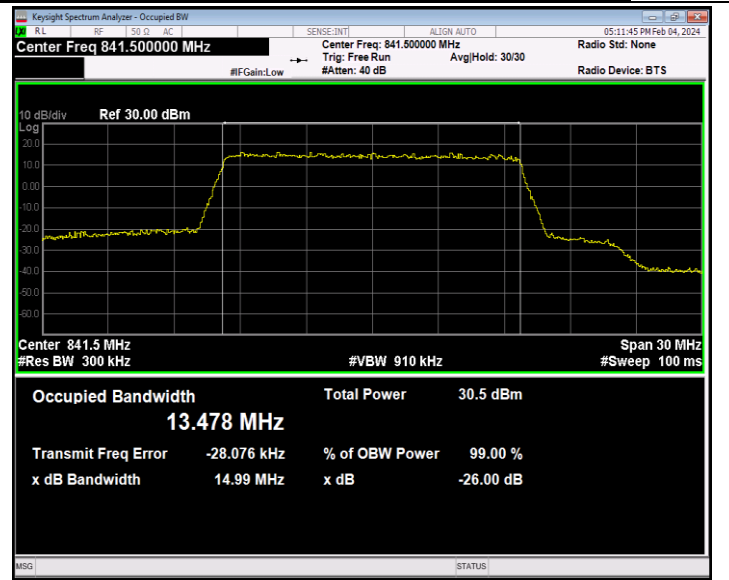
26(824-849)-15MHz-16QAM-26965-75RB#0-PASS
