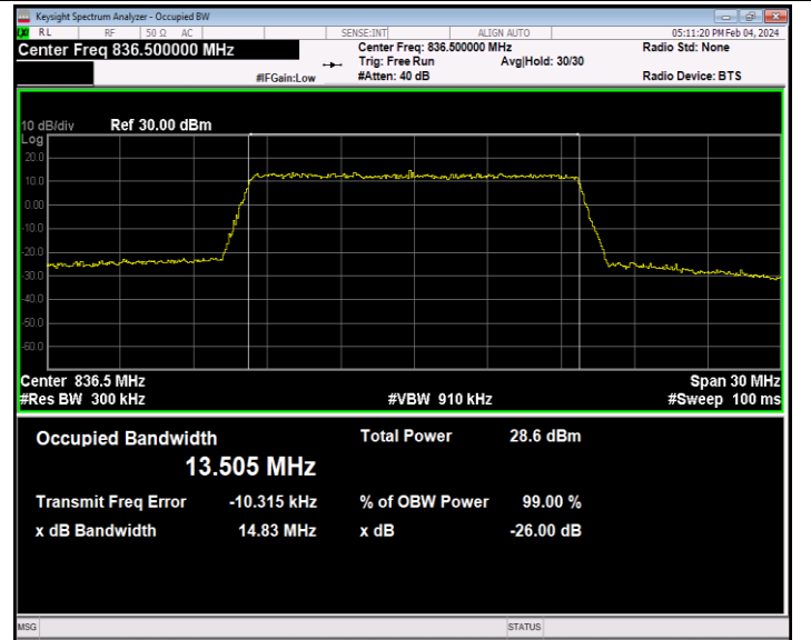
26(824-849)-15MHz-64QAM-26915-75RB#0-PASS
