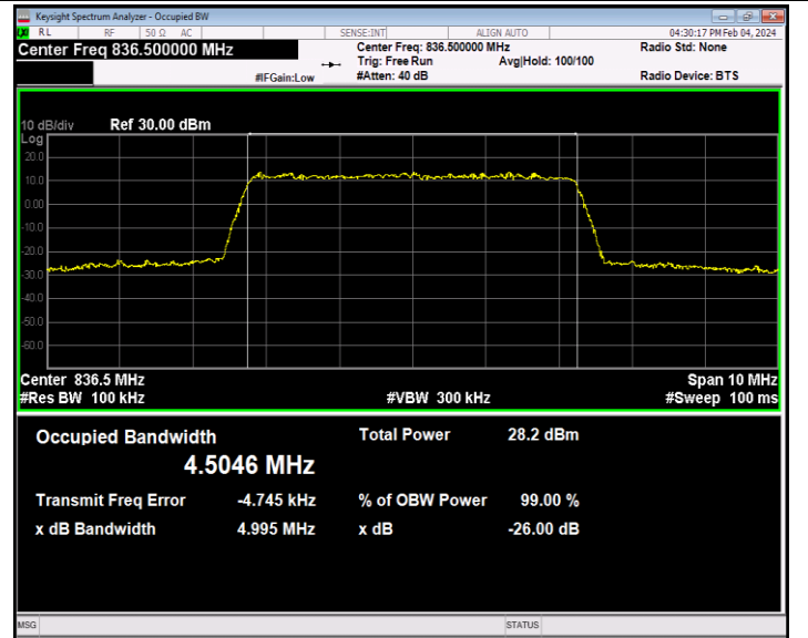
26(824-849)-5MHz-64QAM-26915-25RB#0-PASS
