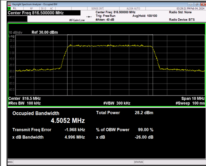
26(814-824)-5MHz-64QAM-26715-25RB#0-PASS
