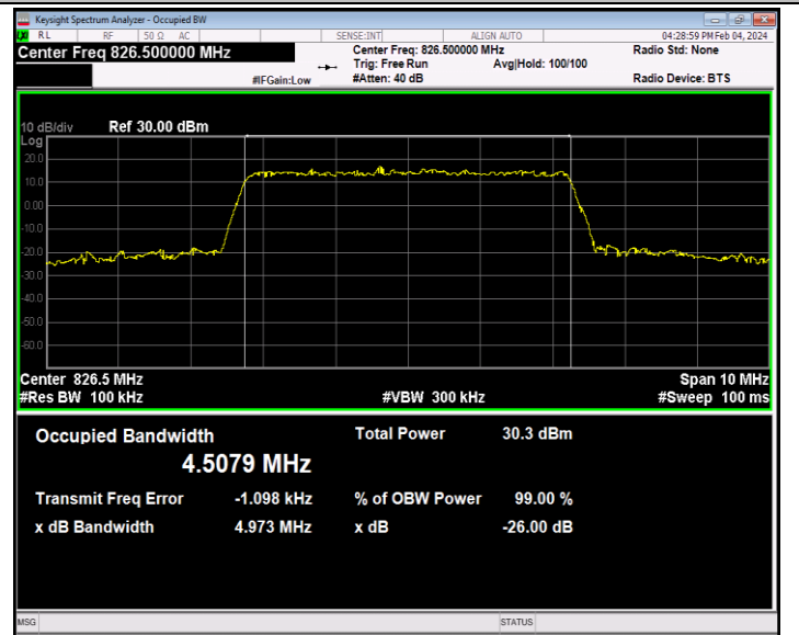
26(824-849)-5MHz-16QAM-26815-25RB#0-PASS
