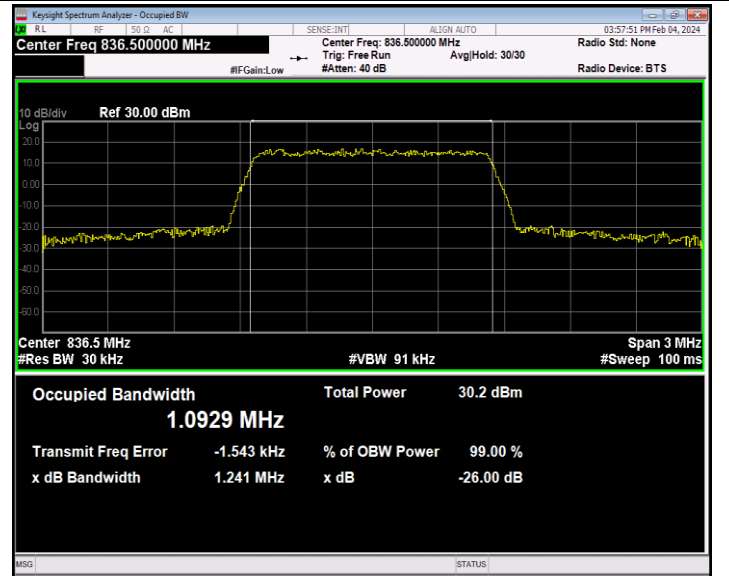
26(824-849)-1.4MHz-QPSK-26915-6RB#0-PASS
