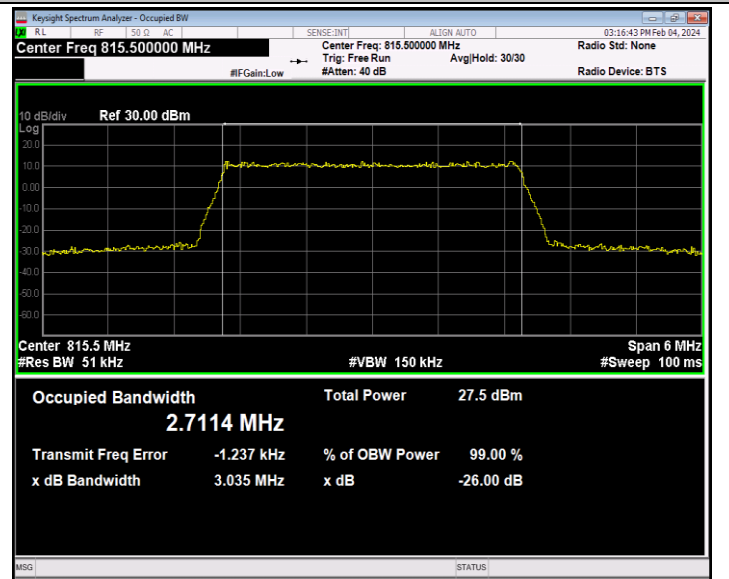
26(814-824)-3MHz-64QAM-26705-15RB#0-PASS
