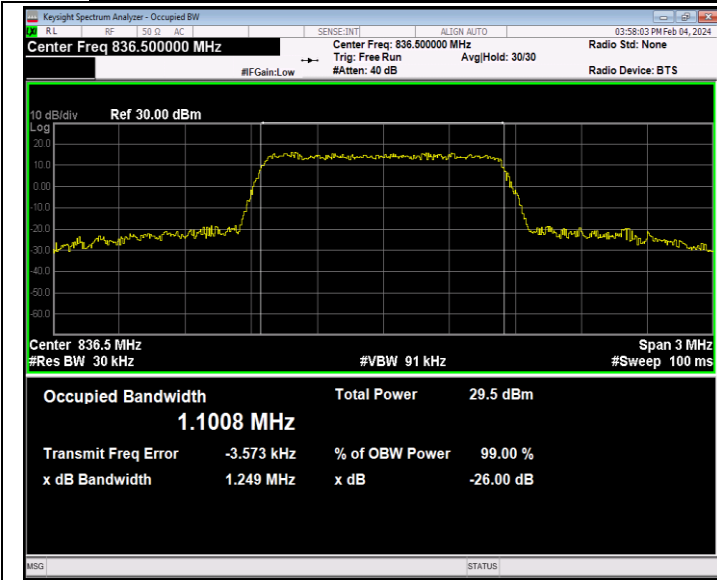
26(824-849)-1.4MHz-16QAM-26915-6RB#0-PASS
