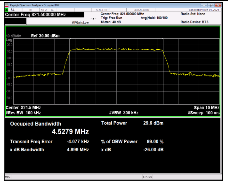
26(814-824)-5MHz-16QAM-26765-25RB#0-PASS
