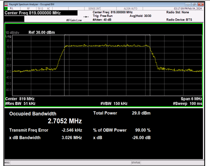
26(814-824)-3MHz-16QAM-26740-15RB#0-PASS
