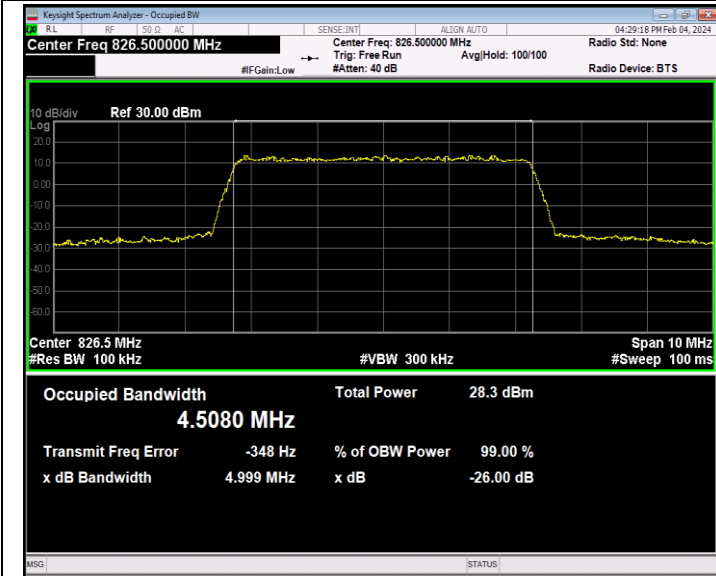
26(824-849)-5MHz-64QAM-26815-25RB#0-PASS
