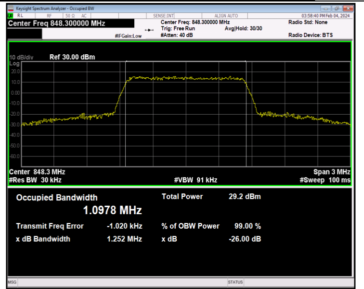
26(824-849)-1.4MHz-16QAM-27033-6RB#0-PASS
