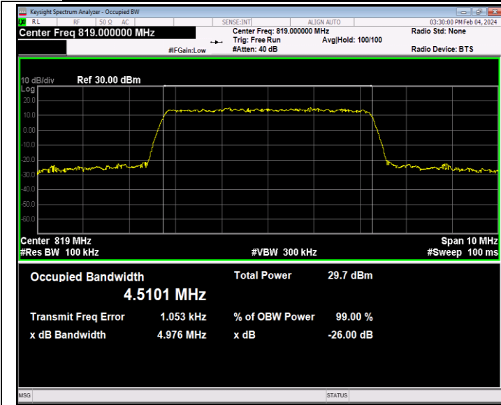
26(814-824)-5MHz-16QAM-26740-25RB#0-PASS
