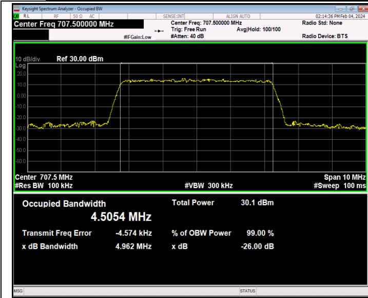
Band12-5MHz-16QAM-23095-25RB#0-PASS
