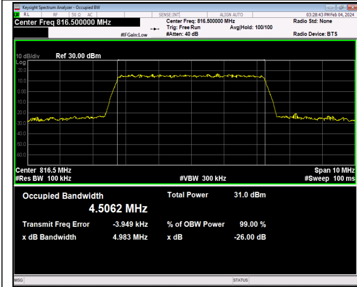
26(814-824)-5MHz-QPSK-26715-25RB#0-PASS
