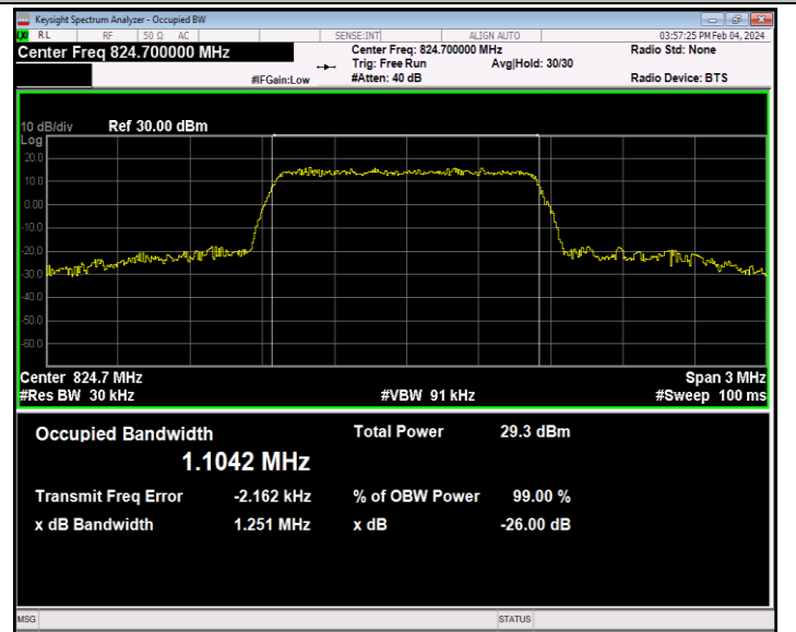
26(824-849)-1.4MHz-16QAM-26797-6RB#0-PASS
