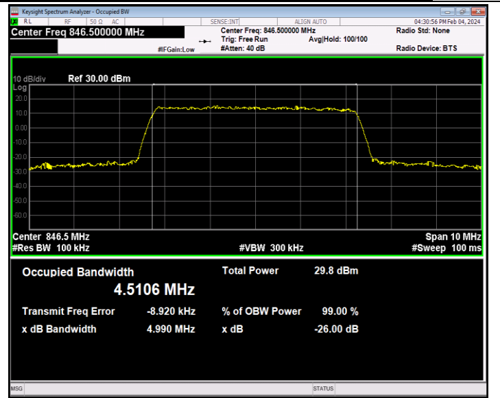
26(824-849)-5MHz-16QAM-27015-25RB#0-PASS
