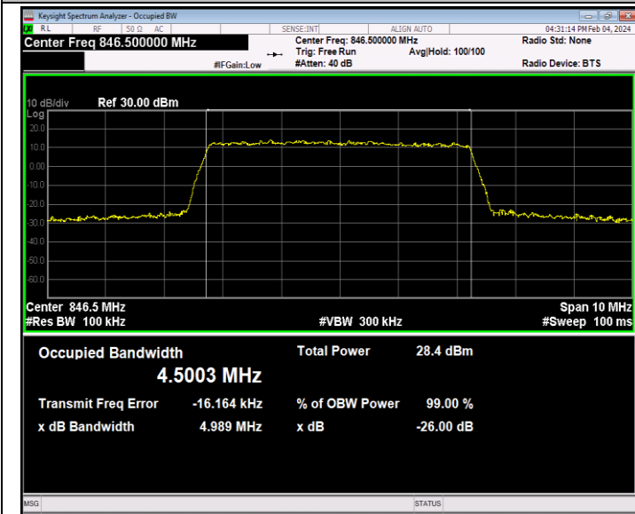
26(824-849)-5MHz-64QAM-27015-25RB#0-PASS
