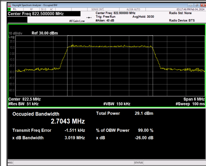
26(814-824)-3MHz-16QAM-26775-15RB#0-PASS
