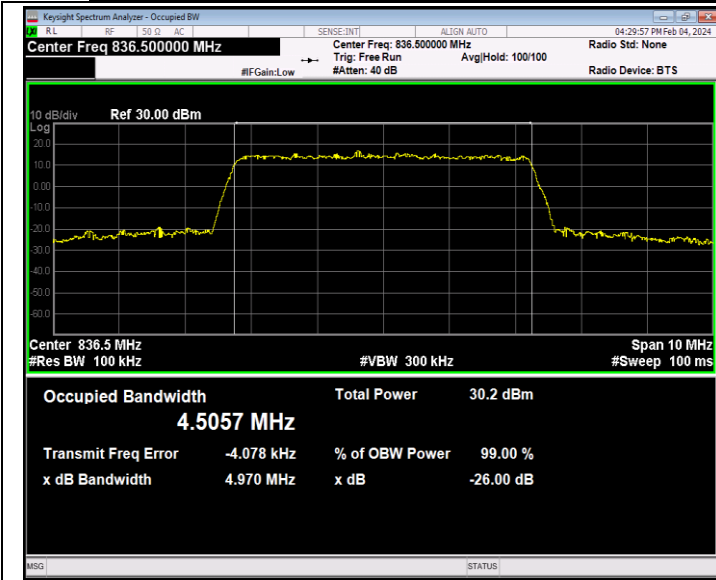
26(824-849)-5MHz-16QAM-26915-25RB#0-PASS
