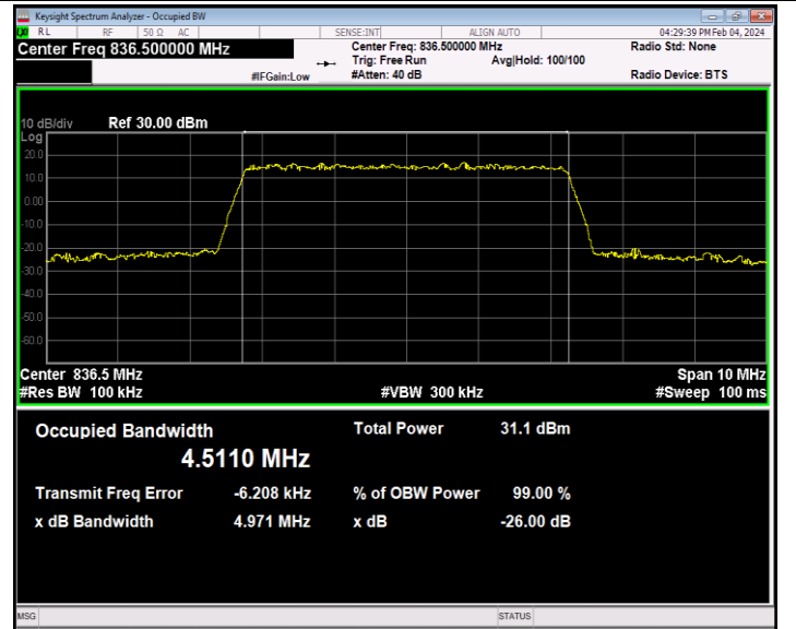
26(824-849)-5MHz-QPSK-26915-25RB#0-PASS
