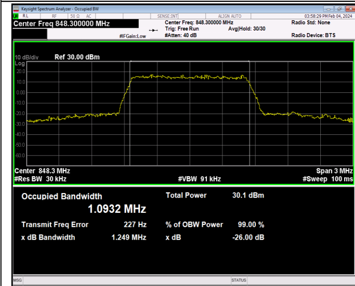
26(824-849)-1.4MHz-QPSK-27033-6RB#0-PASS
