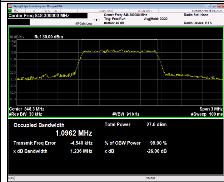
26(824-849)-1.4MHz-64QAM-27033-6RB#0-PASS
