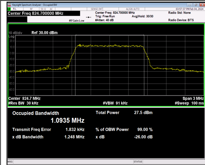
26(824-849)-1.4MHz-64QAM-26797-6RB#0-PASS
