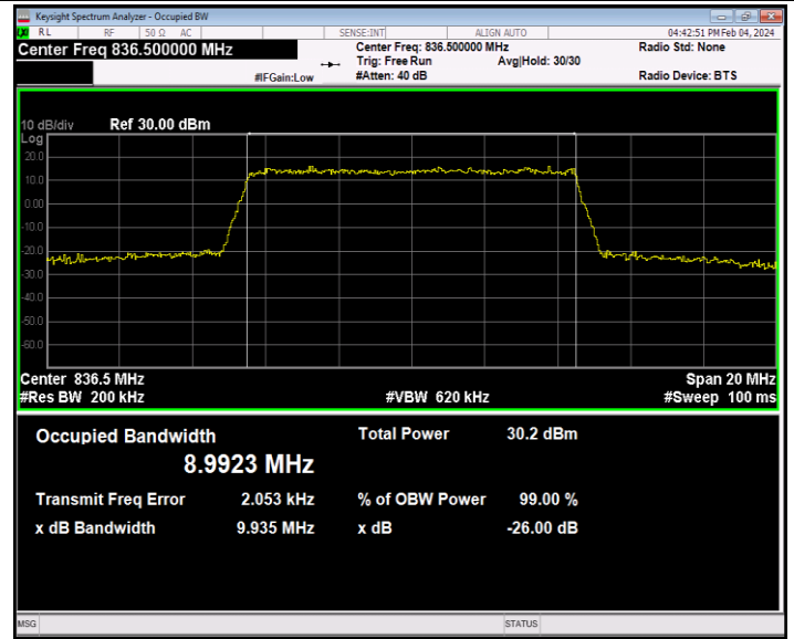
26(824-849)-10MHz-16QAM-26915-50RB#0-PASS
