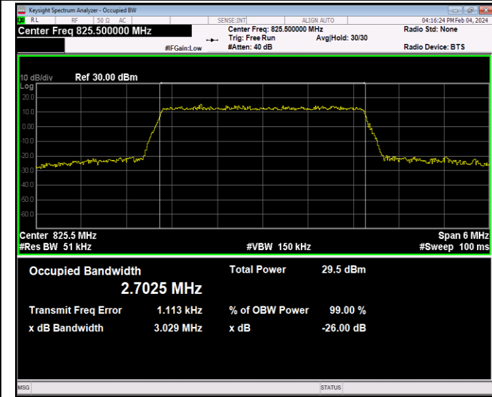
26(824-849)-3MHz-16QAM-26805-15RB#0-PASS
