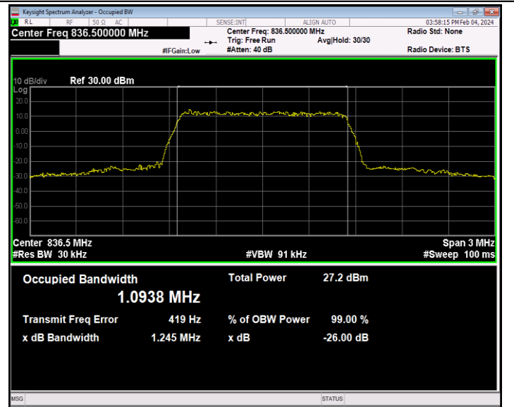
26(824-849)-1.4MHz-64QAM-26915-6RB#0-PASS
