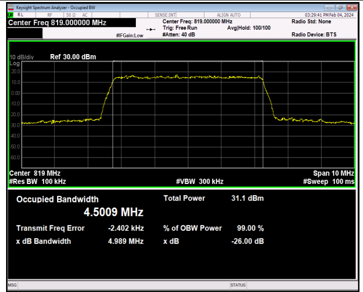
26(814-824)-5MHz-QPSK-26740-25RB#0-PASS
