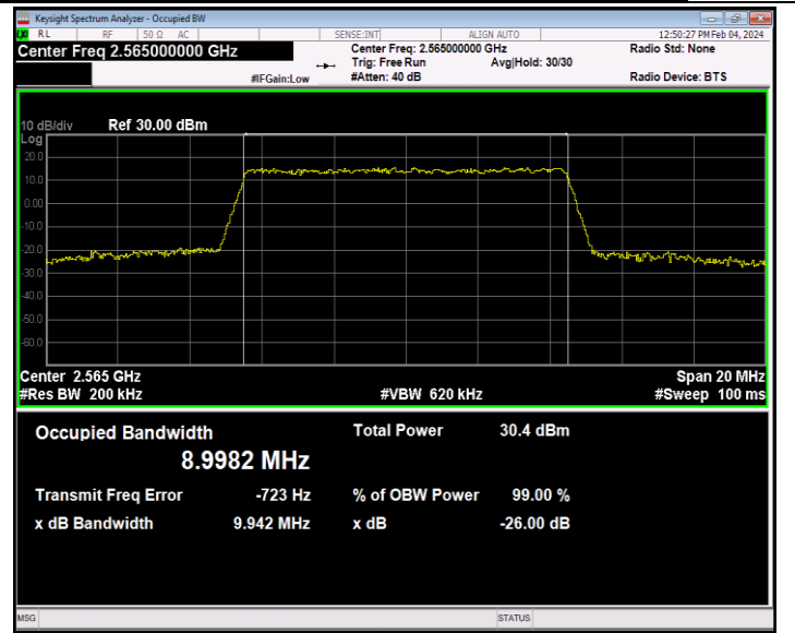
Band7-10MHz-64QAM-21400-50RB#0-PASS
