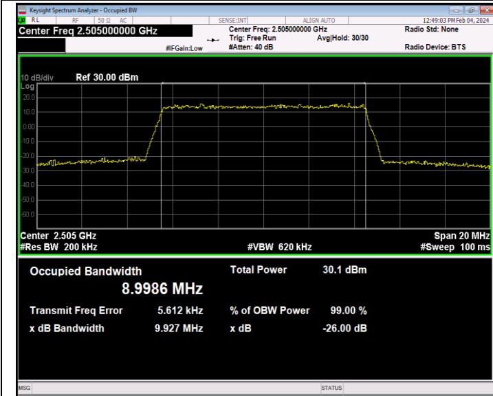
Band7-10MHz-16QAM-20800-50RB#0-PASS
