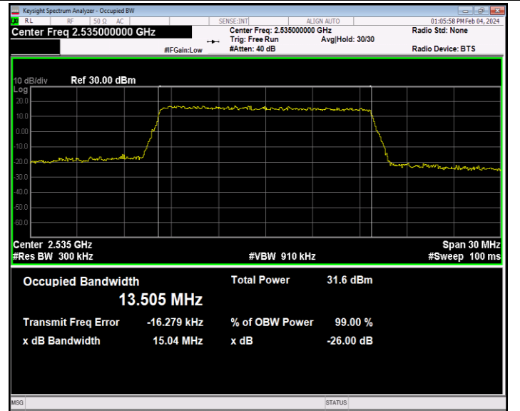
Band7-15MHz-QPSK-21100-75RB#0-PASS
