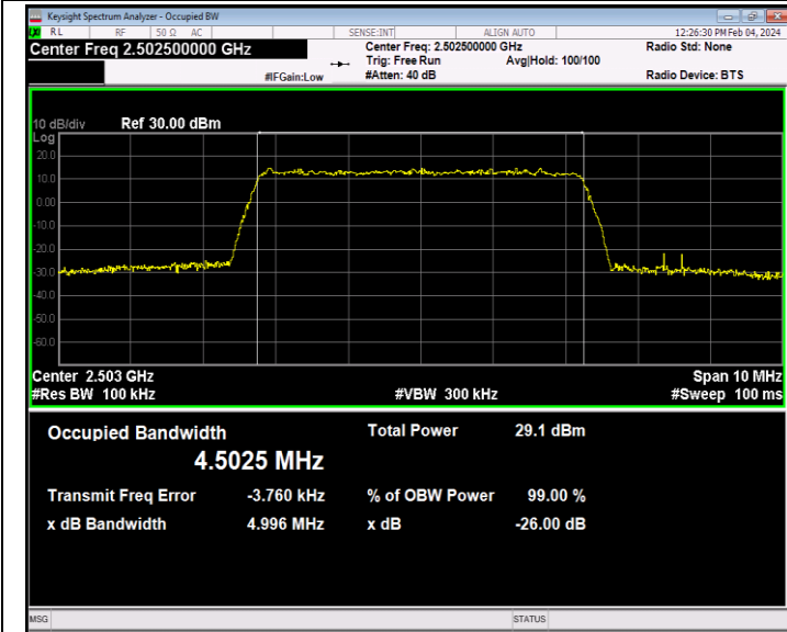
Band7-5MHz-64QAM-20775-25RB#0-PASS
