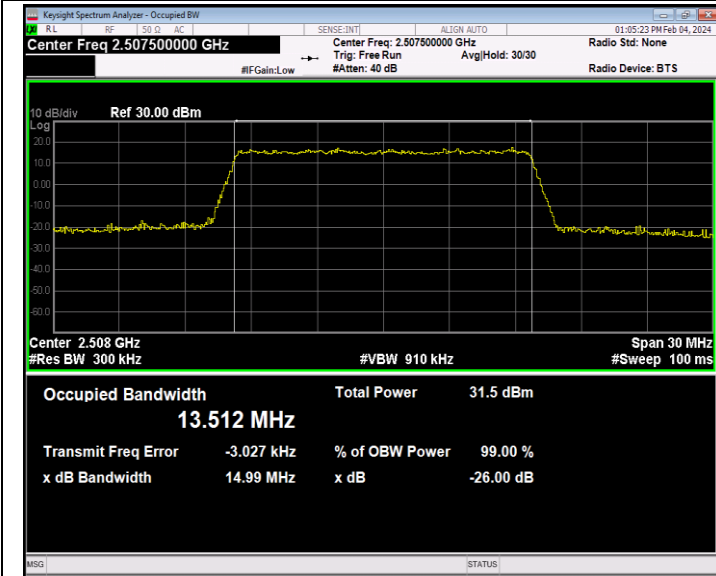
Band7-15MHz-QPSK-20825-75RB#0-PASS
