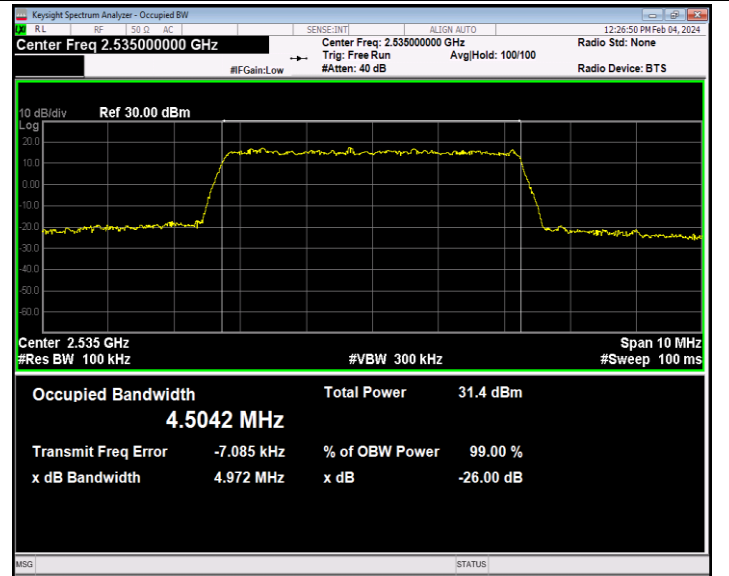
Band7-5MHz-QPSK-21100-25RB#0-PASS
