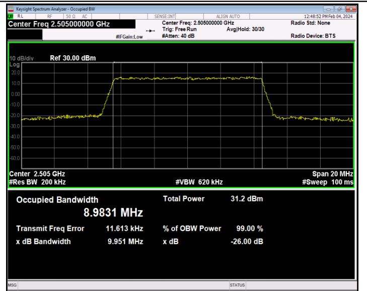
Band7-10MHz-QPSK-20800-50RB#0-PASS
