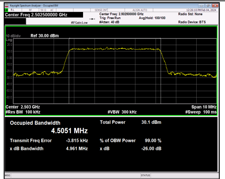
Band7-5MHz-16QAM-20775-25RB#0-PASS
