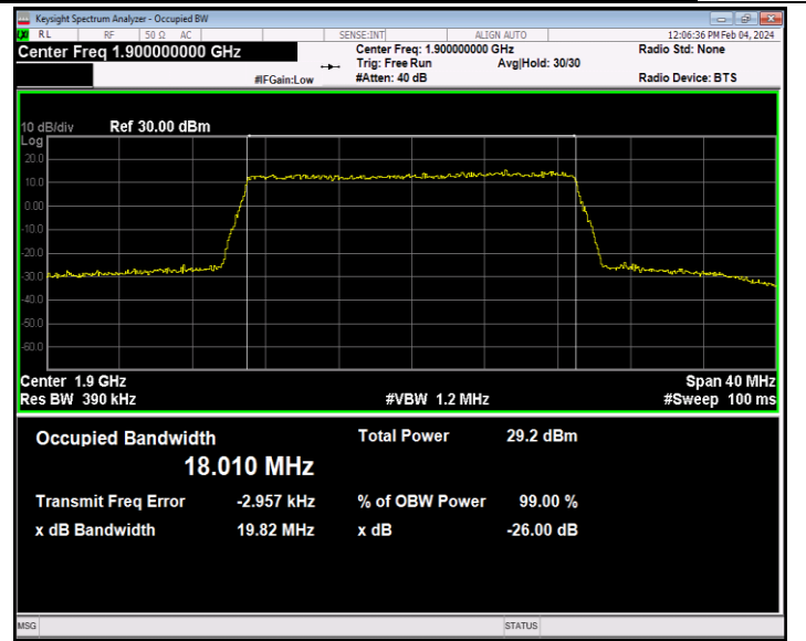
Band2-20MHz-64QAM-19100-100RB#0-PASS
