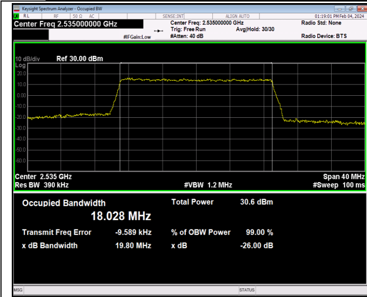
Band7-20MHz-64QAM-21100-100RB#0-PASS
