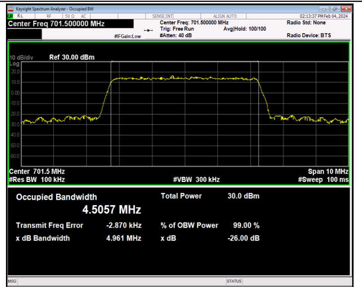
Band12-5MHz-16QAM-23035-25RB#0-PASS
