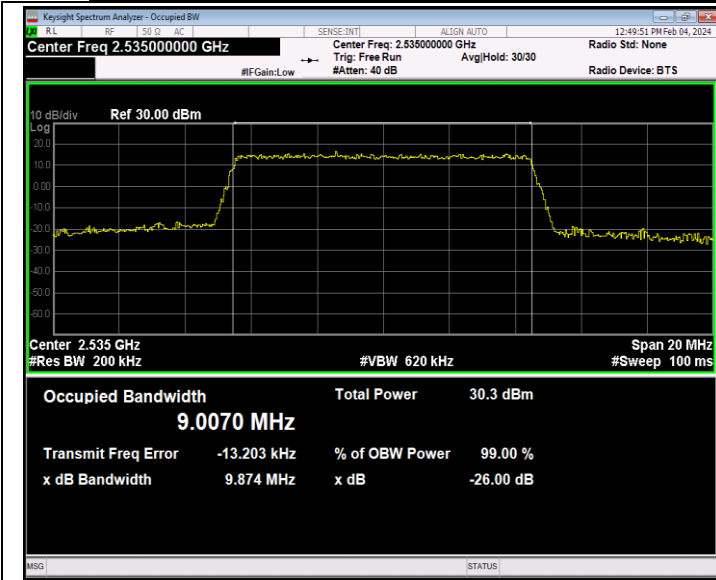
Band7-10MHz-64QAM-21100-50RB#0-PASS
