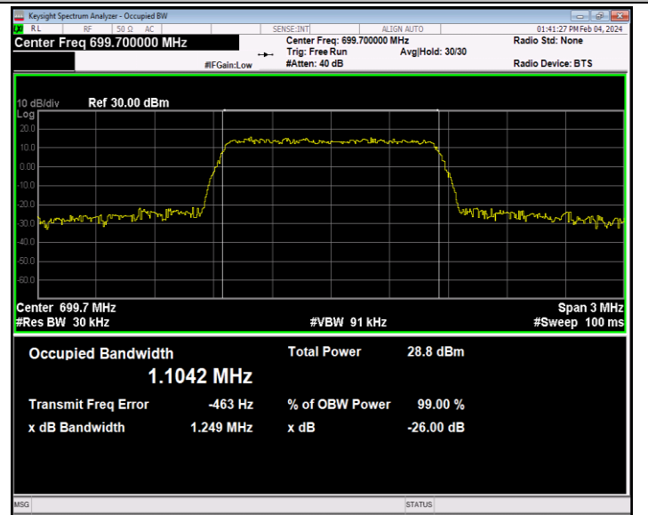
Band12-1.4MHz-16QAM-23017-6RB#0-PASS
