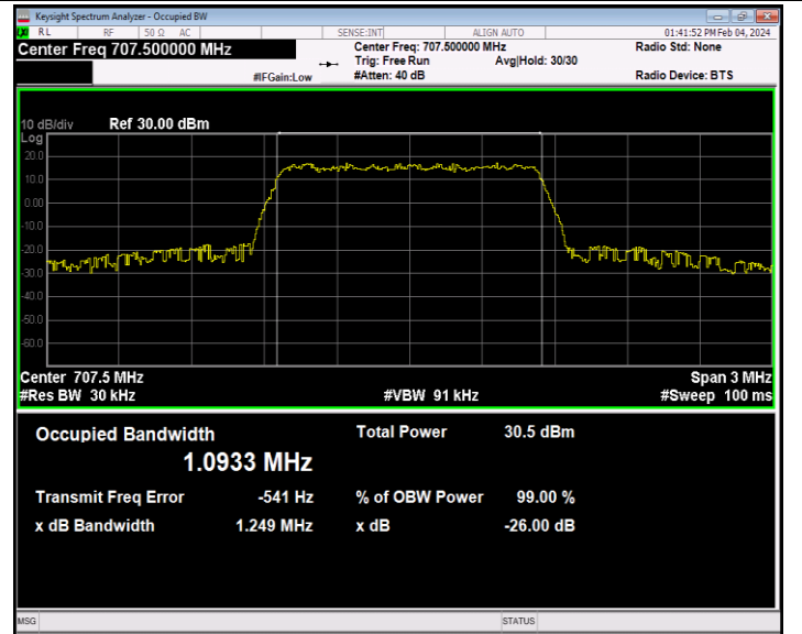
Band12-1.4MHz-QPSK-23095-6RB#0-PASS
