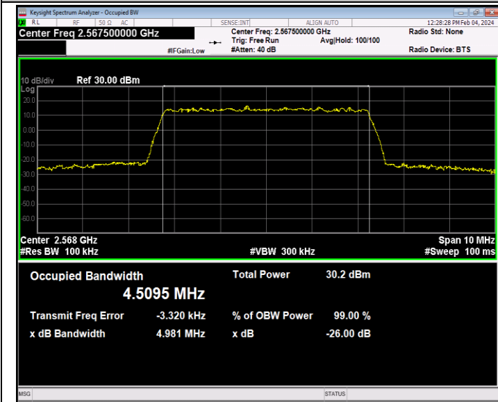
Band7-5MHz-64QAM-21425-25RB#0-PASS
