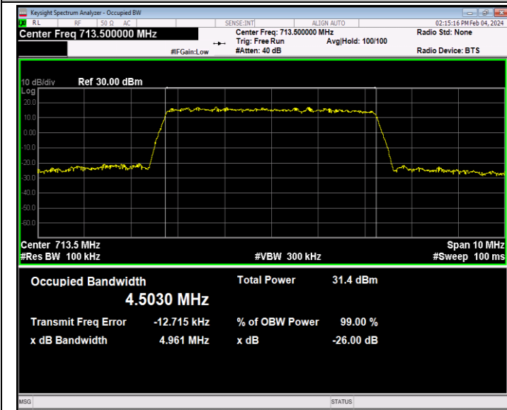
Band12-5MHz-QPSK-23155-25RB#0-PASS
