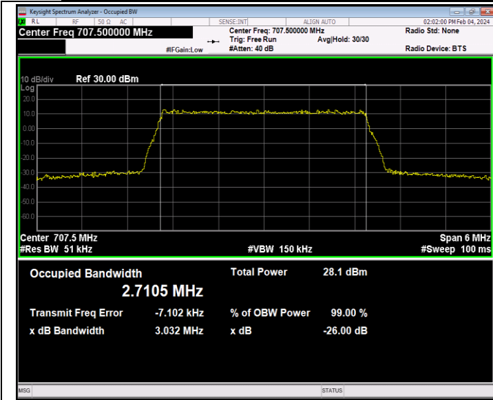
Band12-3MHz-64QAM-23095-15RB#0-PASS
