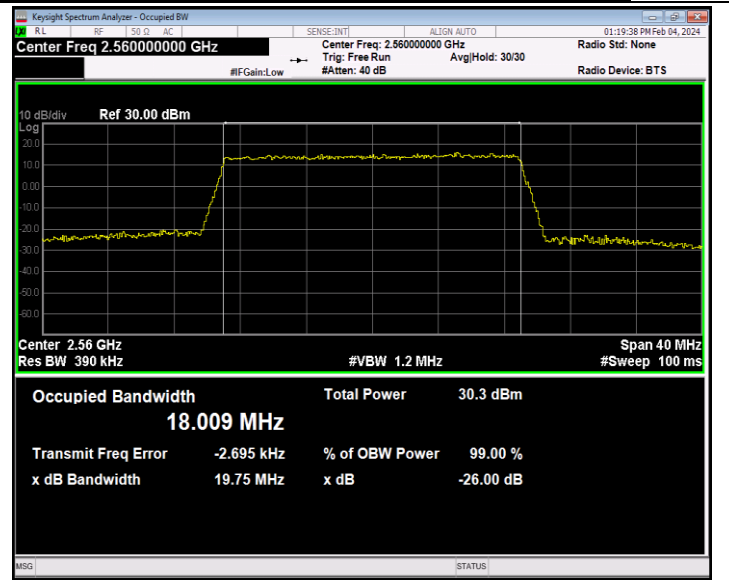
Band7-20MHz-64QAM-21350-100RB#0-PASS
