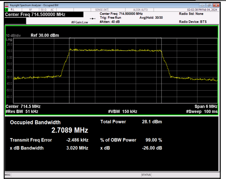
Band12-3MHz-64QAM-23165-15RB#0-PASS
