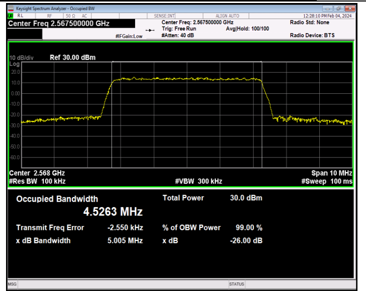
Band7-5MHz-16QAM-21425-25RB#0-PASS
