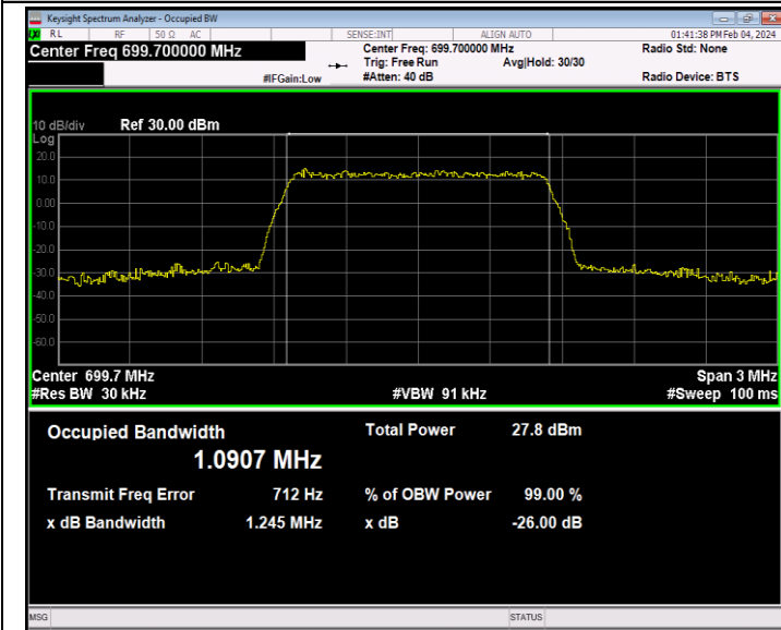
Band12-1.4MHz-64QAM-23017-6RB#0-PASS
