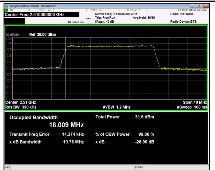
Band7-20MHz-QPSK-20850-100RB#0-PASS
