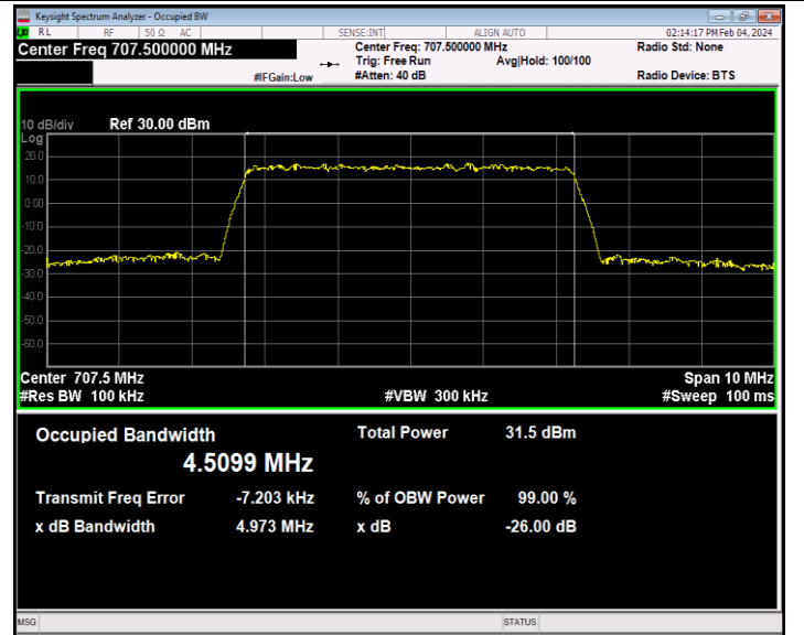
Band12-5MHz-QPSK-23095-25RB#0-PASS
