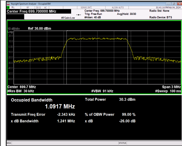
Band12-1.4MHz-QPSK-23017-6RB#0-PASS
