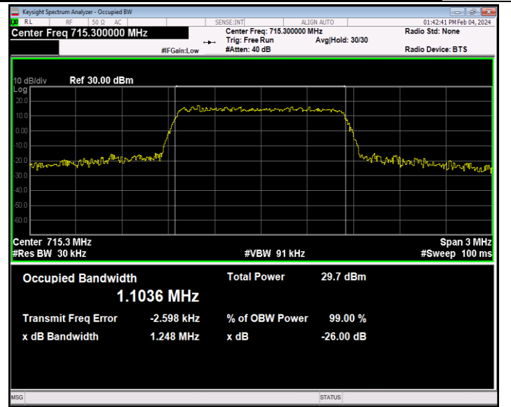
Band12-1.4MHz-16QAM-23173-6RB#0-PASS
