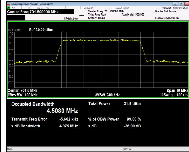
Band12-5MHz-QPSK-23035-25RB#0-PASS
