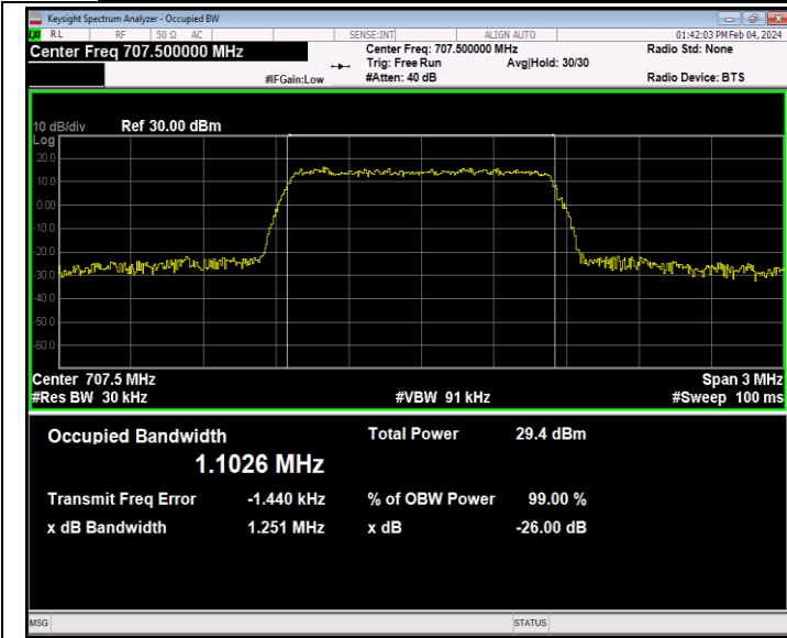
Band12-1.4MHz-16QAM-23095-6RB#0-PASS
