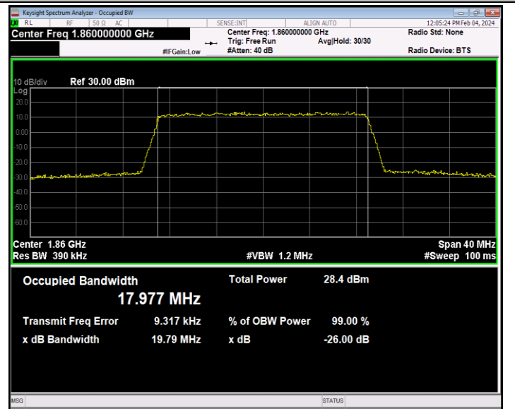
Band2-20MHz-64QAM-18700-100RB#0-PASS
