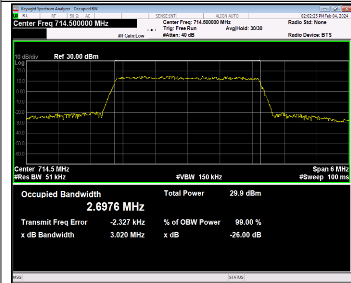
Band12-3MHz-16QAM-23165-15RB#0-PASS
