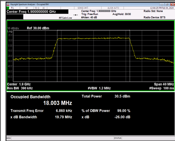
Band2-20MHz-16QAM-19100-100RB#0-PASS
