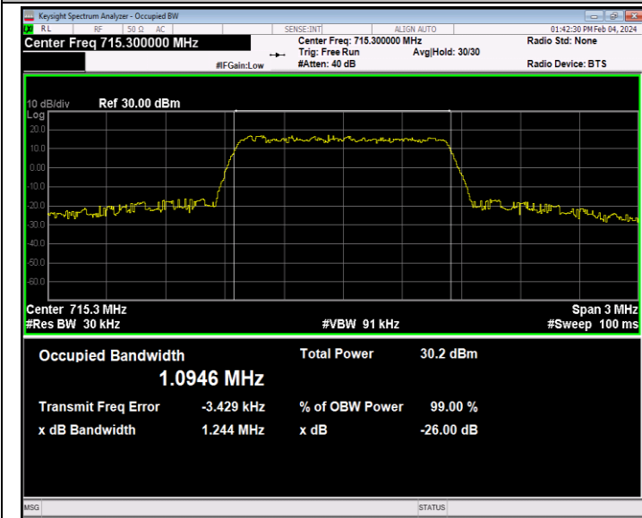
Band12-1.4MHz-QPSK-23173-6RB#0-PASS
