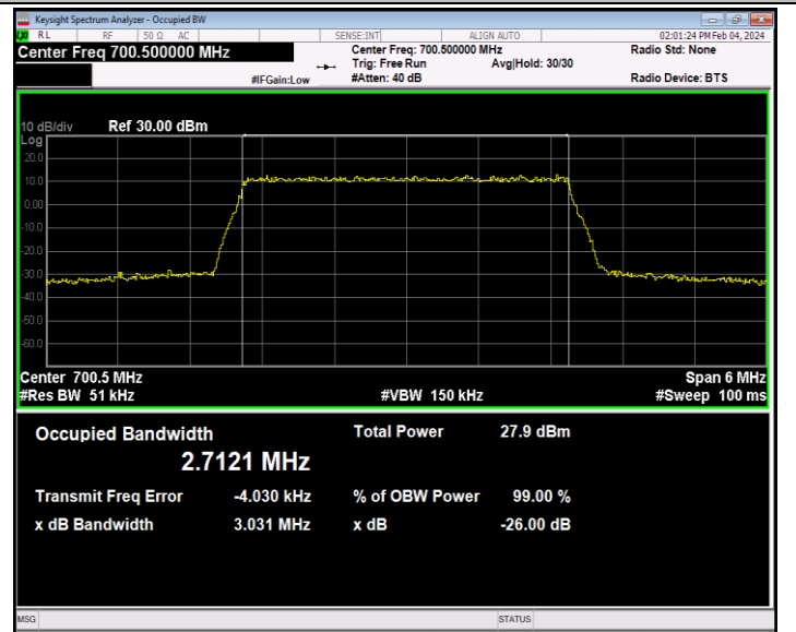
Band12-3MHz-64QAM-23025-15RB#0-PASS
