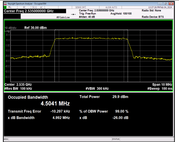
Band7-5MHz-64QAM-21100-25RB#0-PASS
