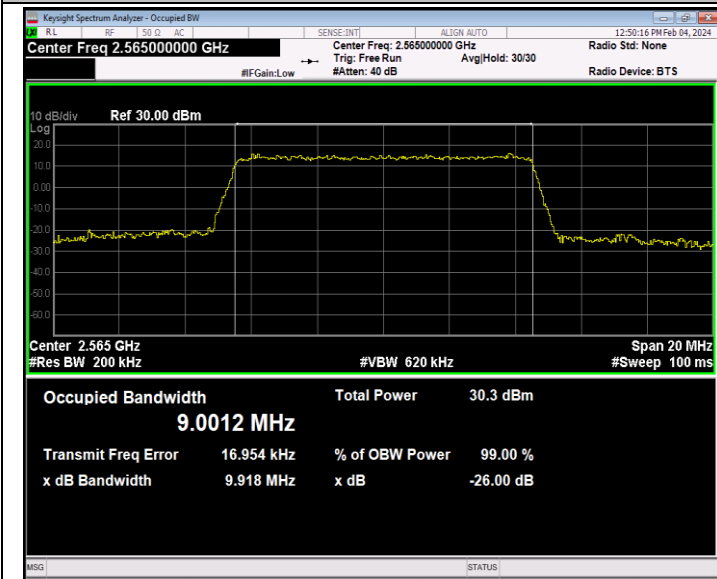
Band7-10MHz-16QAM-21400-50RB#0-PASS
