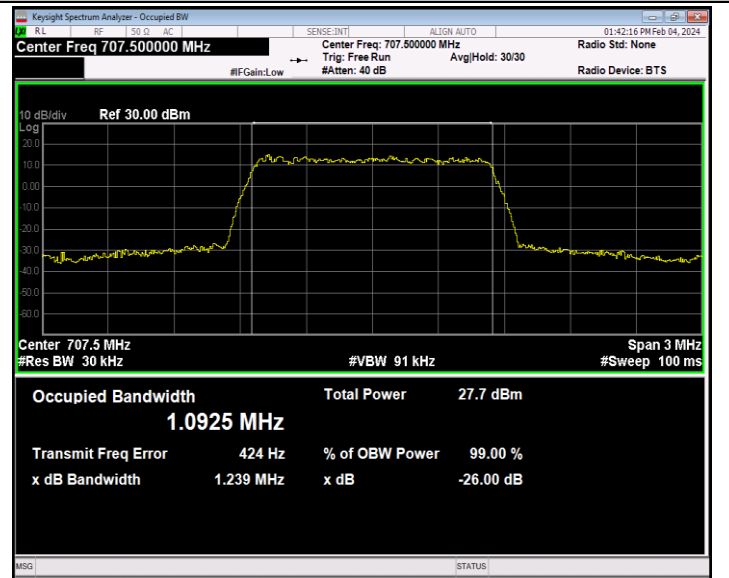
Band12-1.4MHz-64QAM-23095-6RB#0-PASS
