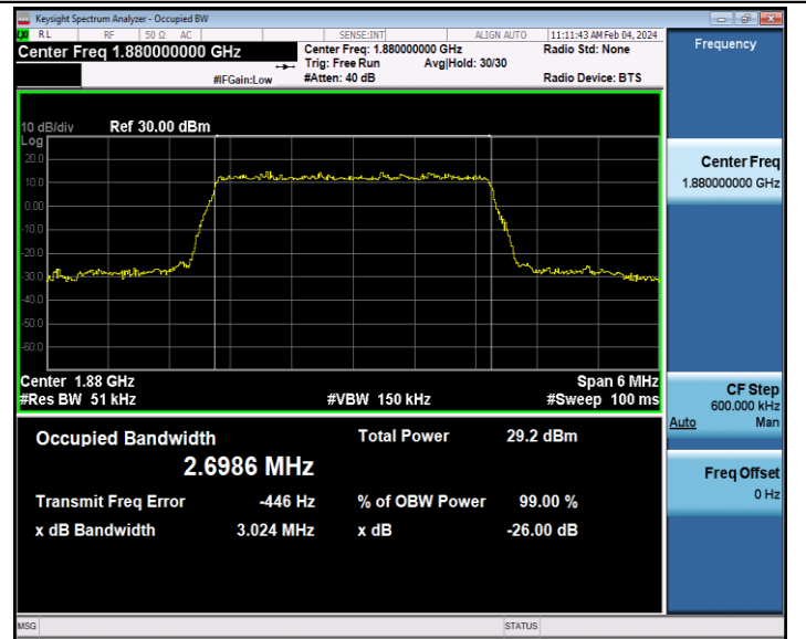
Band2-3MHz-16QAM-18900-15RB#0-PASS
