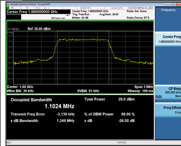
Band2-1.4MHz-16QAM-18900-6RB#0-PASS
