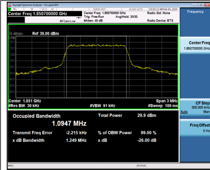
Band2-1.4MHz-QPSK-18607-6RB#0-PASS
