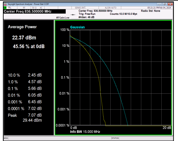
26(824-849)-15MHz-QPSK-26915-75RB#0-PASS
