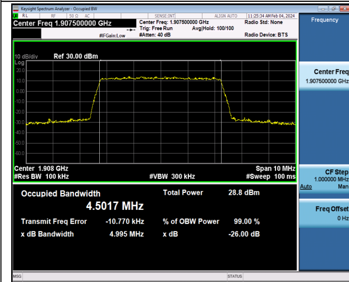
Band2-5MHz-64QAM-19175-25RB#0-PASS
