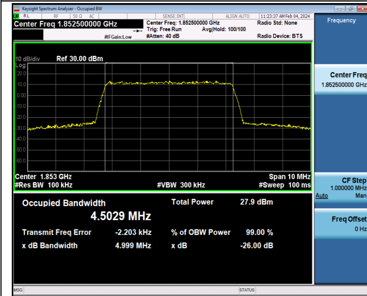
Band2-5MHz-64QAM-18625-25RB#0-PASS
