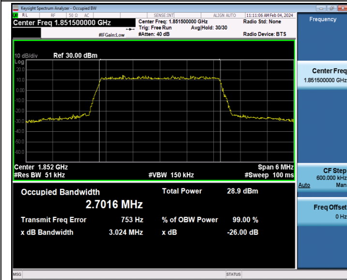
Band2-3MHz-16QAM-18615-15RB#0-PASS
