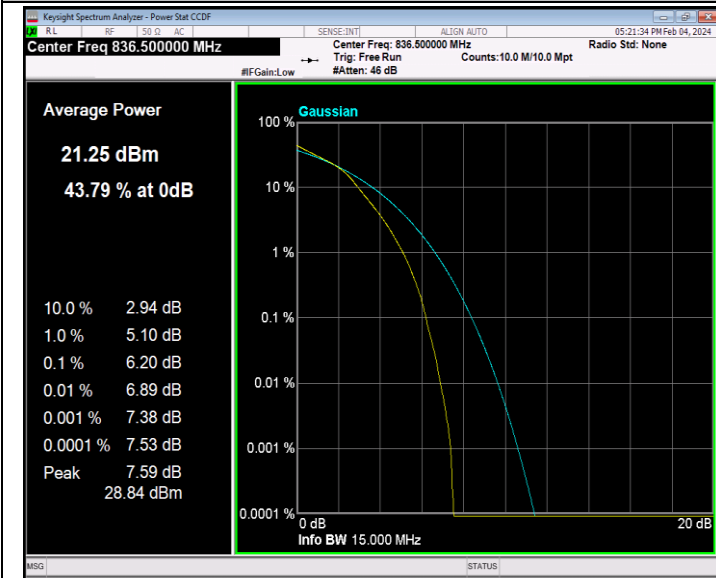
26(824-849)-15MHz-16QAM-26915-75RB#0-PASS
