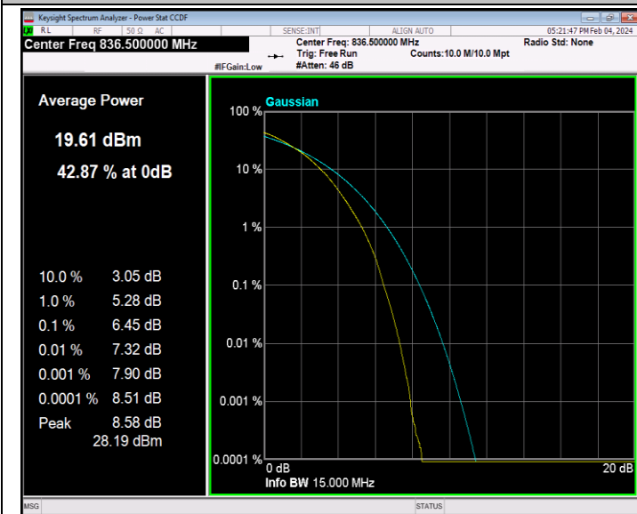
26(824-849)-15MHz-64QAM-26915-75RB#0-PASS
