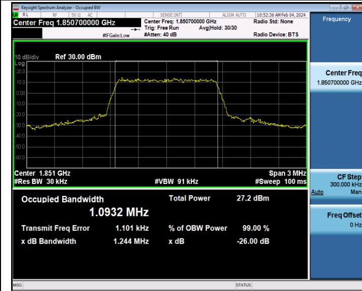
Band2-1.4MHz-16QAM-18507-6RB#0-PASS
