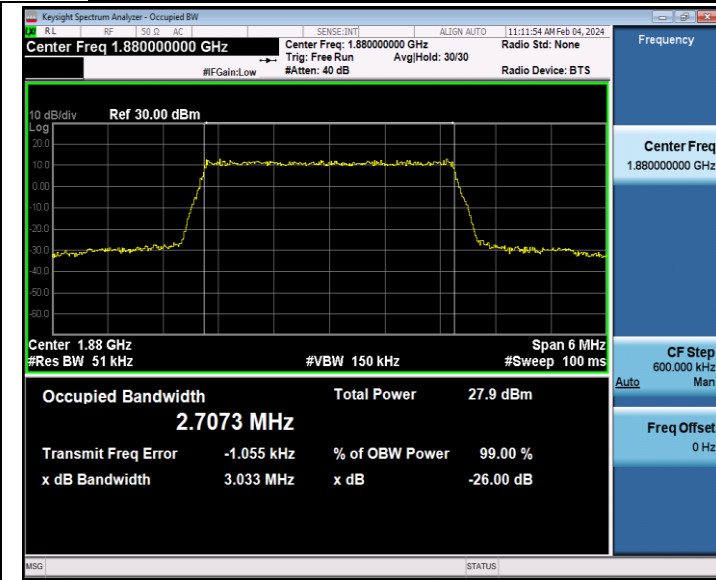
Band2-3MHz-64QAM-18900-15RB#0-PASS
