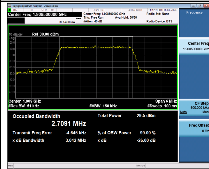
Band2-3MHz-16QAM-19185-15RB#0-PASS
