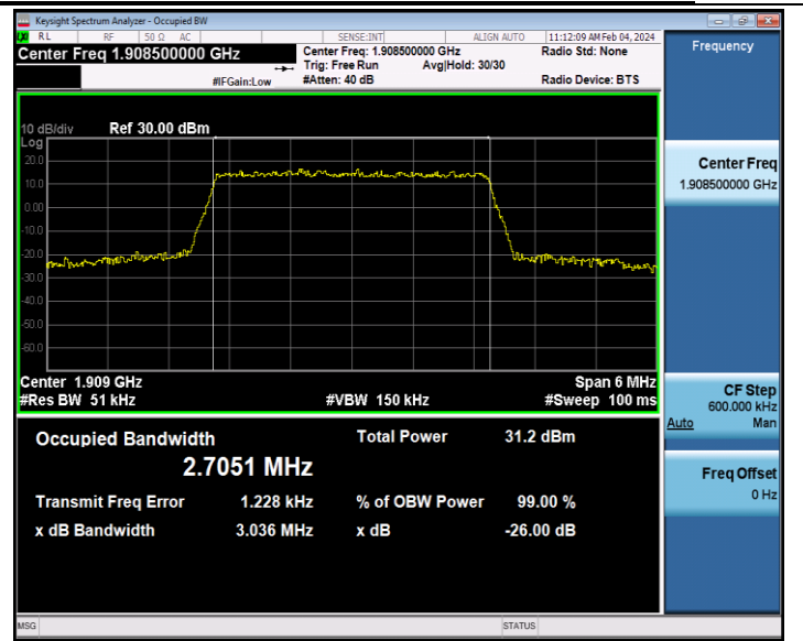
Band2-3MHz-QPSK-19185-15RB#0-PASS
