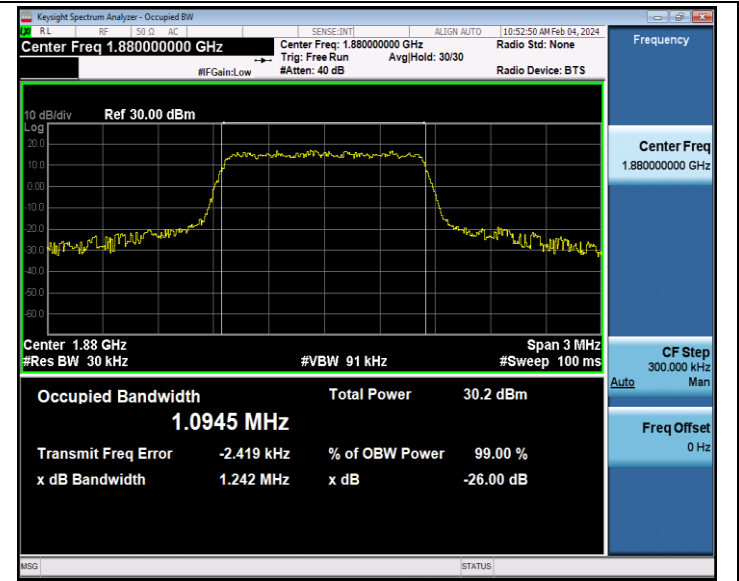
Band2-1.4MHz-QPSK-18900-6RB#0-PASS
