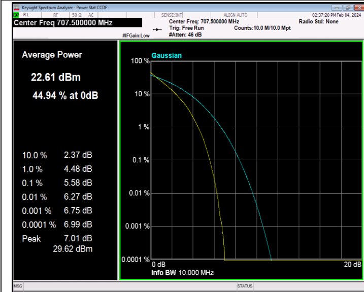
Band12-10MHz-QPSK-23095-50RB#0-PASS
