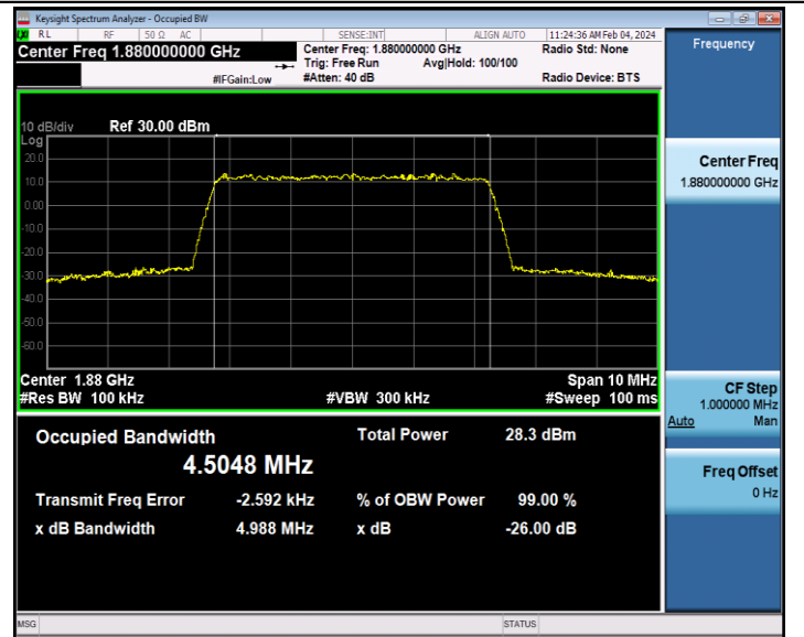
Band2-5MHz-64QAM-18900-25RB#0-PASS
