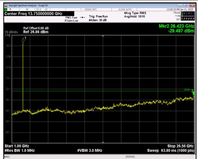
Band38-5MHz-16QAM-38000-1RB#0-Range2:1000~ 26500MHz
