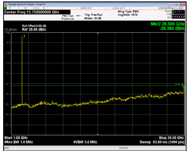
Band38-5MHz-16QAM-37775-1RB#0-Range2:1000~ 26500MHz
