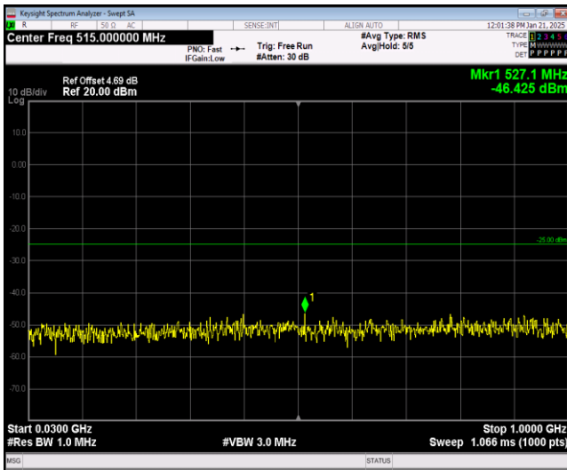
Band38-5MHz-64QAM-38225-1RB#0-Range1:30~1000MHz
