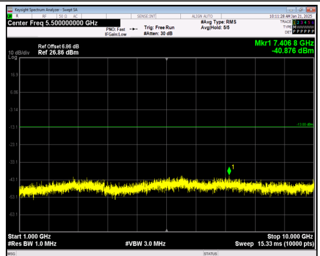
Band17-5MHz-QPSK-23825-1RB#0-Range2:1000~1 0000MHz
