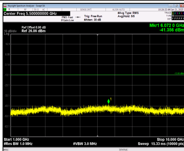
Band17-10MHz-16QAM-23780-1RB#0-Range2:1000~10000MHz
