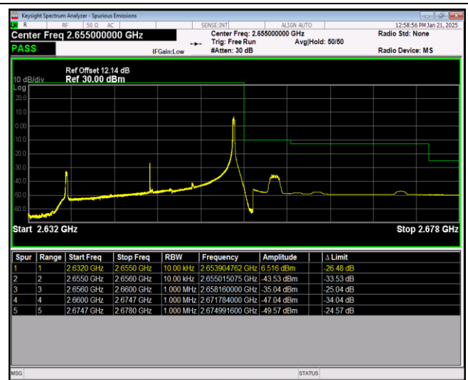
Band41-20MHz-16QAM-40140-1RB#0
