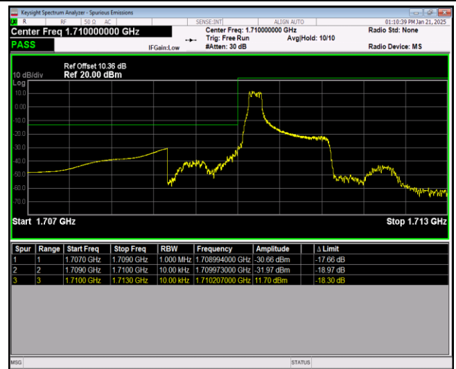
Band66-1.4MHz-16QAM-131979-6RB#0
