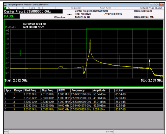
Band41-20MHz-16QAM-40140-100RB#0
