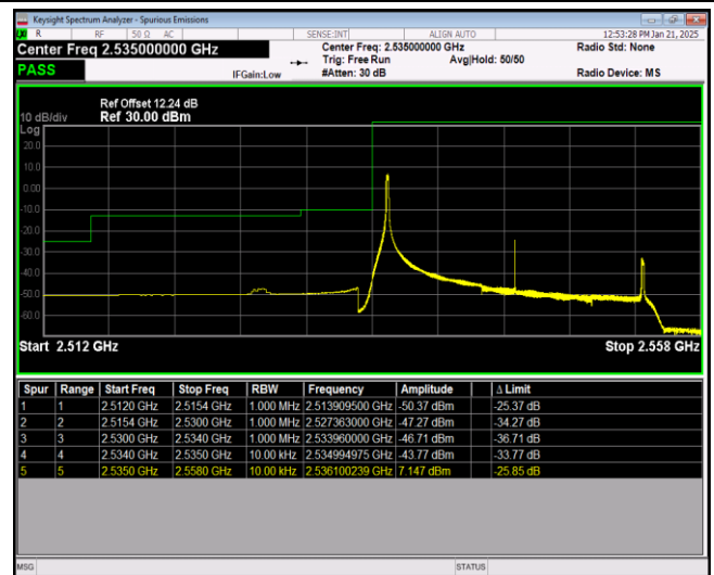
Band41-20MHz-64QAM-40140-100RB#0
