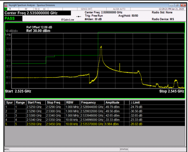
Band41-5MHz-64QAM-40065-25RB#0
