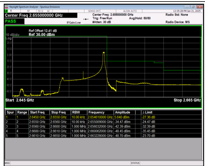
Band41-20MHz-QPSK-40140-1RB#0
