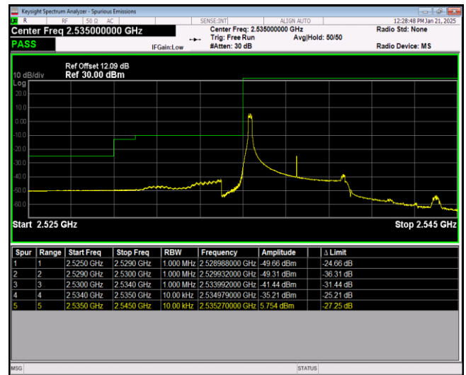
Band41-5MHz-16QAM-40065-25RB#0
