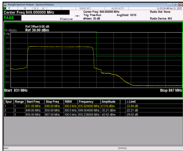
Band26-15MHz-16QAM-26865-1RB#74
