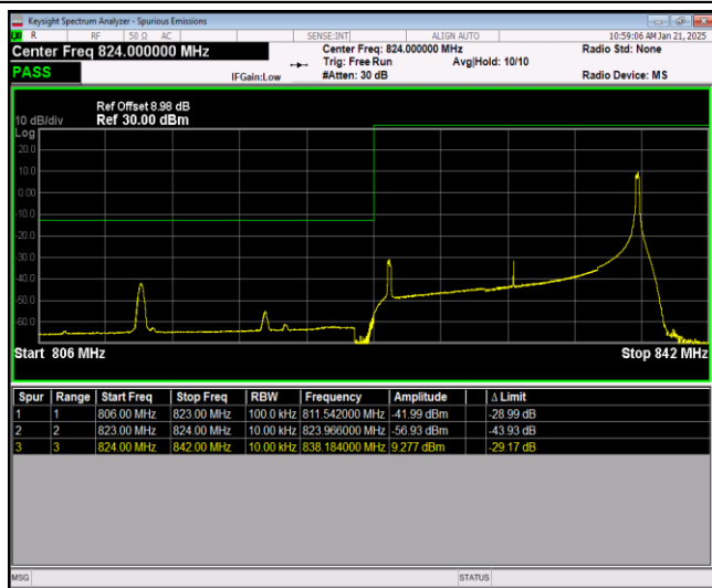
Band26-15MHz-64QAM-26965-1RB#0
