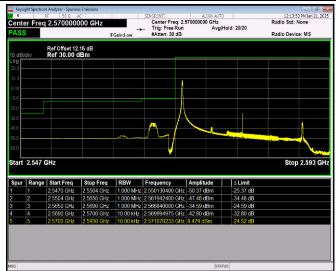
Band38-20MHz-QPSK-37850-100RB#0
