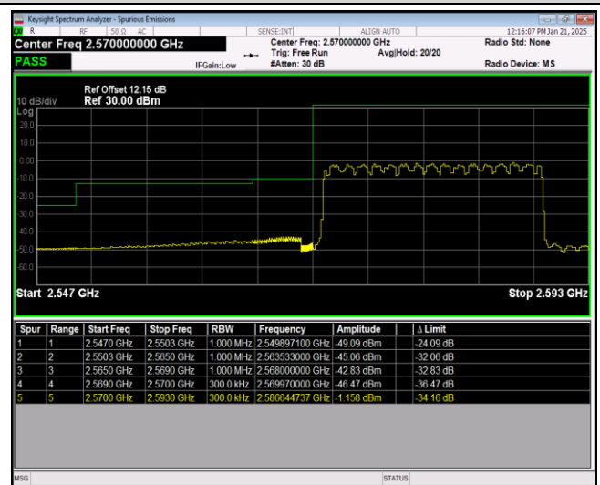
Band38-20MHz-16QAM-38150-1RB#99
