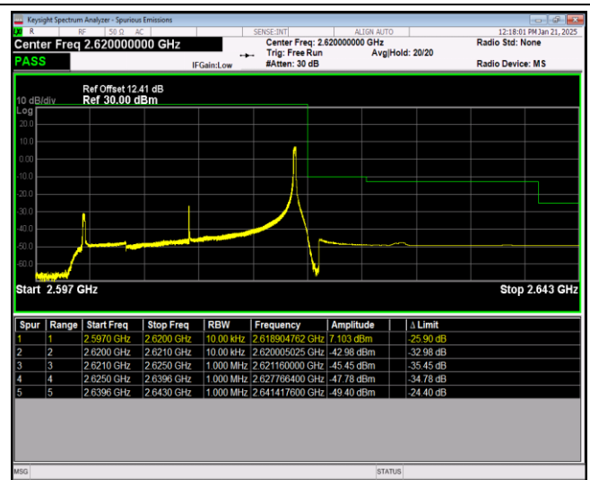
Band38-20MHz-64QAM-37850-1RB#0
