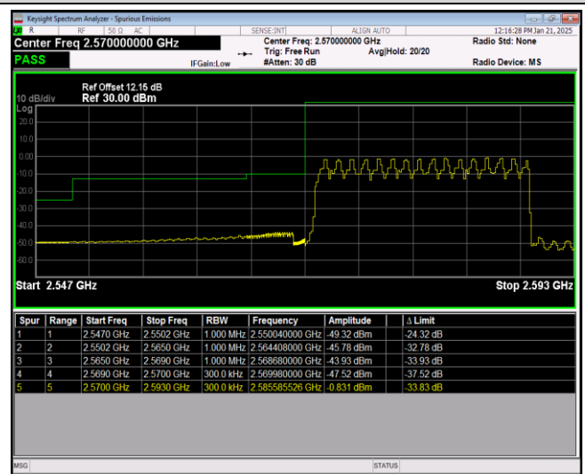
Band38-20MHz-64QAM-38150-1RB#99
