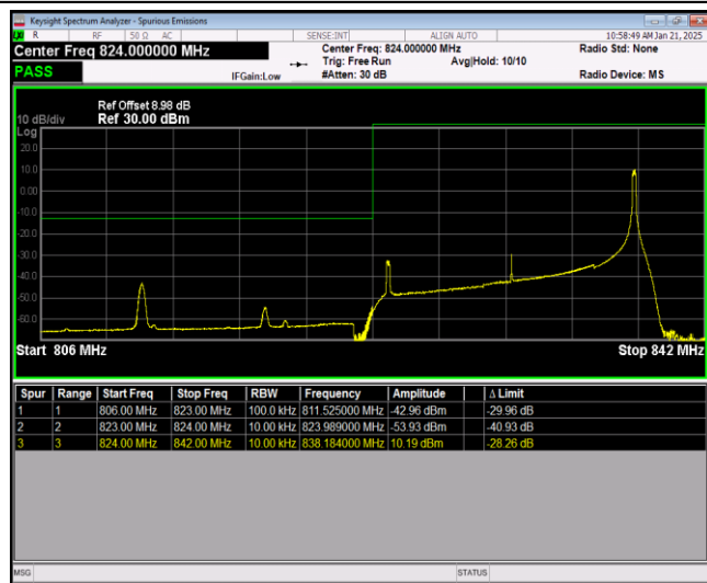
Band26-15MHz-16QAM-26965-1RB#0
