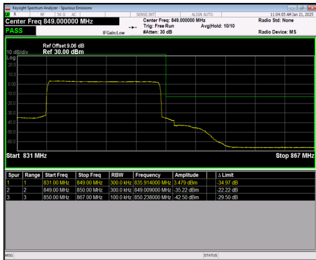
Band26-15MHz-64QAM-26865-1RB#74
