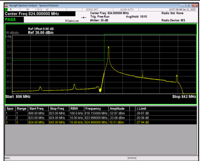
Band26-15MHz-QPSK-26865-75RB#0
