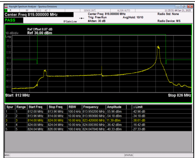
Band26-15MHz-QPSK-26865-1RB#0
