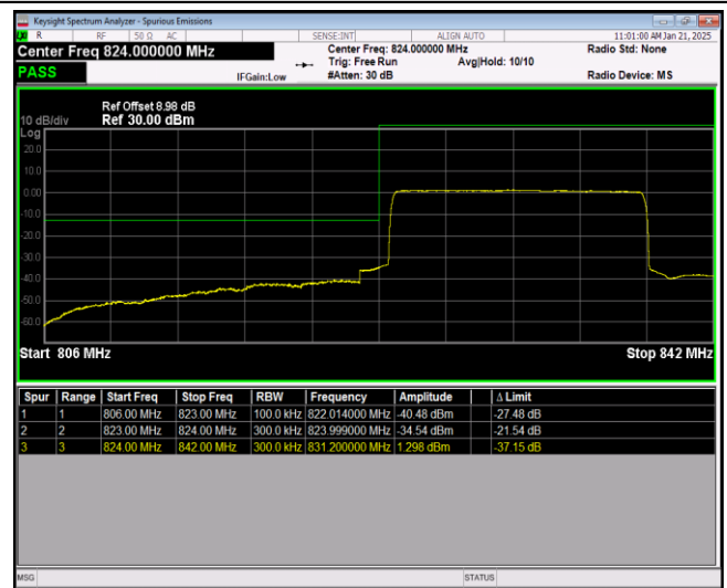
Band26-15MHz-64QAM-26965-1RB#74
