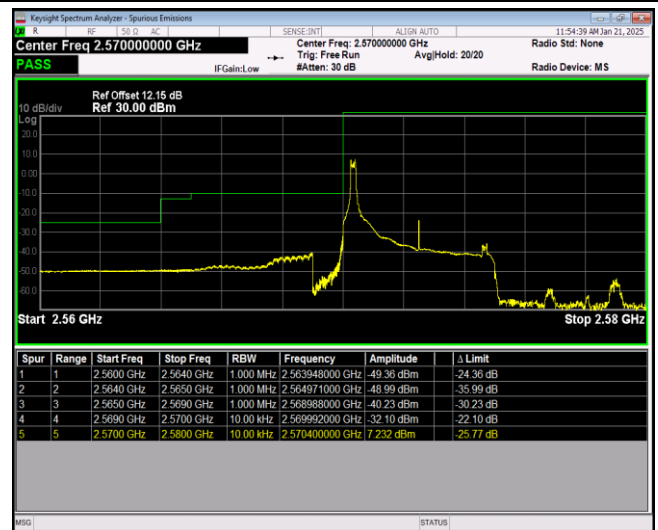
Band38-5MHz-16QAM-37775-25RB#0
