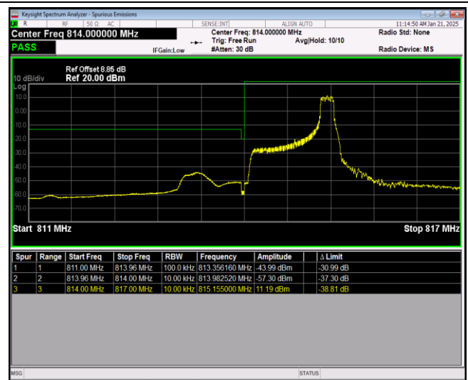
Band26-1.4MHz-16QAM-26783-1RB#0
