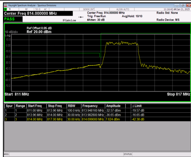
Band26-1.4MHz-64QAM-26783-1RB#5
