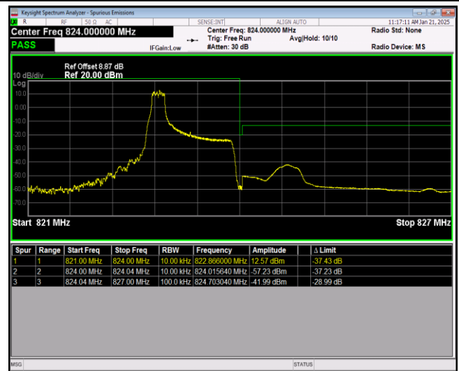
Band26-1.4MHz-QPSK-26783-6RB#0
