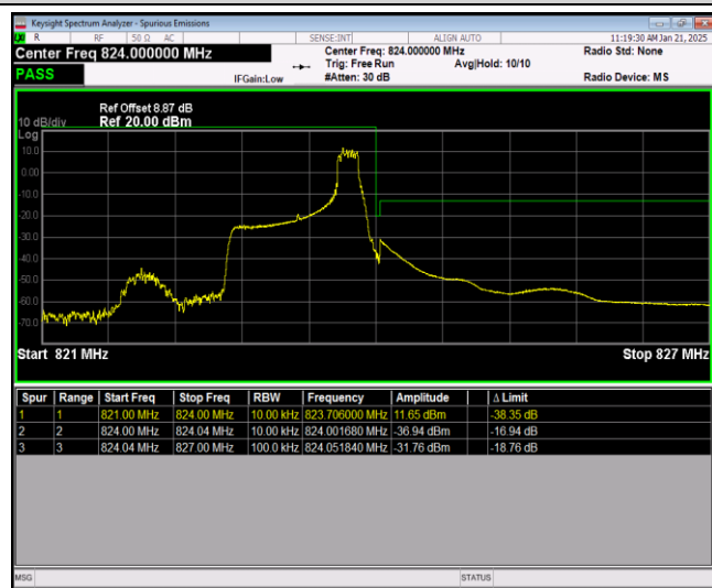
Band26-1.4MHz-64QAM-26797-1RB#0
