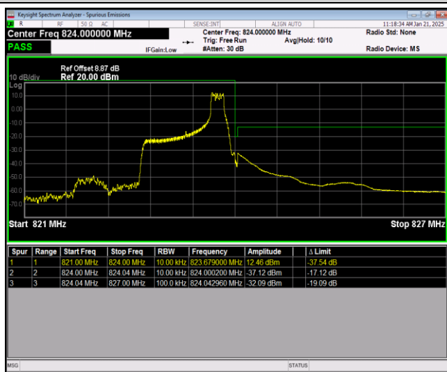
Band26-1.4MHz-QPSK-26797-1RB#0
