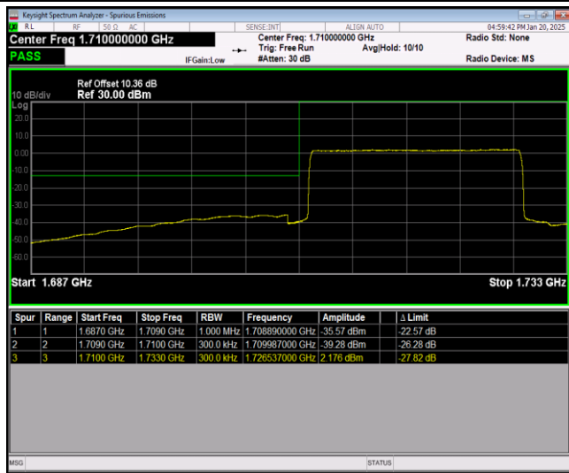
Band4-20MHz-16QAM-20300-1RB#99
