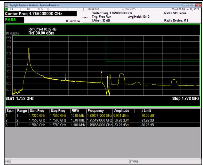
Band4-20MHz-16QAM-20300-100RB#0
