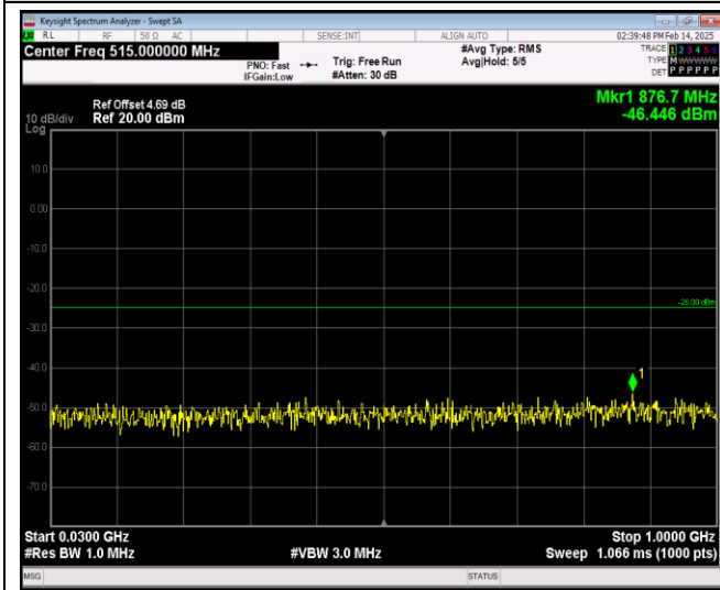
Band38-20MHz-64QAM-38000-1RB#0-Range1:30~1000MHz
