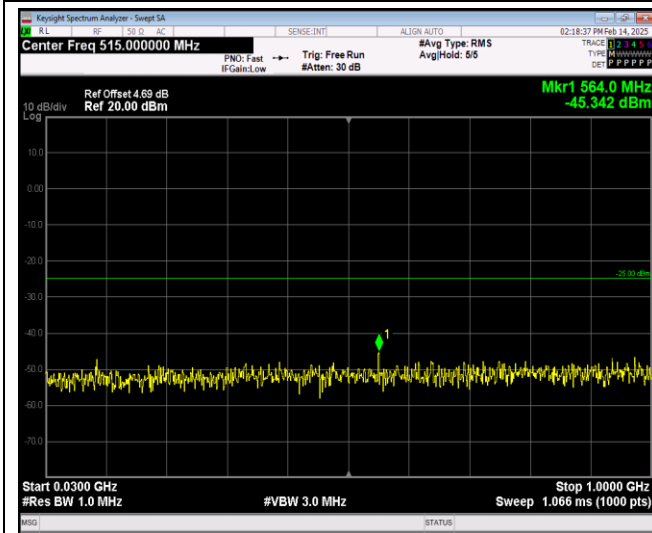
Band38-5MHz-QPSK-38000-1RB#0-Range1:30~100 OMHz
