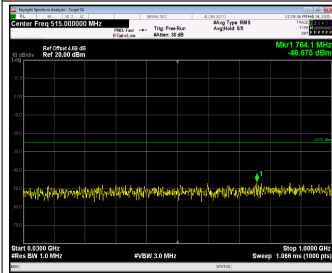
Band38-5MHz-QPSK-38000-1RB#0-Range1:30~100 OMHz
