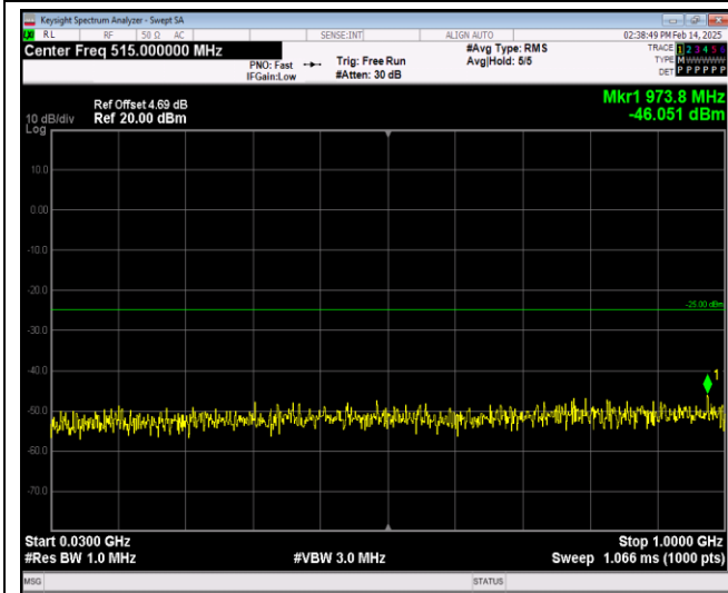
Band38-20MHz-64QAM-38000-1RB#0-Range1:30~1000MHz
