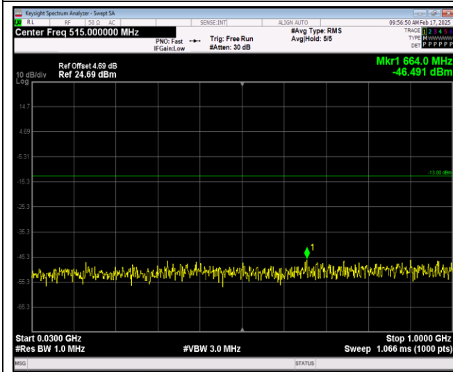
Band66-1.4MHz-16QAM-132665-1RB#0-Range1:30~1000MHz
