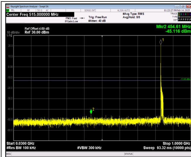
Band38-5MHz-QPSK-37775-1RB#0-Range1:30~100 OMHz
