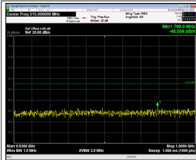
Band38-20MHz-64QAM-37850-1RB#0-Range1:30~1000MHz
