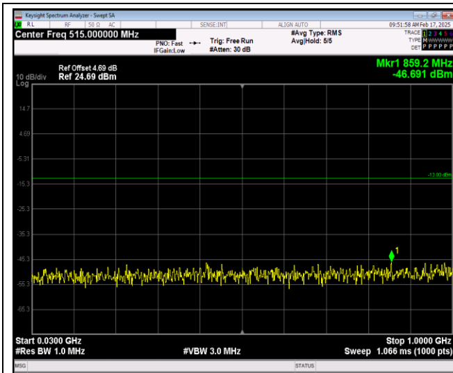
Band66-1.4MHz-16QAM-132322-1RB#0-Range1:30~1000MHz
