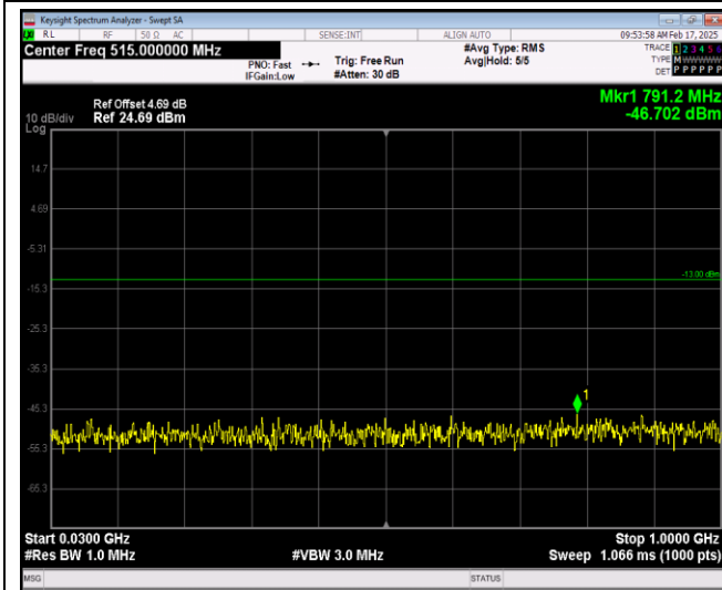
Band66-1.4MHz-16QAM-132665-1RB#0-Range1:30~1000MHz
