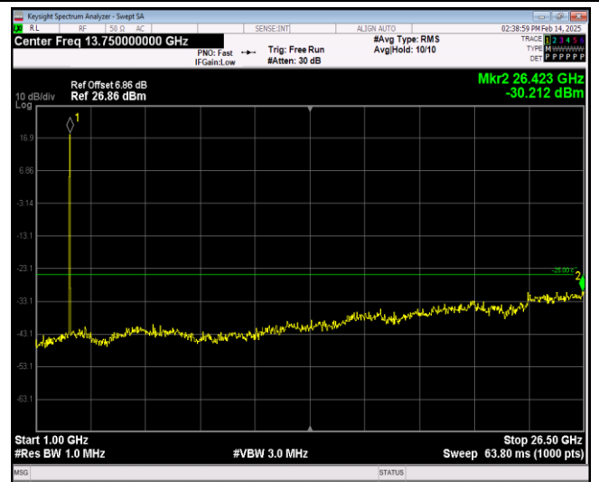
Band38-20MHz-64QAM-38000-1RB#0-Range2:1000~26500MHz
