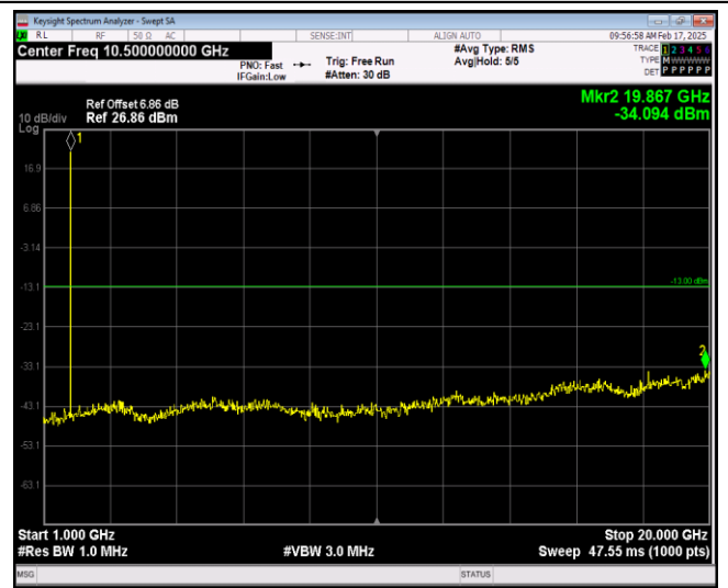
Band66-1.4MHz-16QAM-132665-1RB#0-Range2:1000~20000MHz
