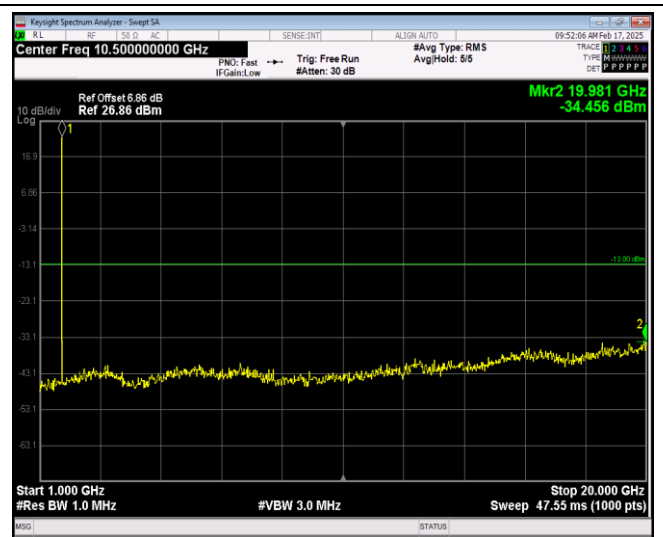
Band66-1.4MHz-16QAM-132322-1RB#0-Range2:1000~20000MHz
