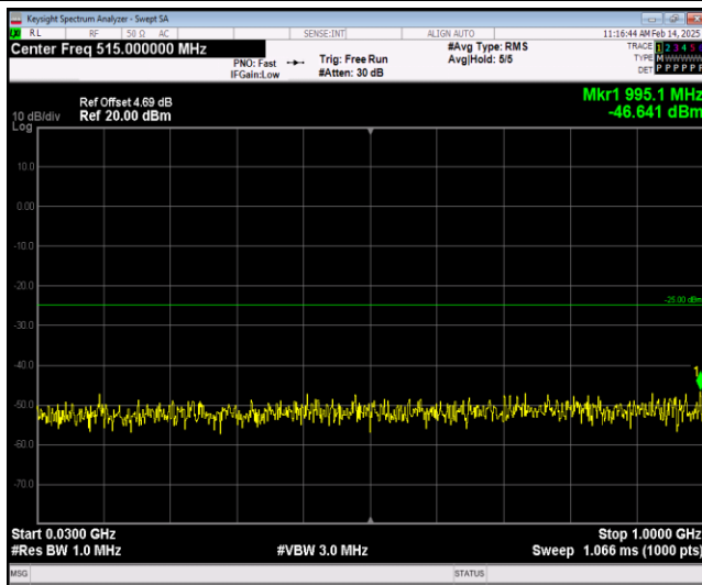
Band7-20MHz-64QAM-21350-1RB#0-Range1:30~1000MHz
