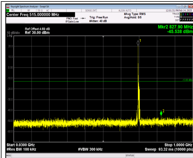
Band12-10MHz-QPSK-23130-1RB#0-Range1:30~1000MHz
