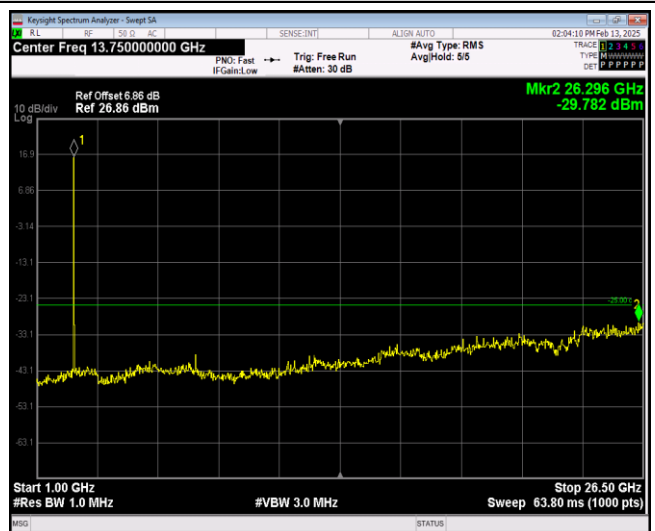
Band7-5MHz-16QAM-20775-1RB#0-Range2:1000~2 6500MHz
