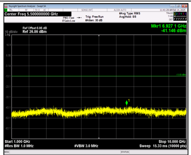
Band12-1.4MHz-64QAM-23095-1RB#0-Range2:1000~10000MHz
