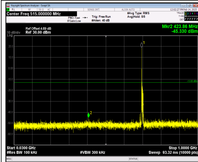
Band12-10MHz-64QAM-23130-1RB#0-Range1:30~-1000MHz
