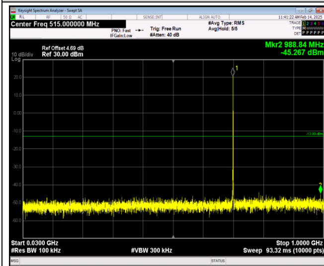
Band12-1.4MHz-64QAM-23095-1RB#0-Range1:30~1000MHz
