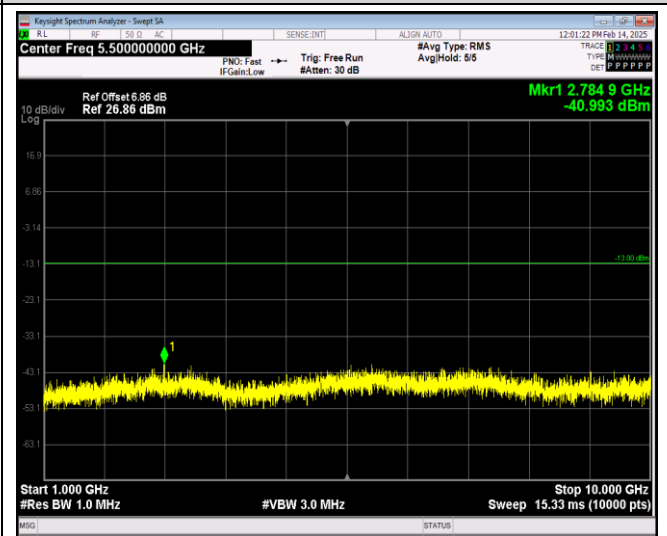
Band12-10MHz-16QAM-23060-1RB#0-Range2:1000~10000MHz
