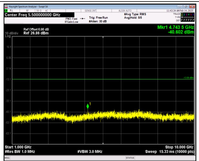
Band12-1.4MHz-64QAM-23017-1RB#0-Range2:1000~10000MHz
