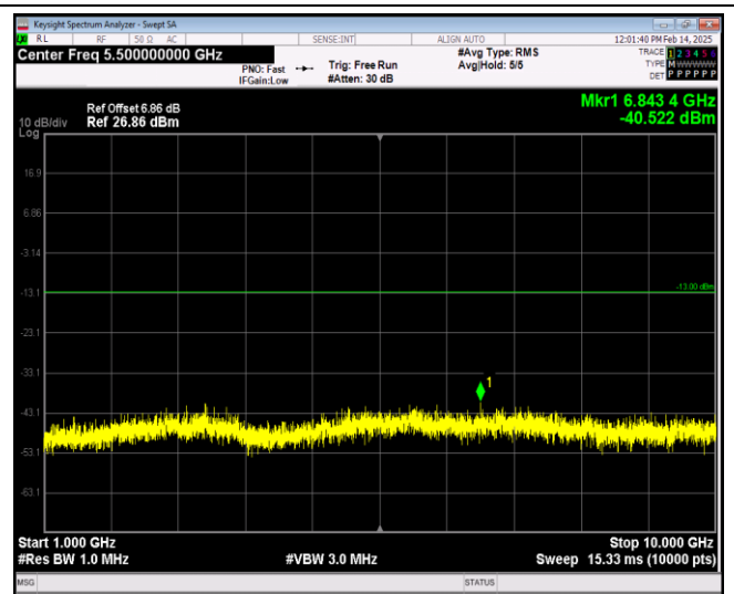
Band12-10MHz-64QAM-23095-1RB#0-Range2:1000~10000MHz
