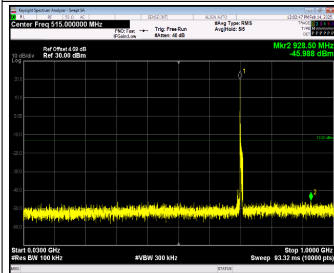
Band12-10MHz-16QAM-23060-1RB#0-Range1:30~1000MHz
