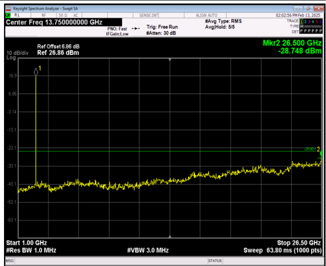
Band7-5MHz-64QAM-21100-1RB#0-Range2:1000~2 6500MHz
