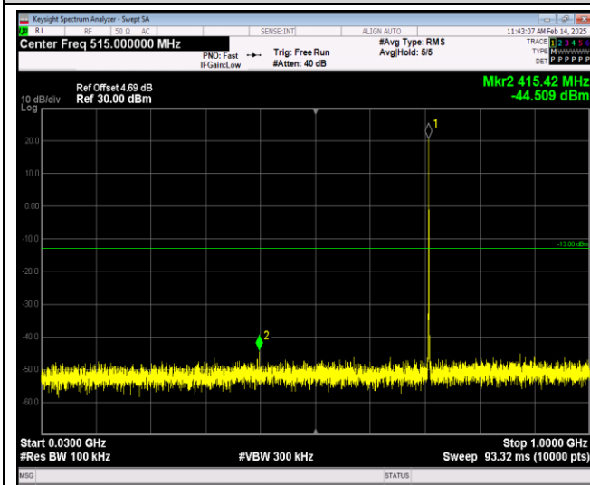
Band12-1.4MHz-QPSK-23173-1RB#0-Range1:30~1000MHz
