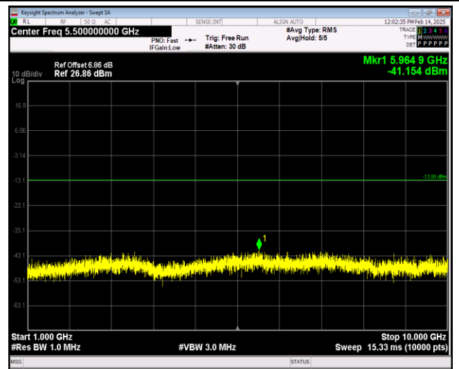
Band12-10MHz-64QAM-23130-1RB#0-Range2:1000~10000MHz
