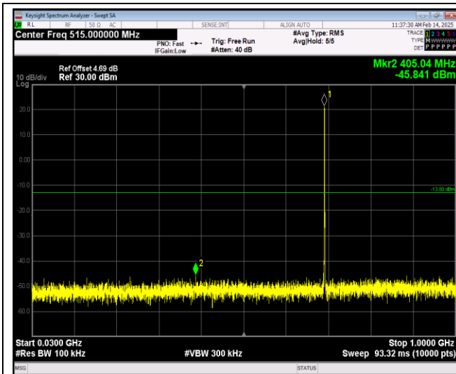
Band12-1.4MHz-QPSK-23095-1RB#0-Range1:30~1000MHz
