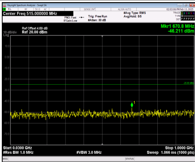
Band7-5MHz-QPSK-21425-1RB#0-Range1:30~1000 MHz
