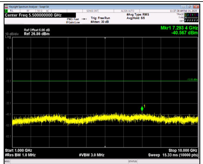
Band12-1.4MHz-QPSK-23095-1RB#0-Range2:1000~10000MHz
