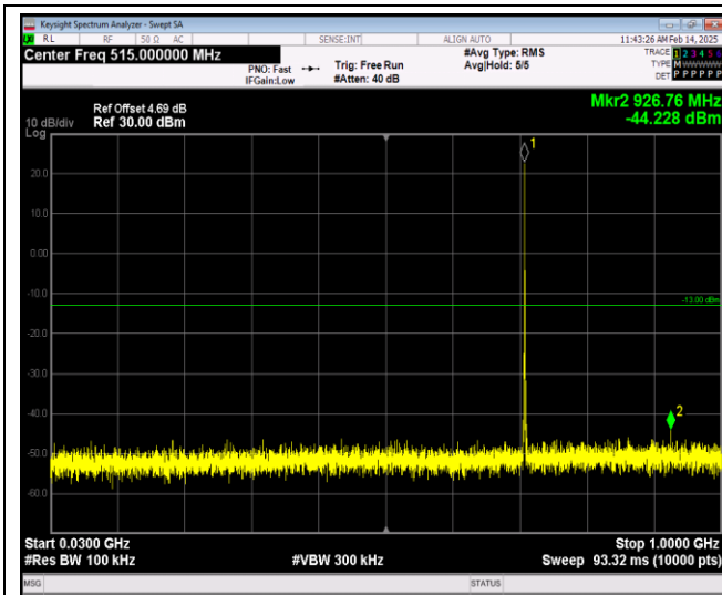
Band12-1.4MHz-64QAM-23017-1RB#0-Range1:30~1000MHz
