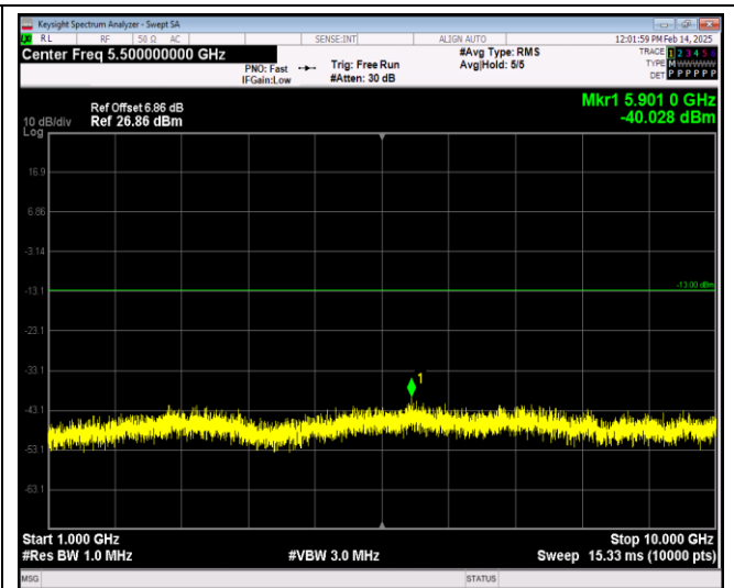
Band12-10MHz-QPSK-23130-1RB#0-Range2:1000~10000MHz
