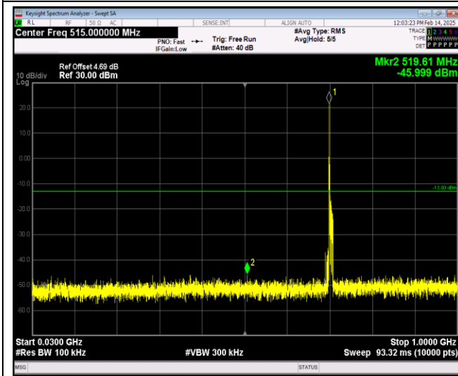
Band12-10MHz-64QAM-23130-1RB#0-Range1:30~-1000MHz
