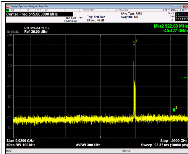
Band12-10MHz-64QAM-23095-1RB#0-Range1:30~-1000MHz
