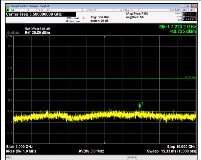
Band12-10MHz-16QAM-23060-1RB#0-Range2:1000~10000MHz
