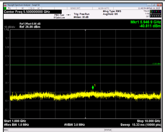
Band12-1.4MHz-QPSK-23173-1RB#0-Range2:1000~10000MHz
