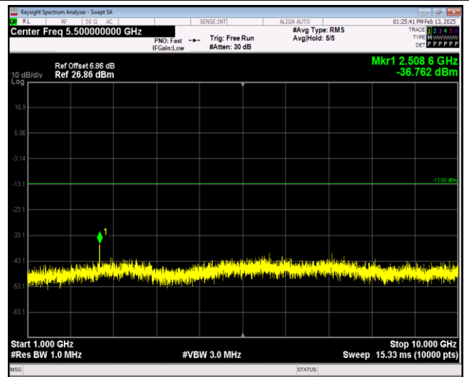
Band5-1.4MHz-16QAM-20643-1RB#0-Range2:1000~10000MHz
