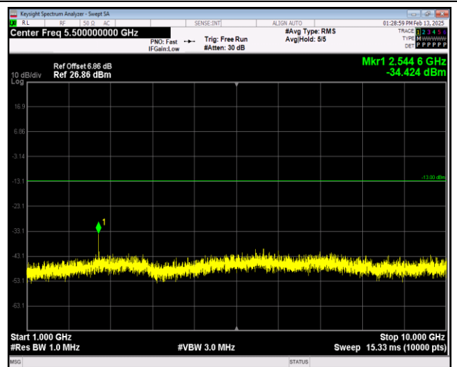
Band5-1.4MHz-64QAM-20407-1RB#0-Range2:1000~10000MHz
