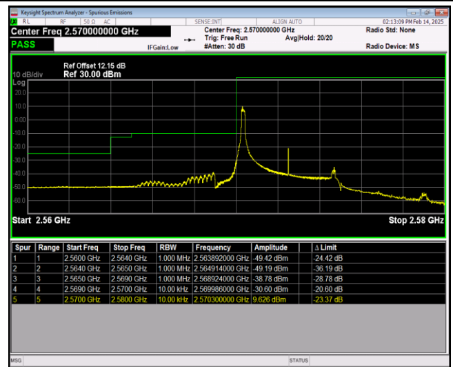
Band38-5MHz-16QAM-37775-25RB#0
