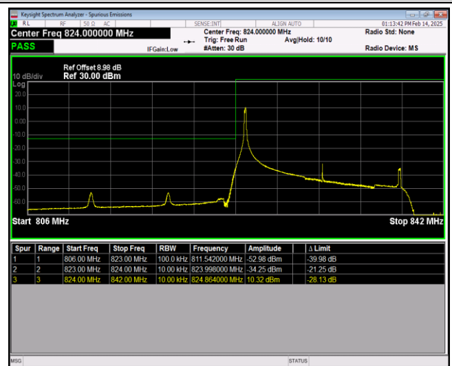
Band26-15MHz-16QAM-26865-75RB#0
