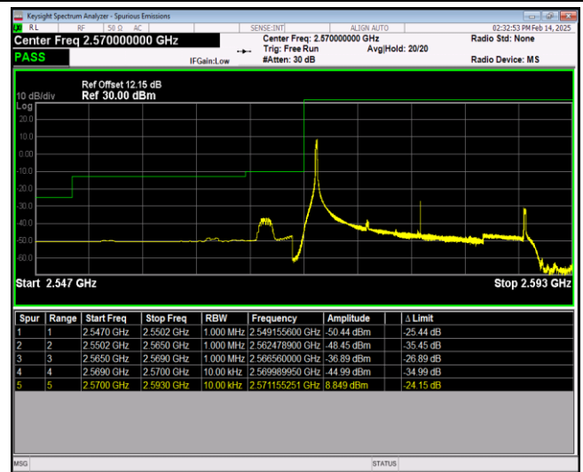
Band38-20MHz-64QAM-37850-100RB#0
