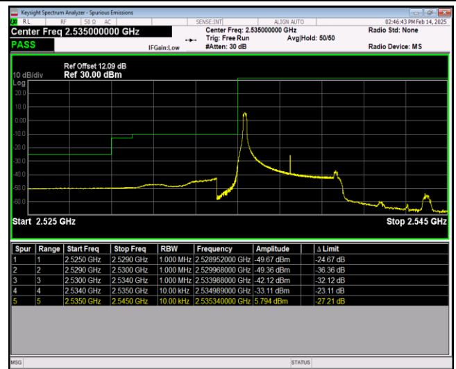
Band41-5MHz-16QAM-40065-25RB#0
