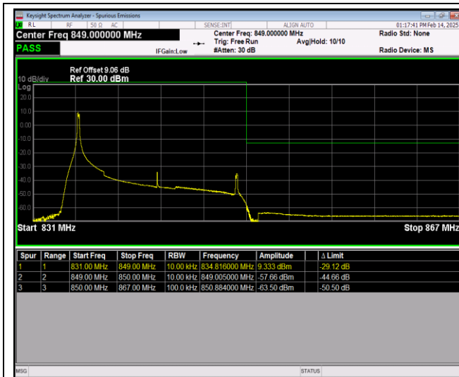
Band26-15MHz-64QAM-26965-75RB#0
