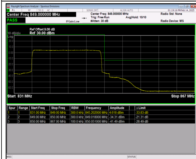
Band26-15MHz-16QAM-26865-1RB#74
