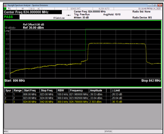
Band26-15MHz-64QAM-26965-1RB#74
