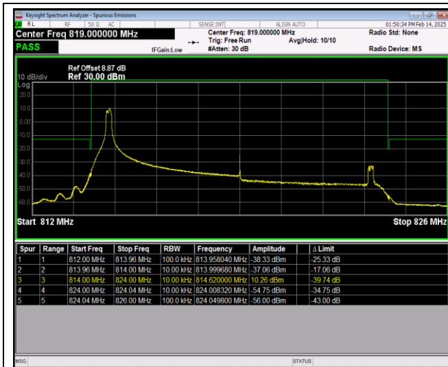
Band26-10MHz-64QAM-26740-50RB#0
