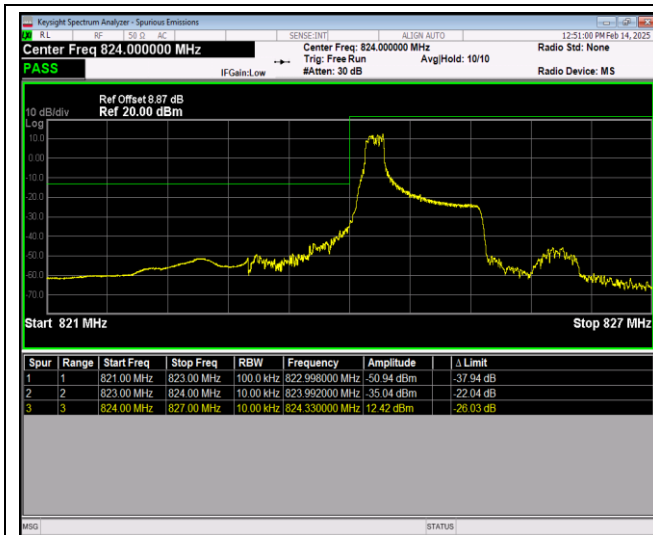
Band26-1.4MHz-64QAM-26797-6RB#0
