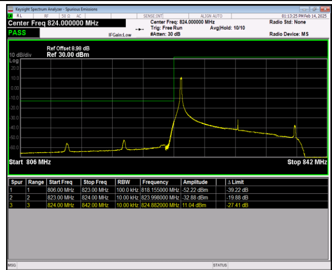
Band26-15MHz-QPSK-26865-75RB#0
