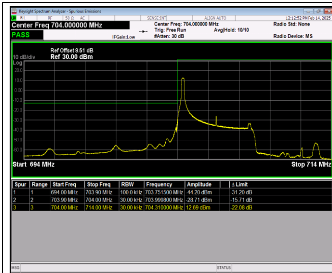
Band17-5MHz-16QAM-23755-25RB#0
