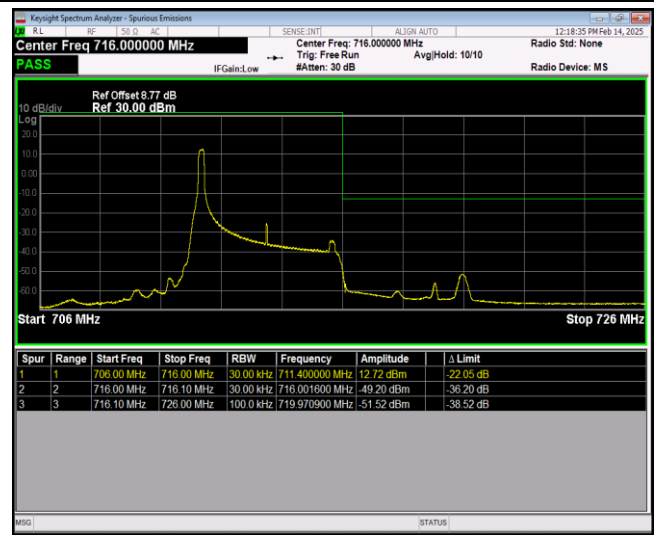
Band17-5MHz-16QAM-23825-25RB#0
