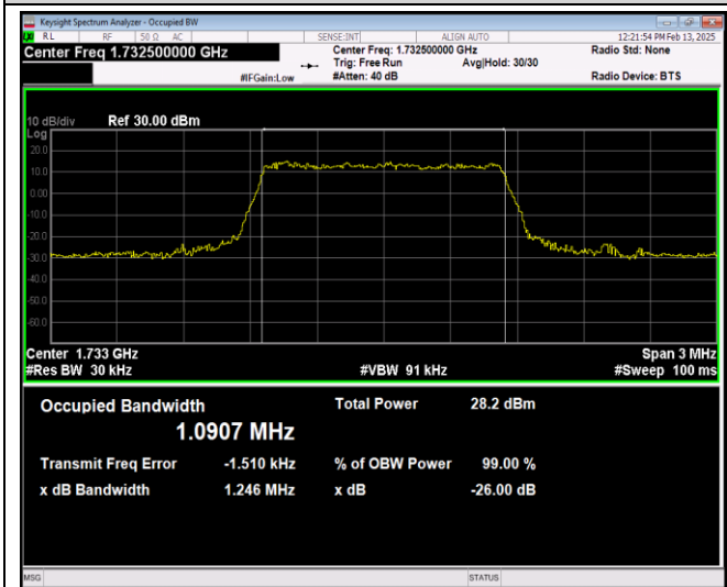
Band4-1.4MHz-64QAM-19957-6RB#0
