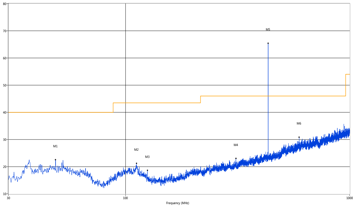
30 MHz to 1 GHz, Low Channel, ANT V
