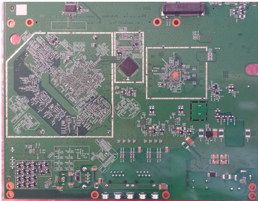
Picture 2: Main Board - Back View
