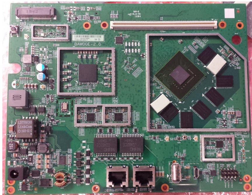
Picture 1: Main Board - Top View (Shields removed)
