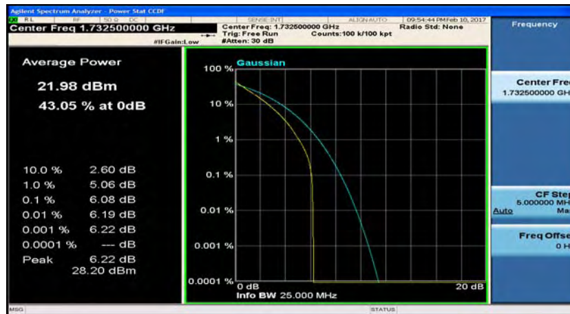
(LTE band 4_Channel Bandwidth:20 MHz)_MCH_QPSK_50RB#25
