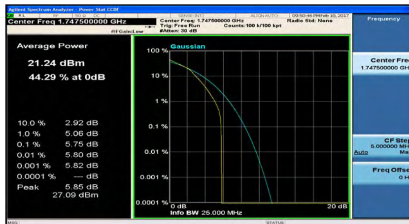
(LTE band 4_Channel Bandwidth:15 MHz)_HCH_16QAM_37RB#38
