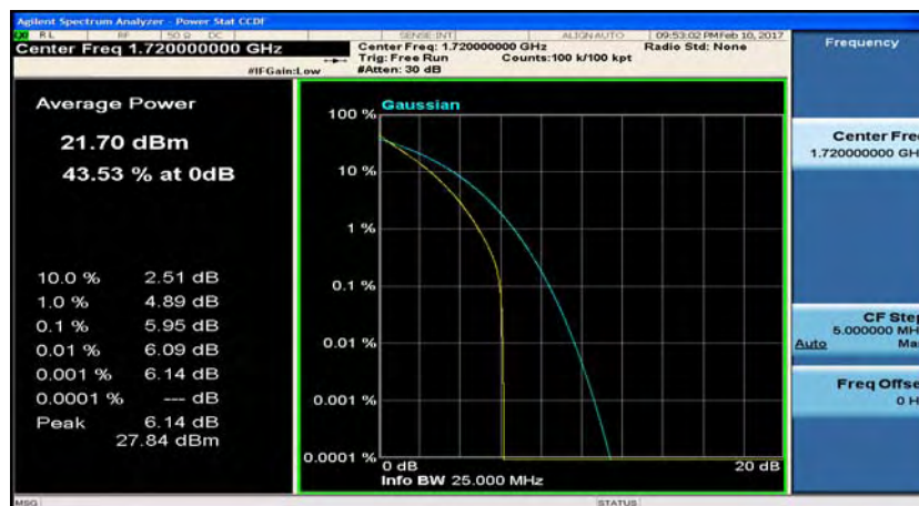
(LTE band 4_Channel Bandwidth:20 MHz)_LCH_QPSK_50RB#50
