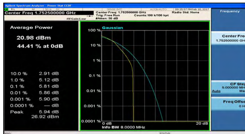
(LTE band 4_Channel Bandwidth: 5 MHz)_HCH_16QAM_12RB#6
