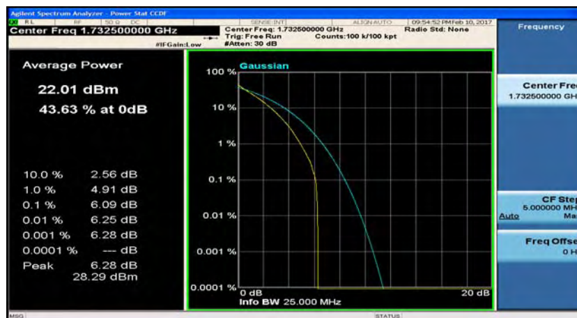
(LTE band 4_Channel Bandwidth:20 MHz)_MCH_QPSK_50RB#50
