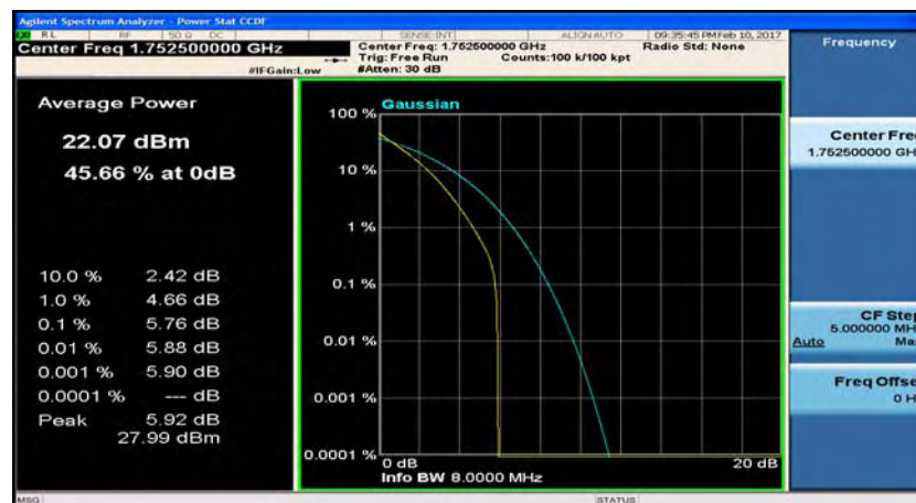
(LTE band 4_Channel Bandwidth: 5 MHz)_HCH_QPSK_12RB#13
