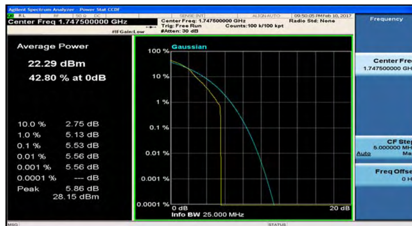
(LTE band 4_Channel Bandwidth:15 MHz)_HCH_16QAM_1RB#74
