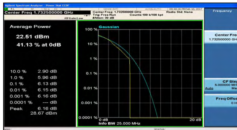
(LTE band 4_Channel Bandwidth:15 MHz)_MCH_16QAM_1RB#74
