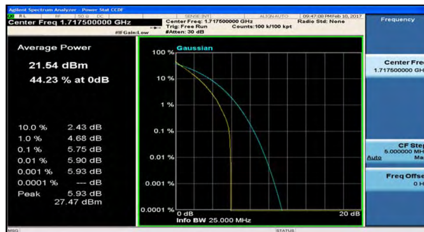
(LTE band 4_Channel Bandwidth:15 MHz)_LCH_QPSK_37RB#38
