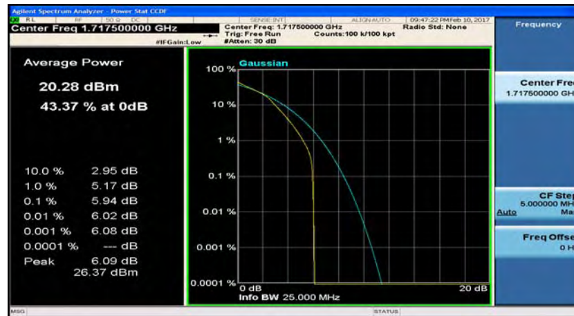
(LTE band 4_Channel Bandwidth:15 MHz)_LCH_16QAM_37RB#18
