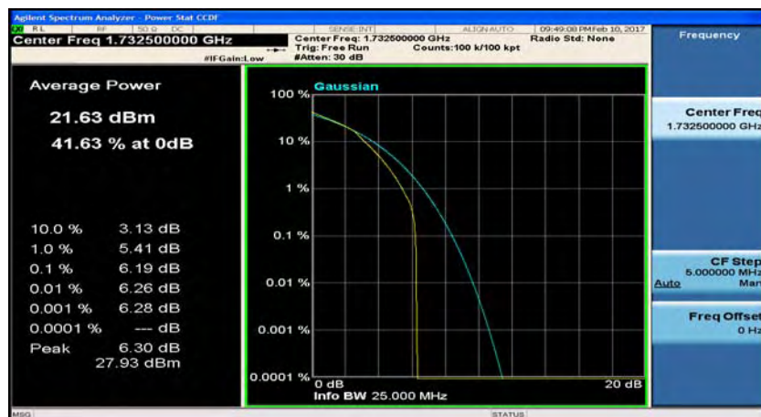
(LTE band 4_Channel Bandwidth:15 MHz)_MCH_16QAM_37RB#38
