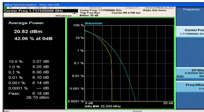
(LTE band 4_Channel Bandwidth:15 MHz)_LCH_16QAM_37RB#38
