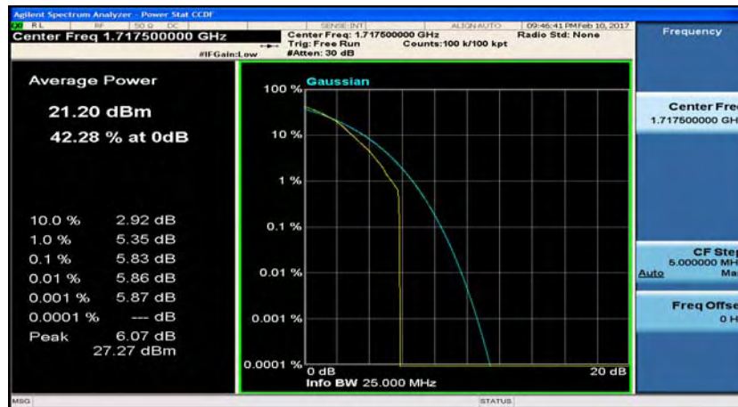
(LTE band 4_Channel Bandwidth:15 MHz)_LCH_16QAM_1RB#37
