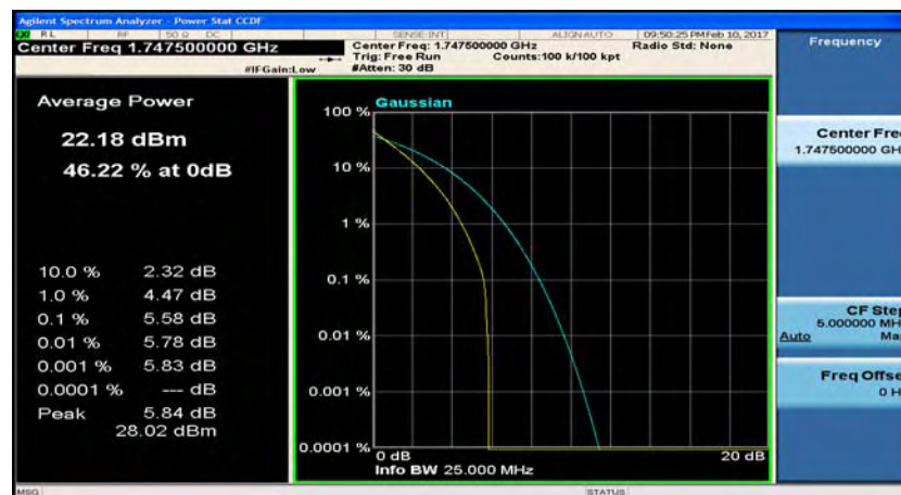
(LTE band 4_Channel Bandwidth:15 MHz)_HCH_QPSK_37RB#38
