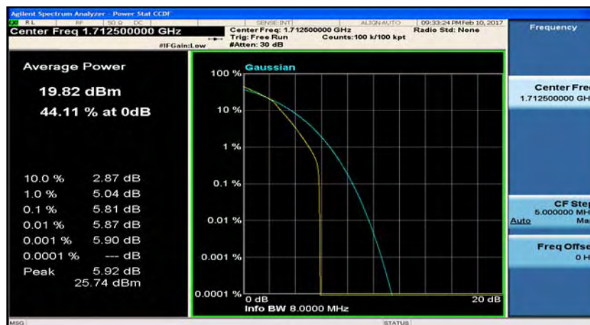
(LTE band 4_Channel Bandwidth: 5 MHz)_LCH_16QAM_12RB#13
