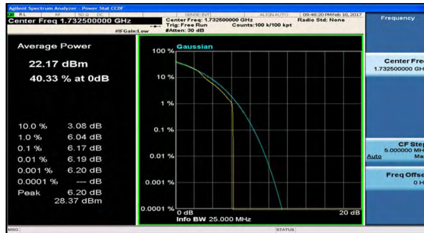
(LTE band 4_Channel Bandwidth:15 MHz)_MCH_16QAM_1RB#37
