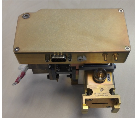
RF Detector
