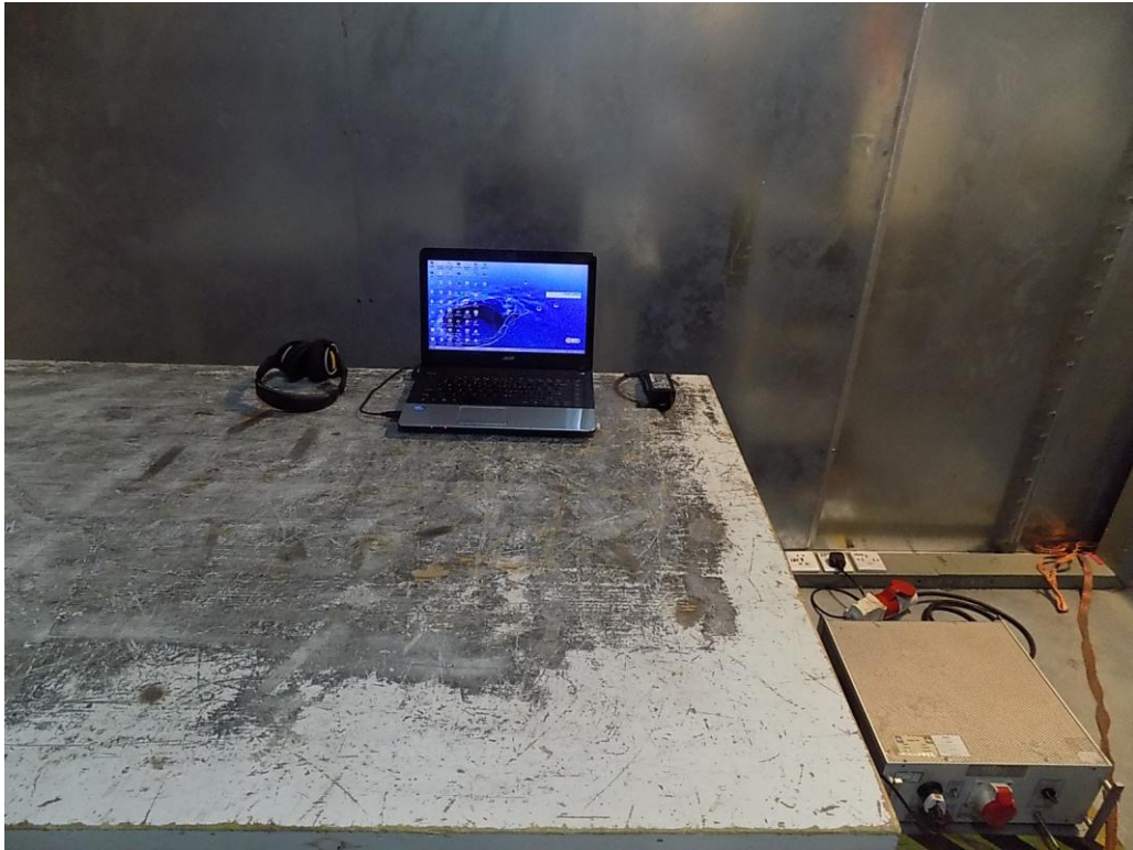
Photos of Power Line Conducted Emission
