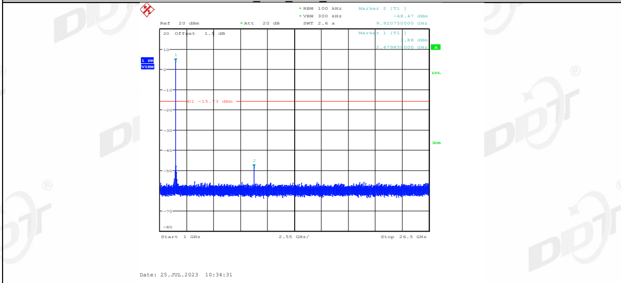
2DH5_Ant1_2402_0~Reference
