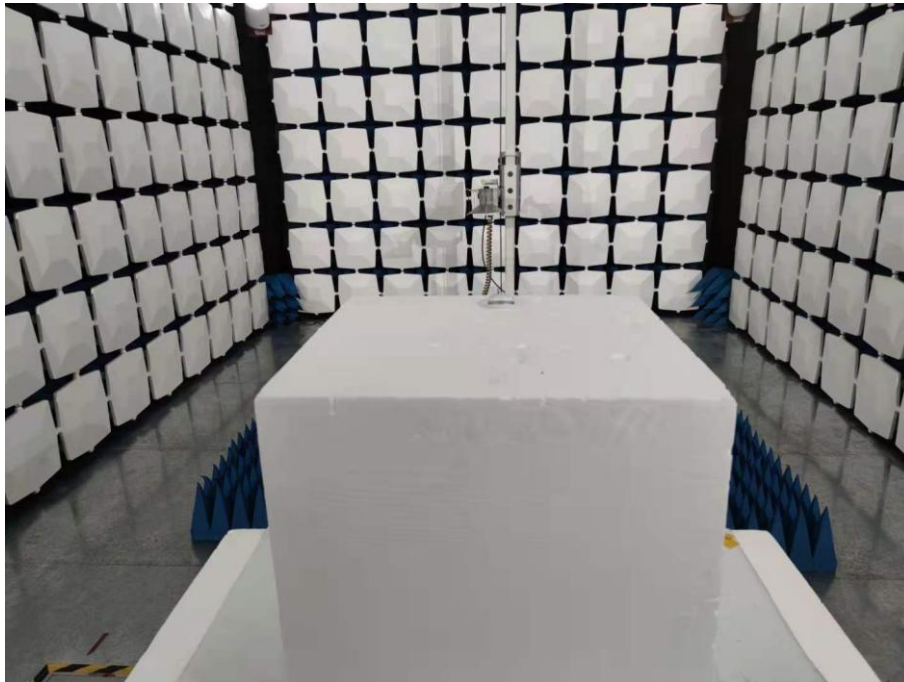
Model: MX107 Above 1GHz for radiated emission test setup
