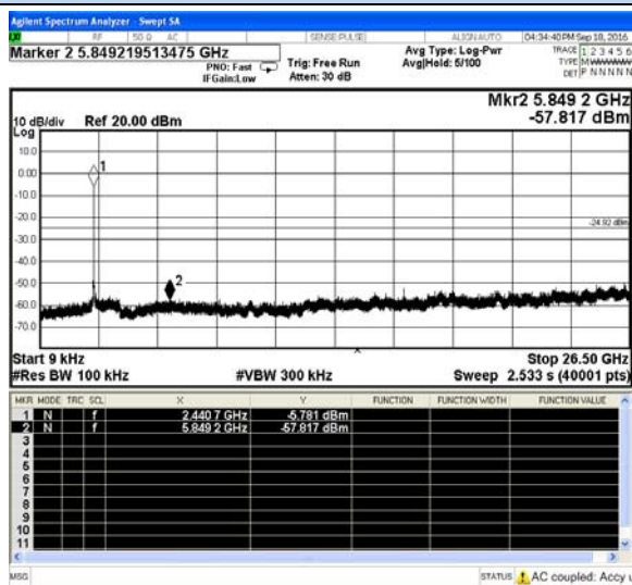
Middle channel
