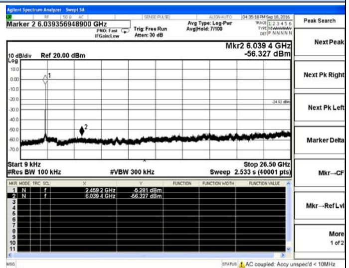
High channel
