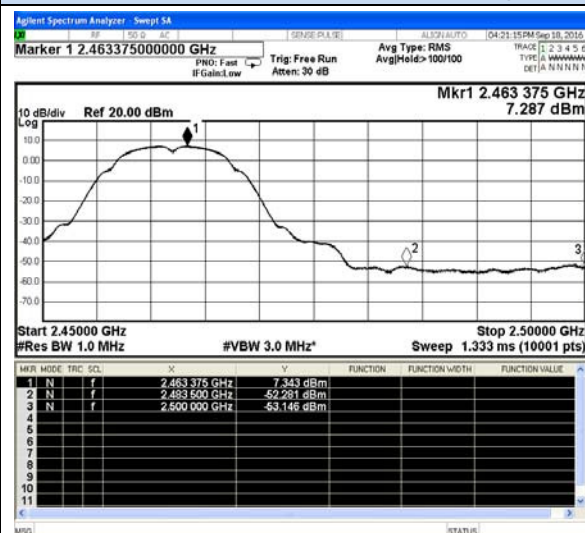
802.11b-High channel(Average)
