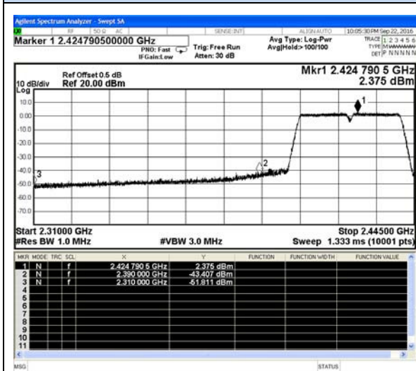
802.11n-HT40 Low channel(Peak)
