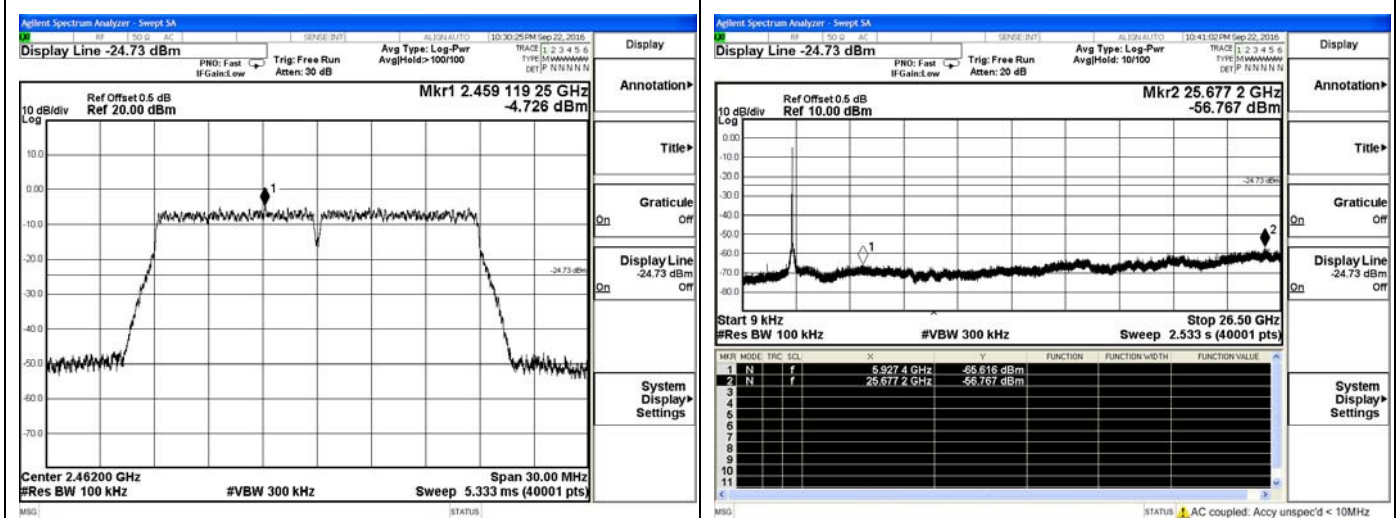
802.11n-HT20 High channel Reference
