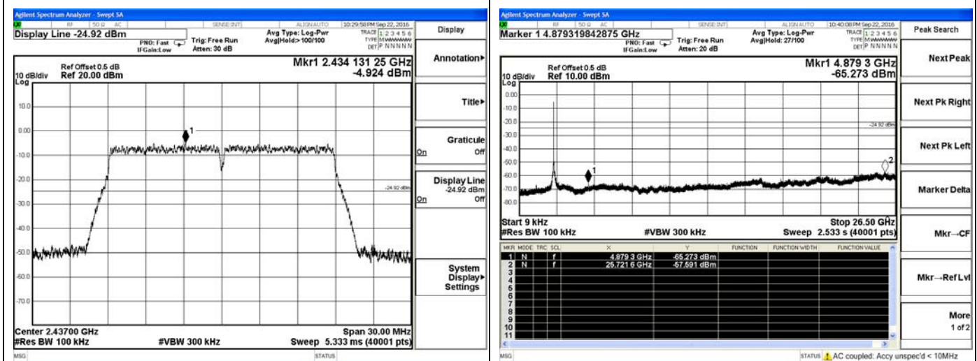
802.11n-HT20 Middle channel Reference
