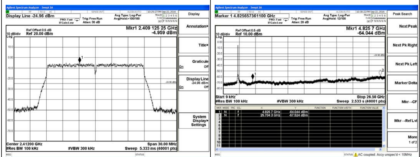
802.11n-HT20 Low channel Reference
