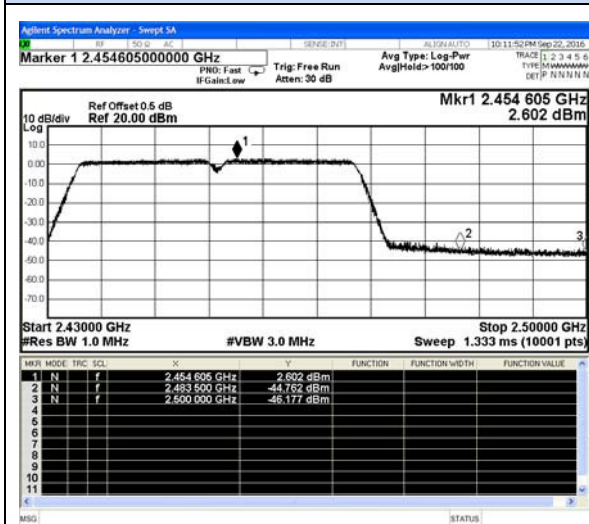
802.11n-HT40 High channel(Peak)
