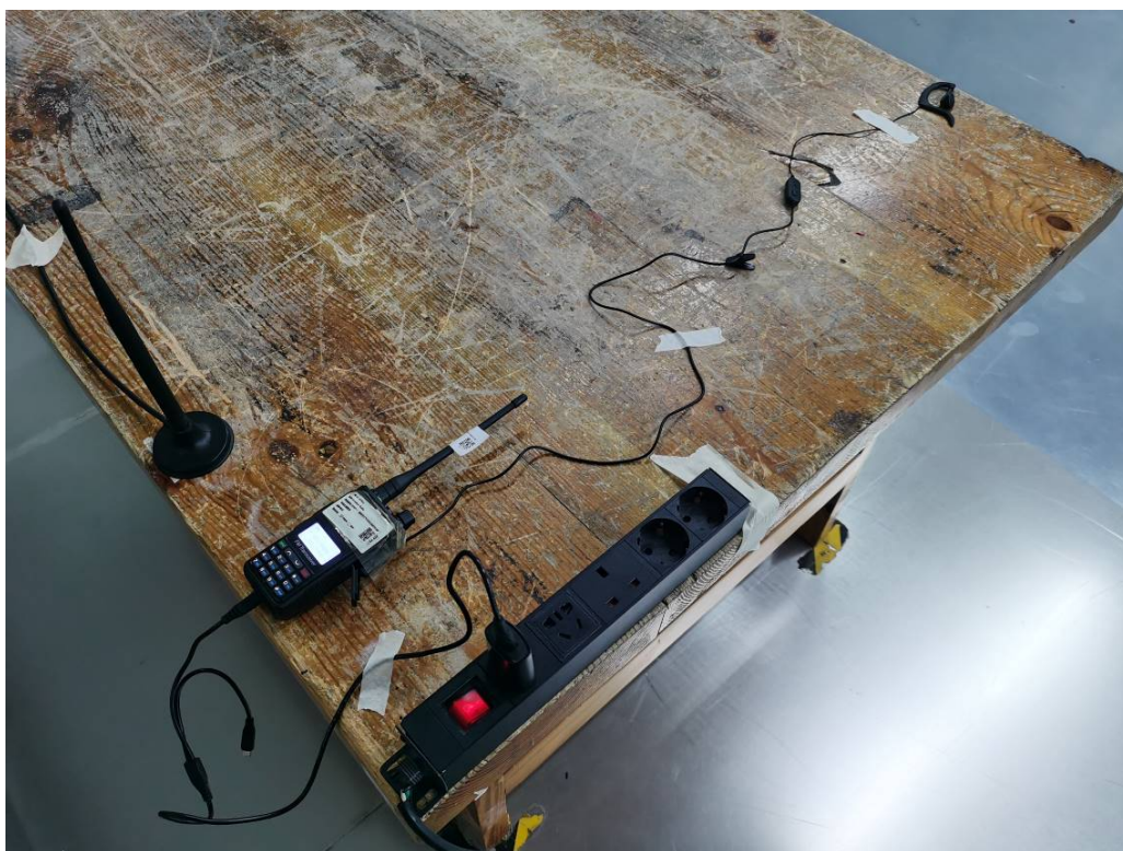
Conducted Emissions Side View M2,M3,M4
