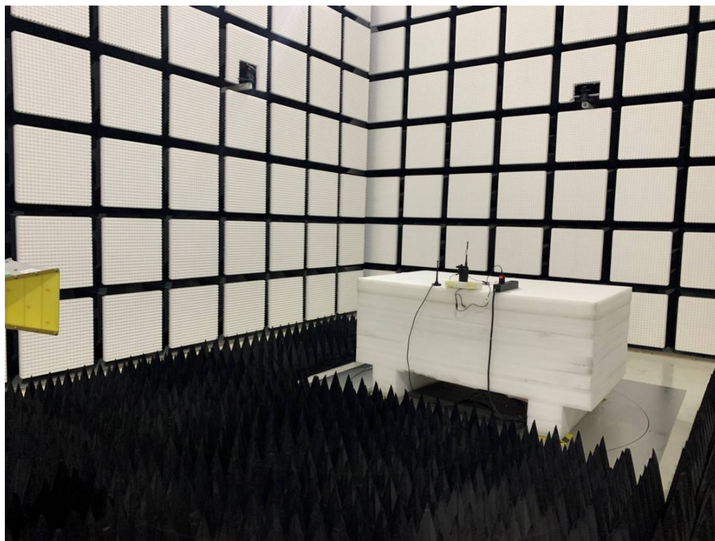
Radiated Emission Above 1GHz Rear View M2,M3,M4
