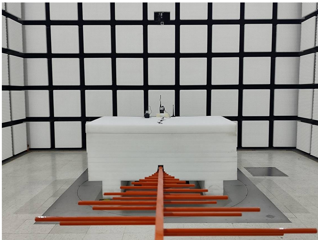
Radiated Emission Below 1GHz Rear View M2,M3,M4
