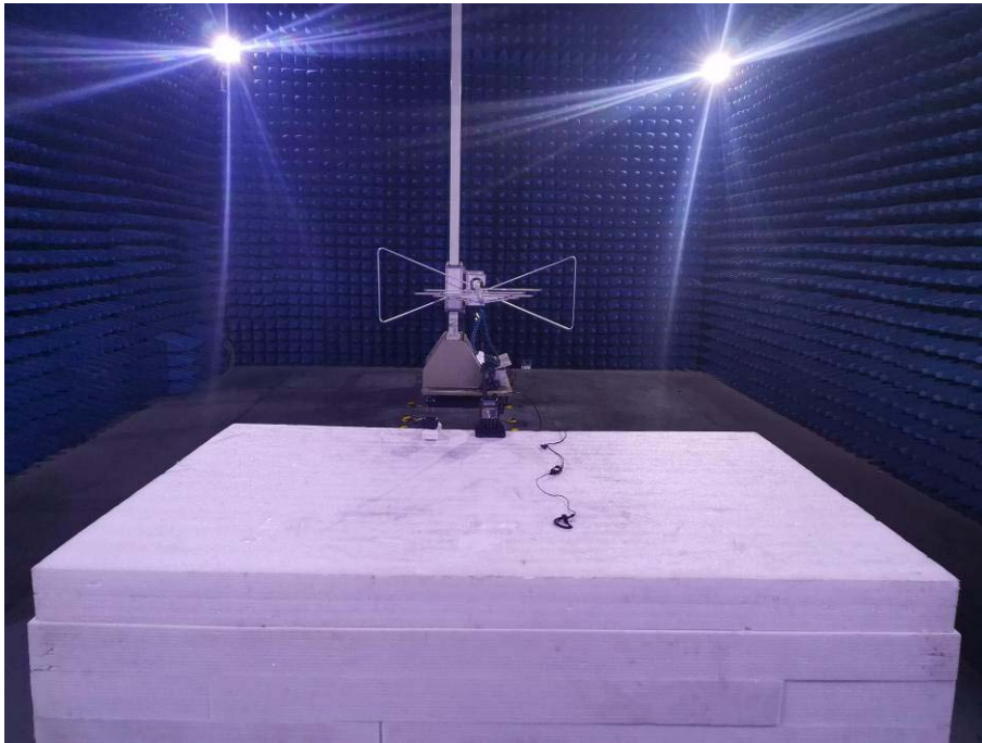
Photo of Radiated Emission Measurement (Below 1G) Test model
