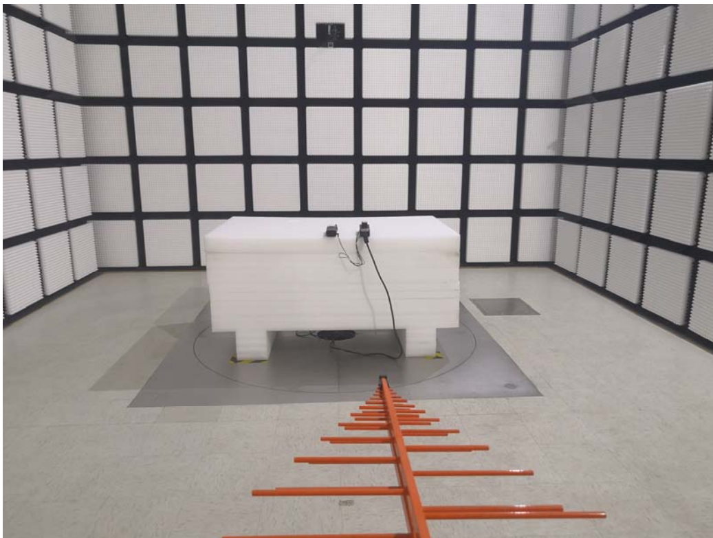
Radiated Emissions Below1G rear View-TM1
