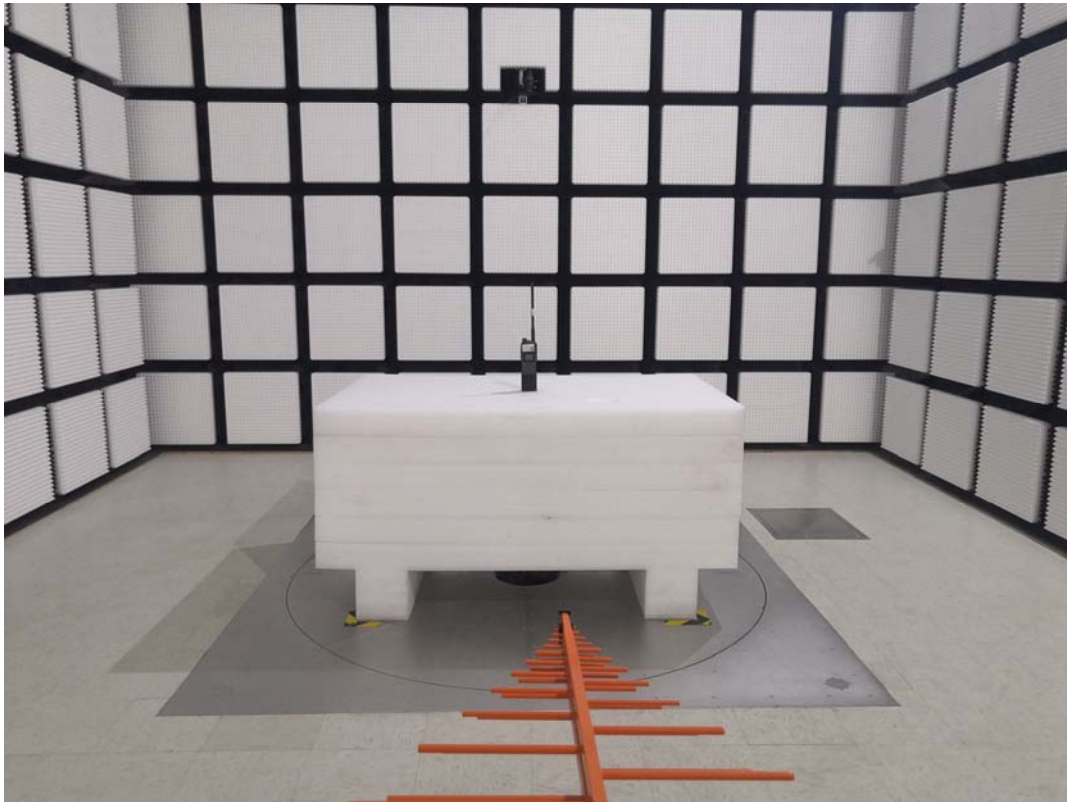
Radiated Emission Below 1G View-TM4
