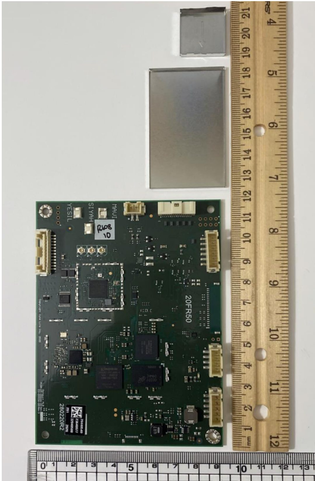
Figure 3: MLB with shield can removed
