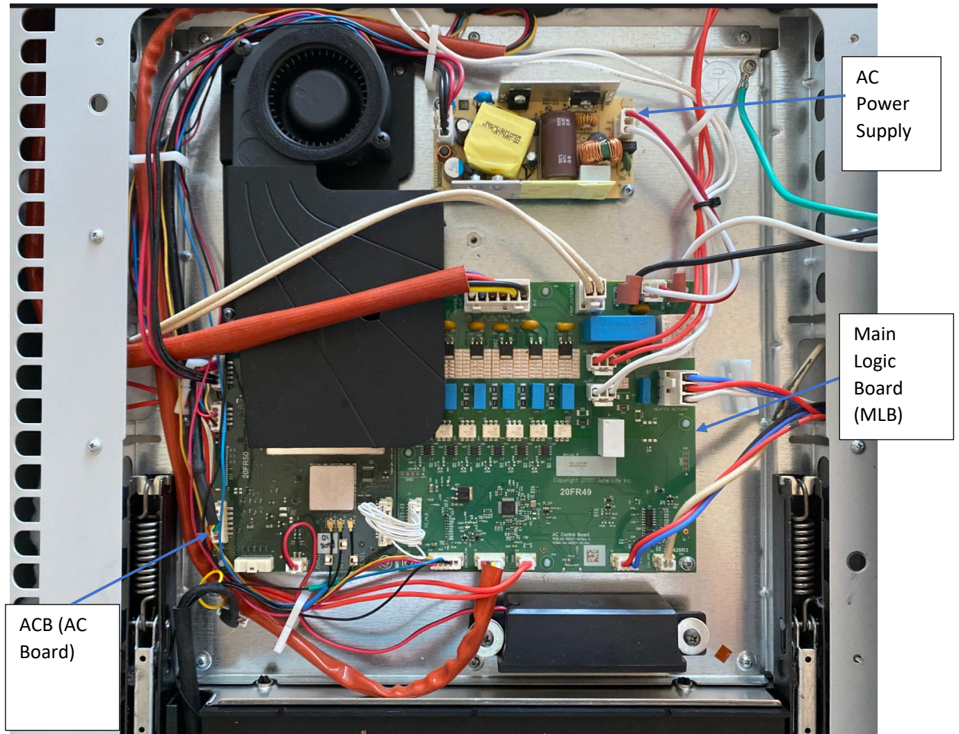
Figure 1: AC Power Supply, MLB (Main Logic Board), ACB (AC Control Board)
