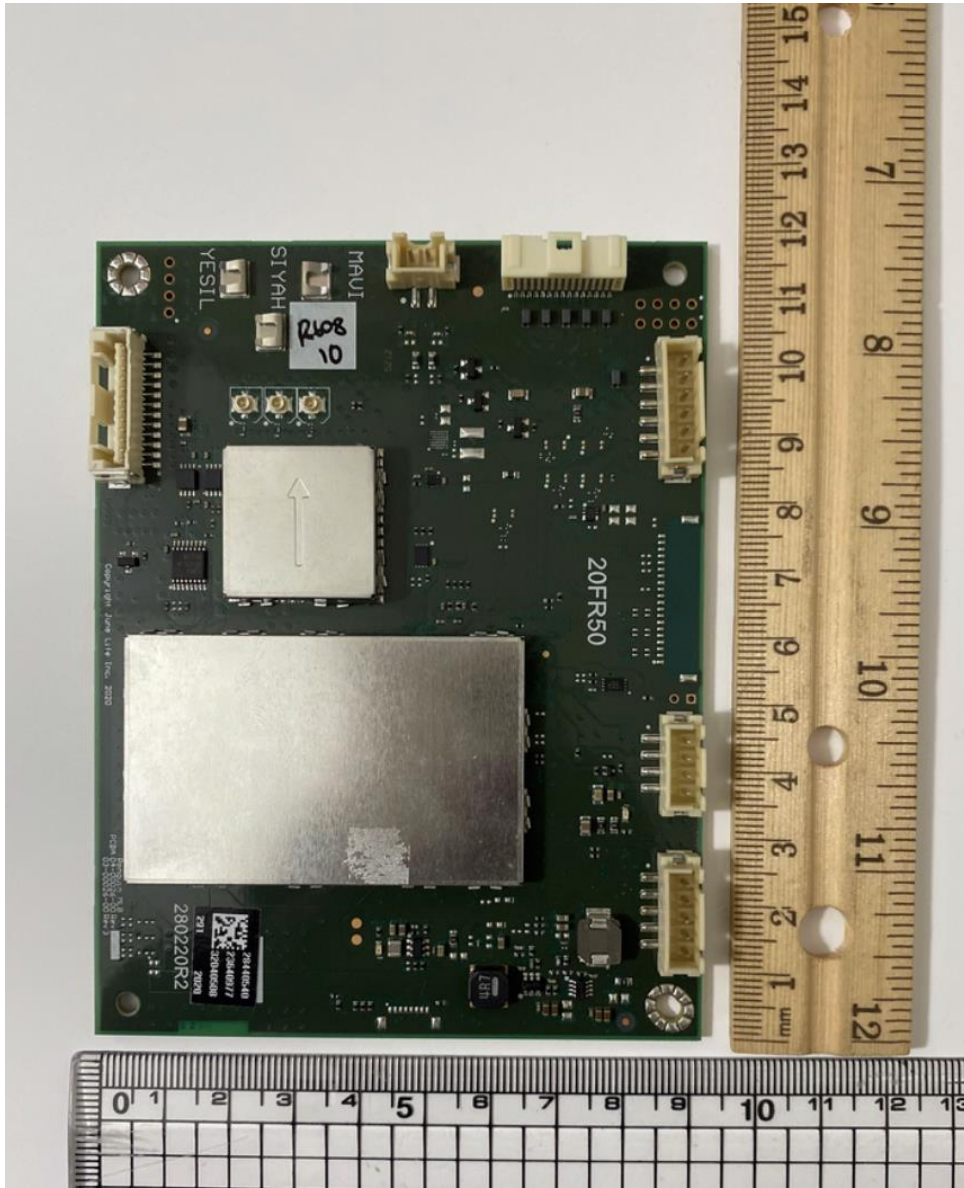
Figure 2: MLB With Shield Cans
