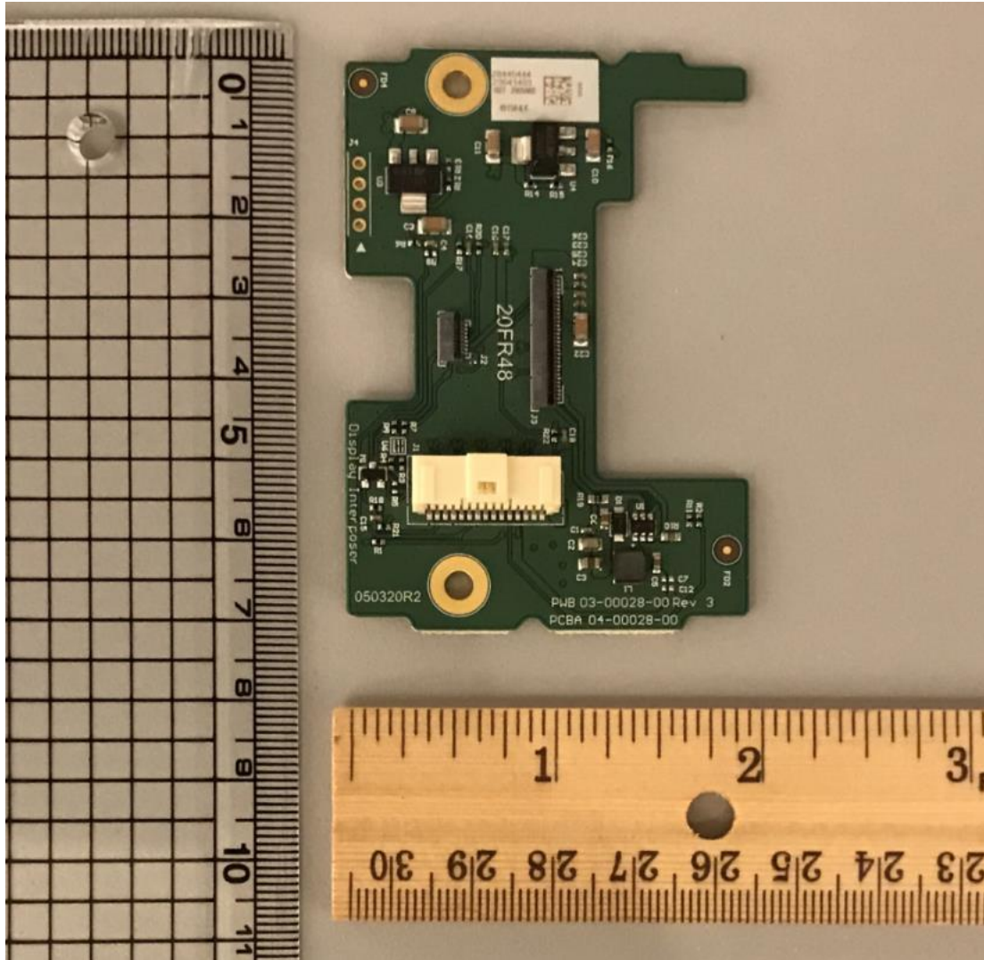
Figure 4: Display Interposer Board
