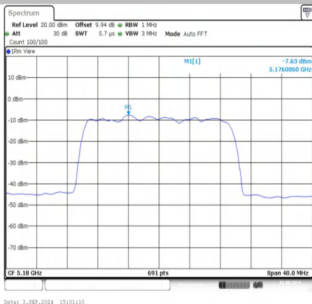
11AX20SISO-Ant1-5180-PASS
