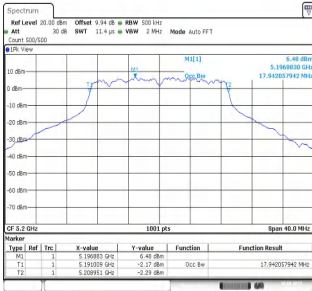
11N20SISO-Ant1-5200
