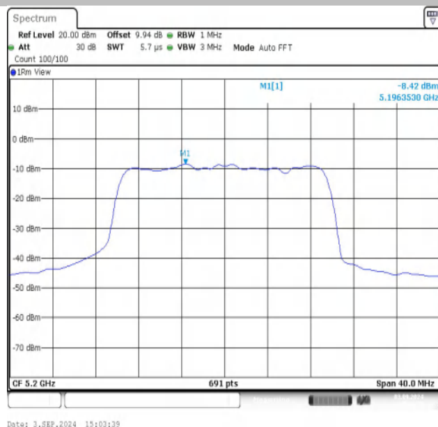
11AX20SISO-Ant1-5200-PASS
