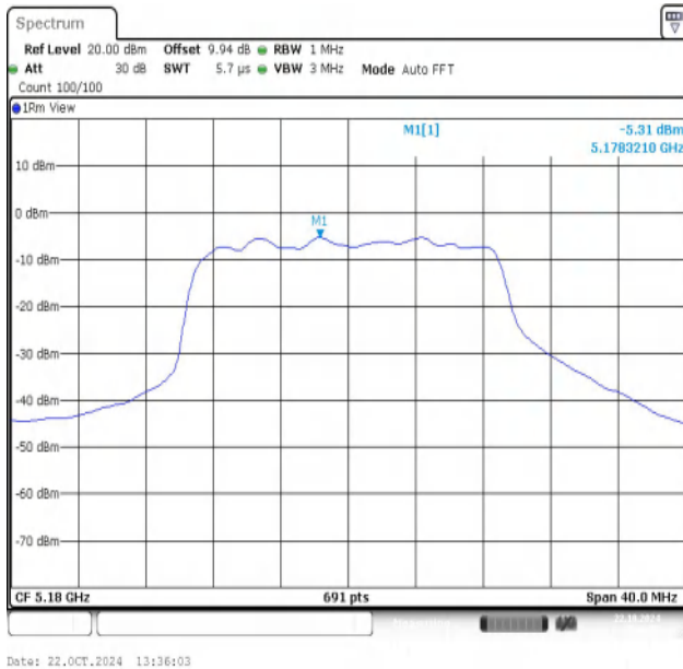
11AC20SISO-Ant1-5180-PASS
