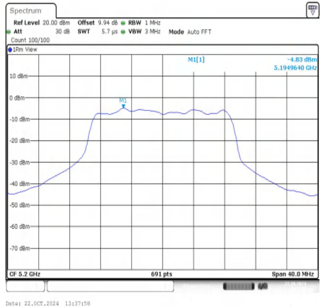
11AC20SISO-Ant1-5200-PASS
