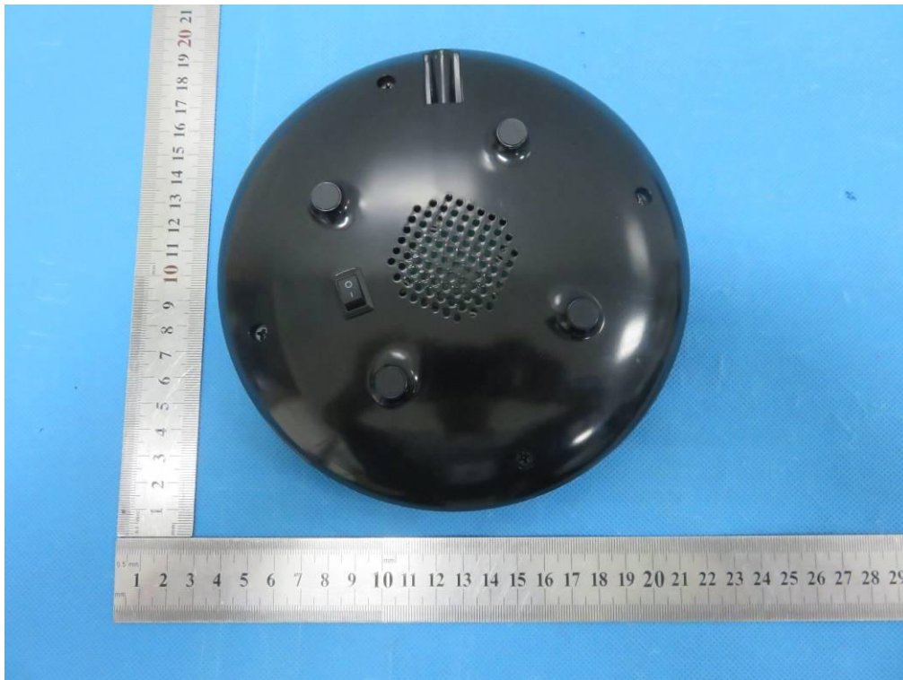
BOTTOM VIEW OF PEDESTAL-WB-46(3)
