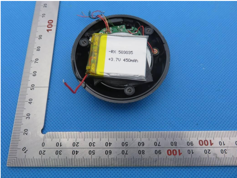
OPEN VIEW OF EUT-2 (WB-46)
