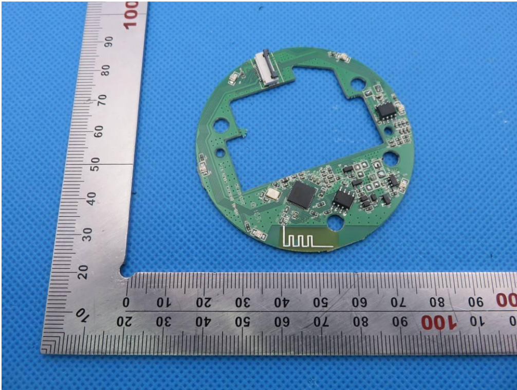
INTERNAL VIEW OF EUT-2 (WB-46)
