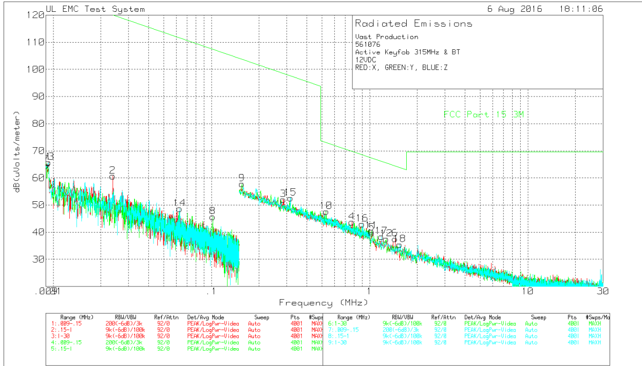
Figure 13 Radiated Emissions Graph (9kHz to 30MHz) Worst-Case – ASK Modulation
