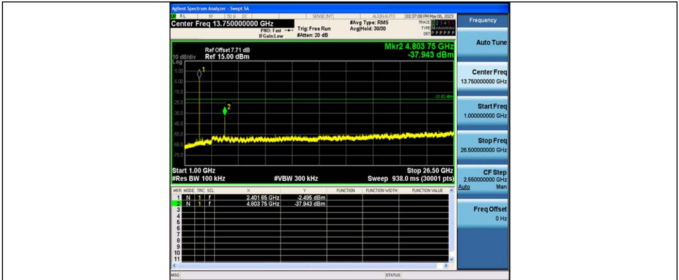
DH5_Ant1_2441_0~Reference
