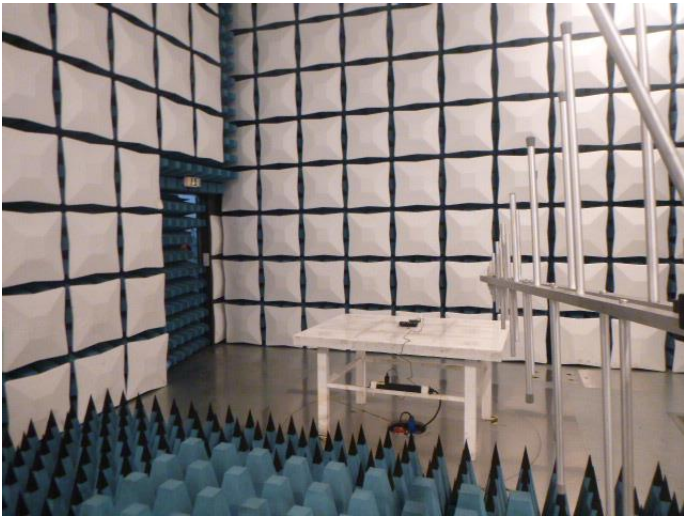
Carrier output power / transmit radiated spurious emission
