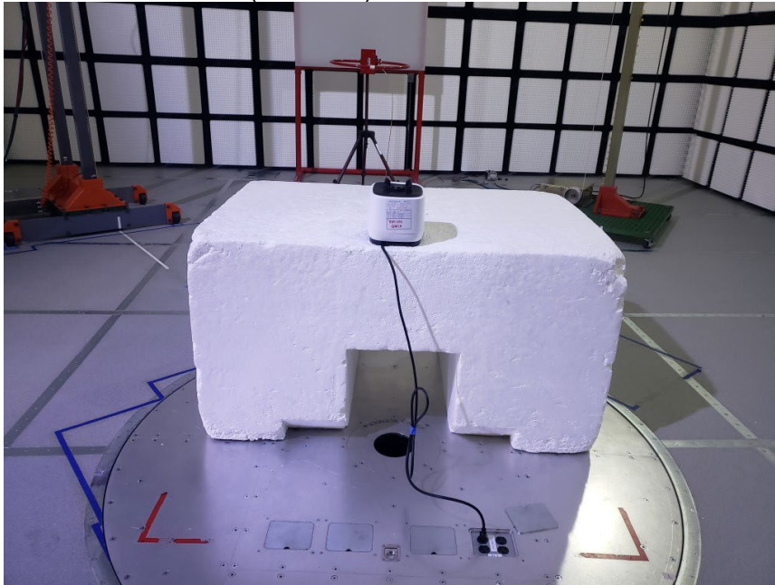
RADIATED PHOTO (<30 MHz) VM0232
