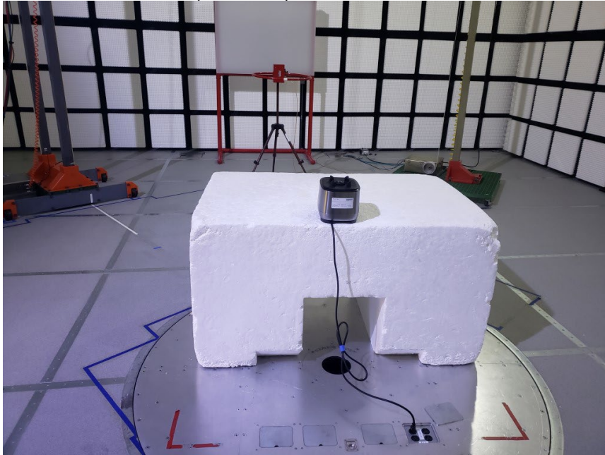
RADIATED PHOTO (<30 MHz) VM0234
