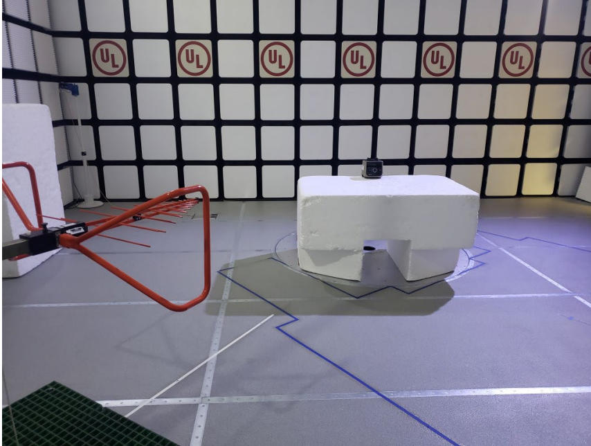
RADIATED PHOTO (30-1000 MHz) VM0231
