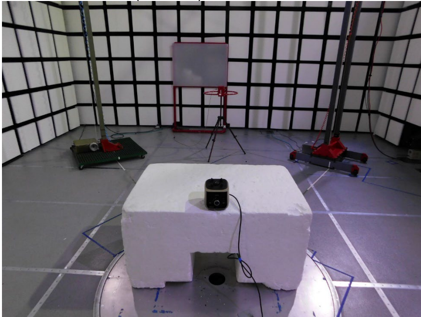
RADIATED PHOTO (<30 MHz) VM0231
