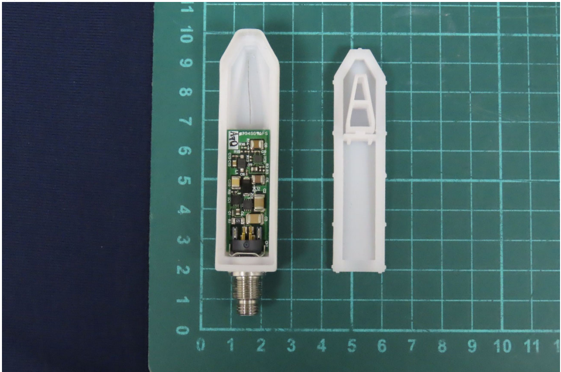
(1) EUT Photo
