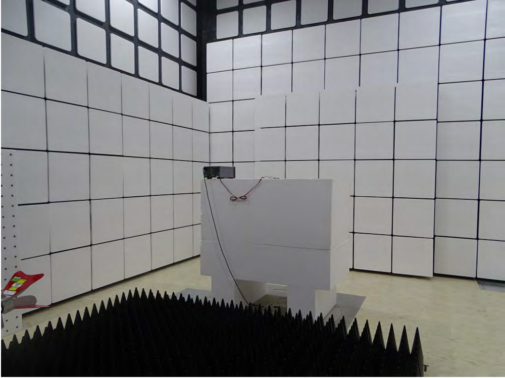
Radiated Test (Horn) - PCB Antenna
