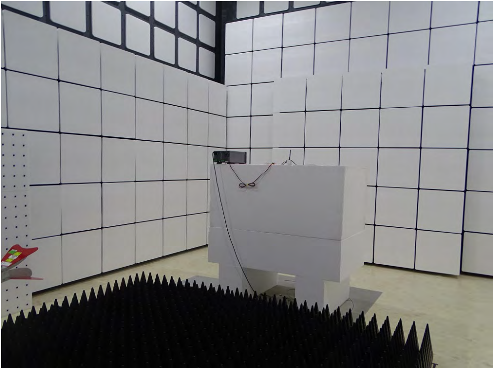
Radiated Test (Horn) - whip Antenna
