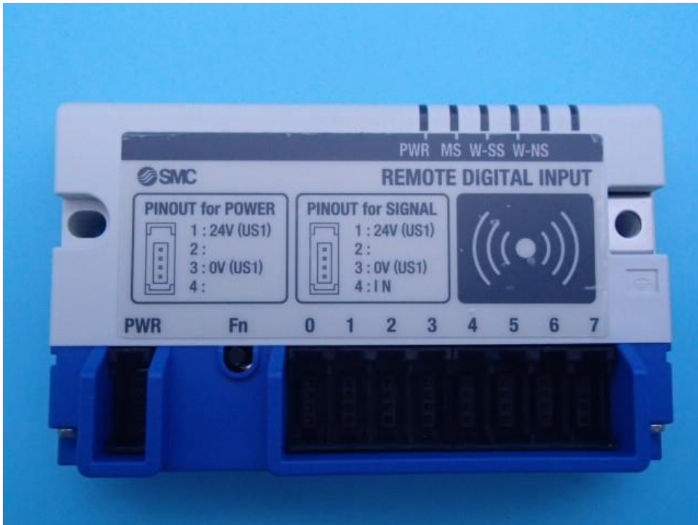
EX600-WDXE1 Front side
