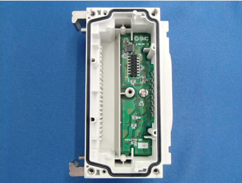
Ex600-WPN2 Inside view
