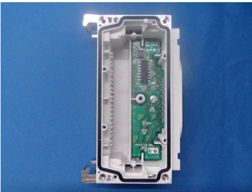
EX600-WSV4-X41 Inside view
