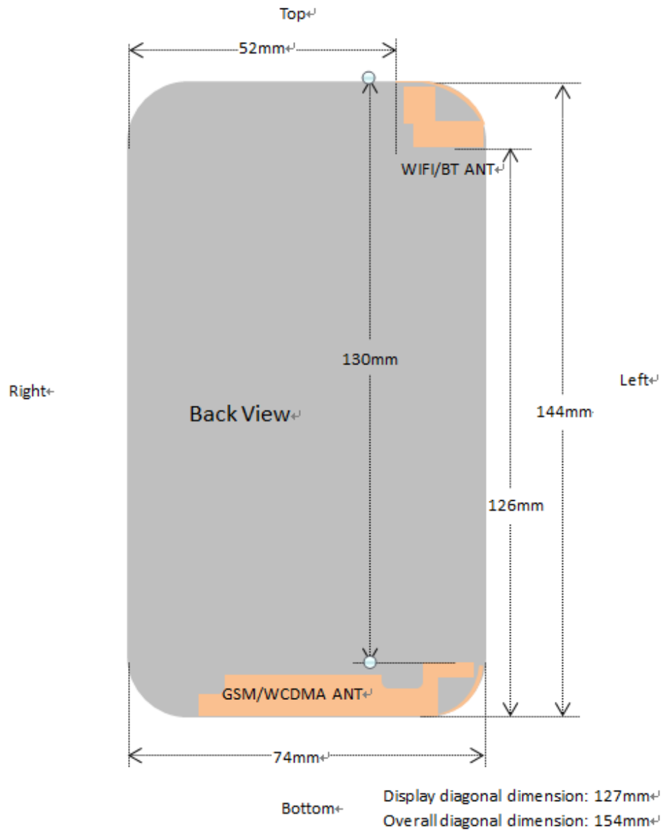
Fig.14.1 EUT Antenna Locations
