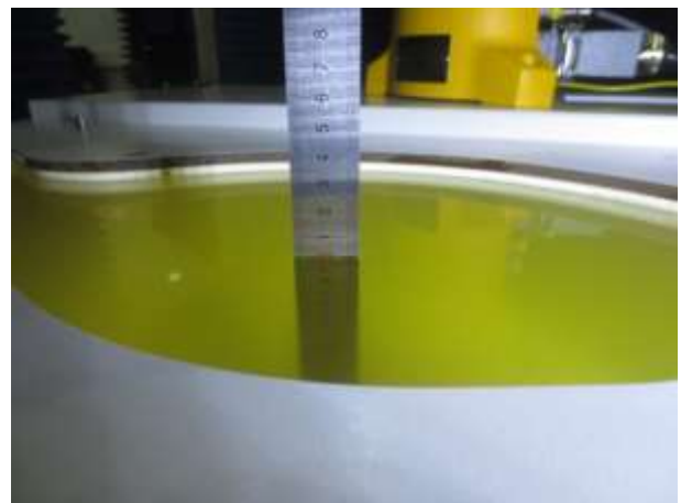
Fig. 9.6 Photo of Liquid Height for Body SAR
