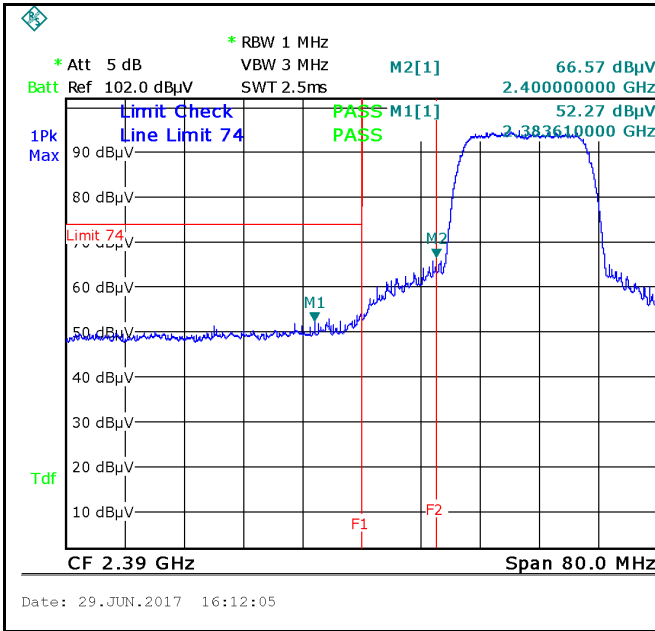
Band Edge, Left Side (Peak) - 802.11g Note: F1 is frequency 2390MHz
