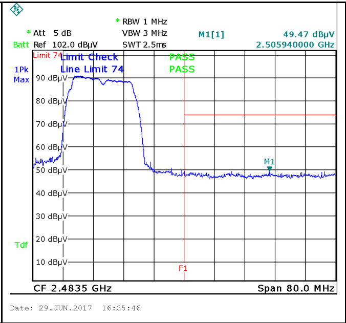
Band Edge, Right Side (Peak) - 802.11g Note: F1 is frequency 2483.5MHz
